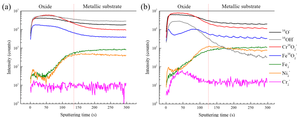
Fig.V-3 ToF-SIMS depth profiles for passive film formed on 304L SS surface in 0.05M \text{H}_2\text{SO}_4(\text{aq}) at 0.4V/SCE for 1h at (a) room temperature, and (b) after heat treatment in vacuum (UHV) at 300°C (the position of the oxide/metal interface is determined by the maximum intensity of \text{Ni}_2^- in the depth profile)
