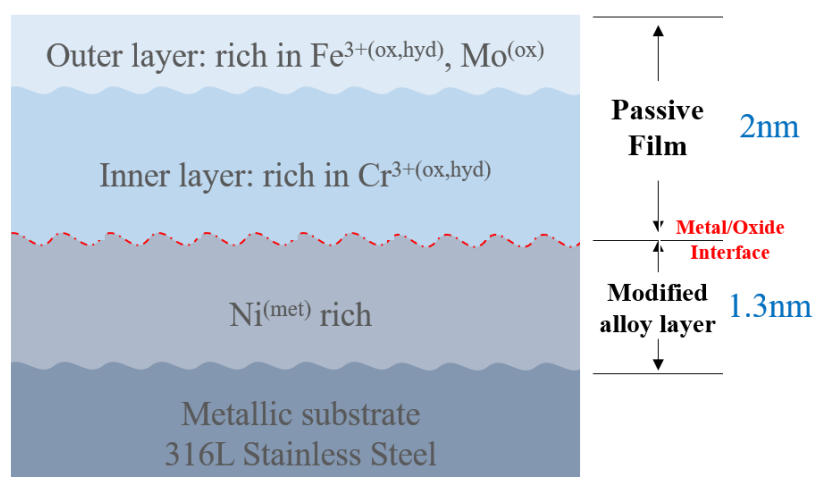
Fig.IV-3 The model for the passive film formed on 316L SS surface in 0.05M H 2 SO 4 (aq) at 0.4V/SCE for 1h
