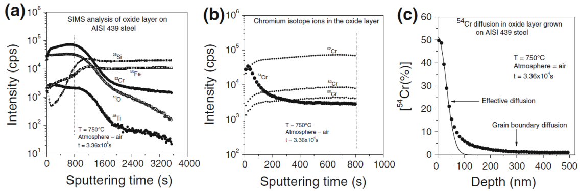
Fig.I-12 SIMS depth profiles of the oxide layer grown on the AISI 439 stainless steel after ^{54}\text{Cr} diffusion at 750°C [272]
