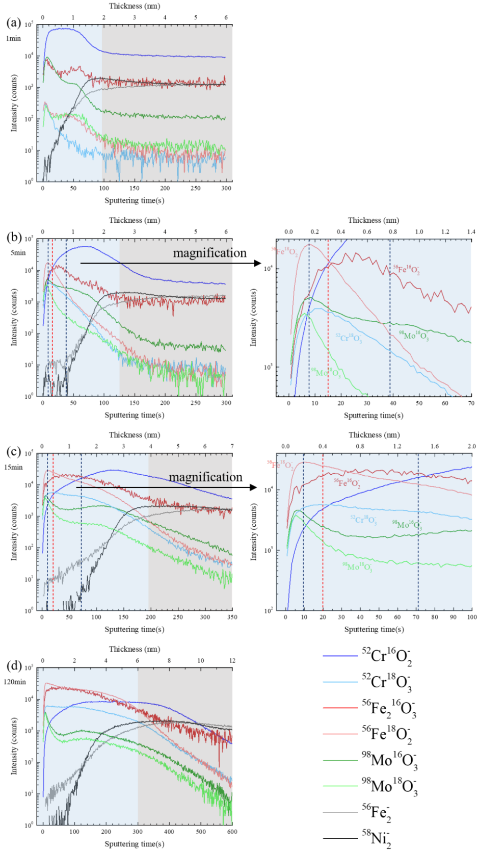
Fig.VI-4 ToF-SIMS profiles obtained on the passive film formed on 316L SS surface after re-oxidation at 300°C for (a) 1 min, (b) 5 min, (c) 15min and (d) 2 h. (The intensity of ^{56}\text{Fe}_2^{16}\text{O}_3^- signal is multiplied by 70)
