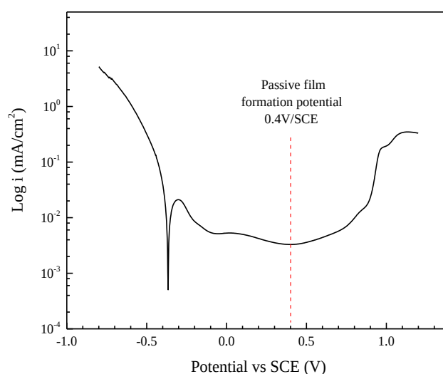
Fig.V-2 Polarization curve of the 304L SS in 0.05M H 2 SO 4 with a scan rate of 1mV/s
