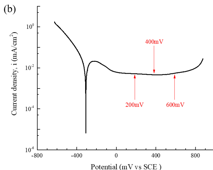
Fig.III-4 (a) Open circuit potential evolution for the CoCrFeMnNi HEA with a native oxide film in 0.05M H 2 SO 4 and (b) Potentiodynamic polarization curve of the CoCrFeMnNi HEA in 0.05M H 2 SO 4 (scan rate of 1mV/s)
