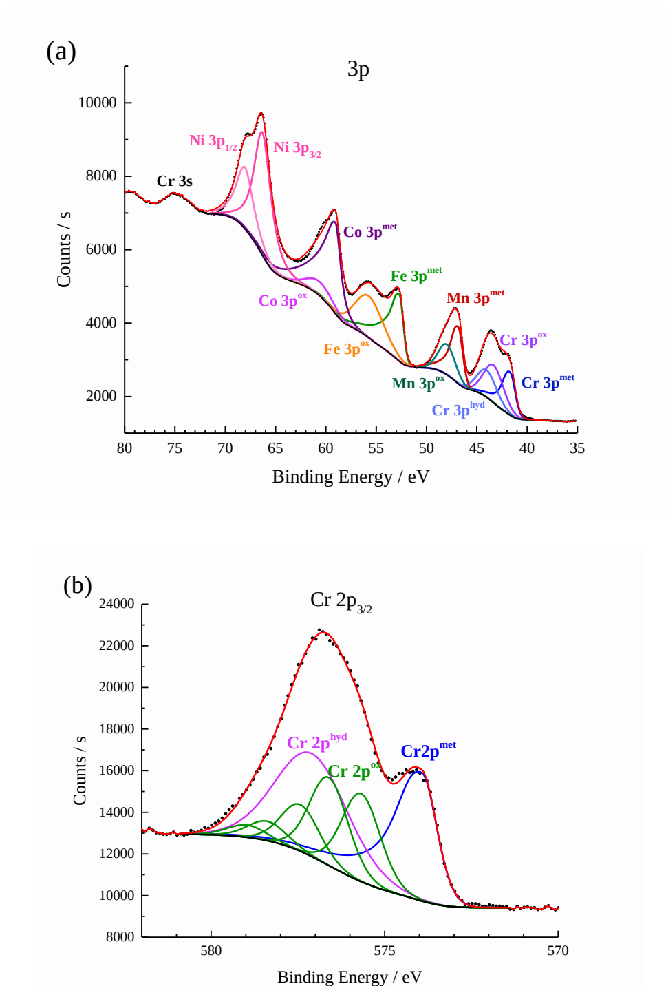
Fig.III-2 XPS core level spectra for the native oxide film formed on the HEA:(a) Cr 3p, Mn 3p, Fe 3p, Co 3p, Ni 3p and (b) Cr 2p 3/2 . The black dots represent the experimental spectra and the colored lines show the peak fitting.
