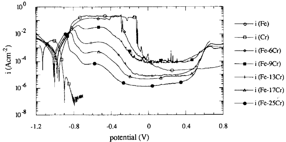
Fig.I-6 The polarization curves of iron, chromium, Fe-x%Cr (x=6, 9, 13, 17, 25) in 0.5M \text{H}_2\text{SO}_4 [131]
