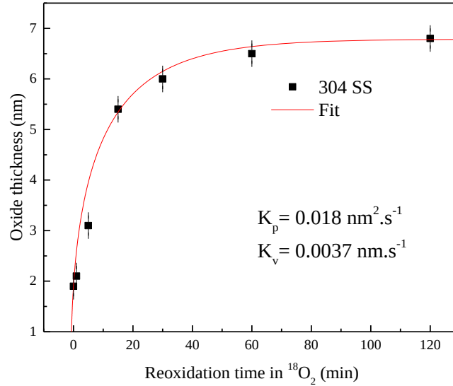
Fig.V-6 Oxidation kinetics of 304L SS at 300°C. Fit of kinetics by Eq.1 (solid line)
