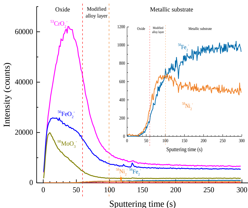
Fig.IV-2 ToF-SIMS depth profiles of the passive film formed on 316L SS surface in 0.05M \text{H}_2\text{SO}_4 (aq) at 0.4V/SCE for 1h. The colour lines mark the limits between oxide film, modified alloy layer and metallic substrate region
