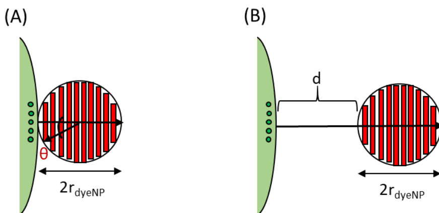
Figure 3.21: The dyeNP has been approximated to be consisted of multiple circular discs to take its large size into account. (A) dyeNP adsorbed directly on the surface of the microcavity, (B) dyeNP present at a surface-to-surface distance d from the microsphere.
