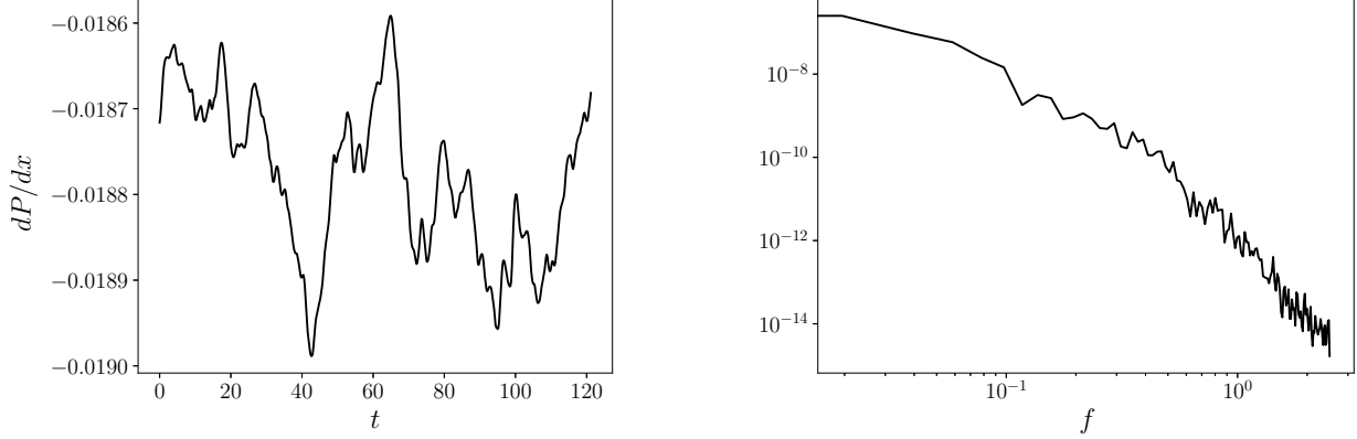
Figure 2.3: Time history (left) and PSD of the streamwise forcing, adapted to maintain a constant unitary non dimensional volume flow rate. The most prominent effect is given by the low frequency oscillations. Turbulent puff Re = 1500 .
