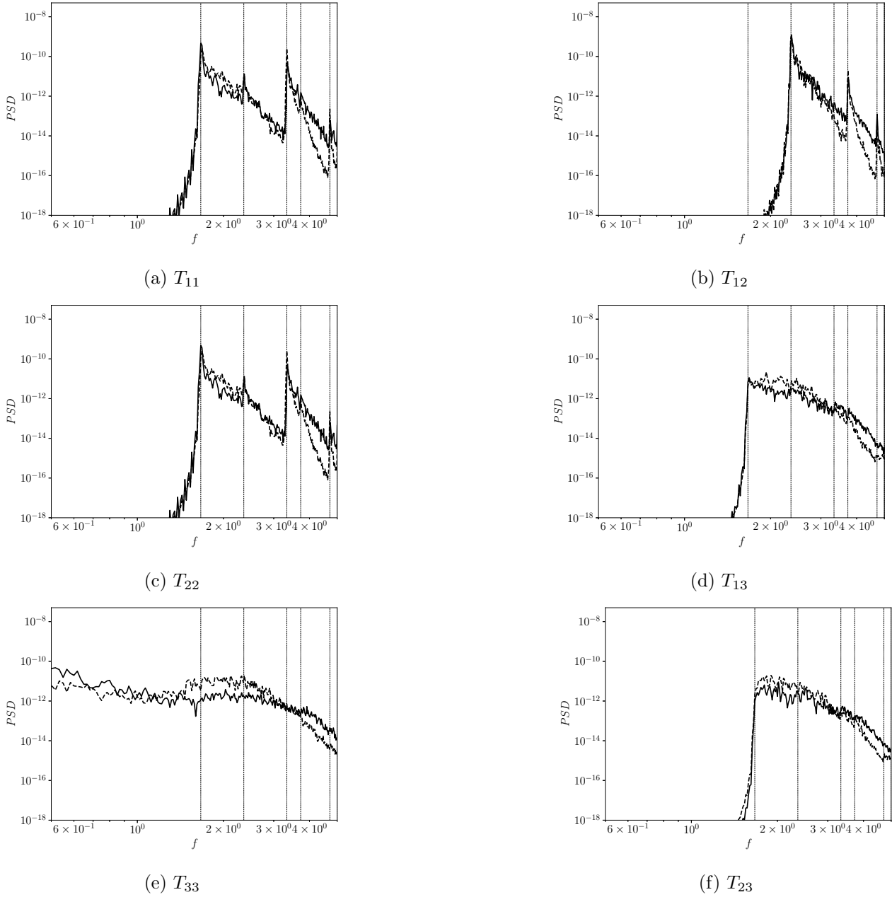
Figure 4.13: Pressure fluctuations PSD spectra for each component of the Lighthill tensor computed at x_3 = -150 (continuous) and x_3 = 150 (dashed), Ma = 0.3 . Turbulent puff in square duct, computed with the exact Green's function. The vertical lines indicate the cut-on frequencies for the (m, n) couples (1,0); (1,1); (2,0); (2,1); (2,2) in this order, from left to right
