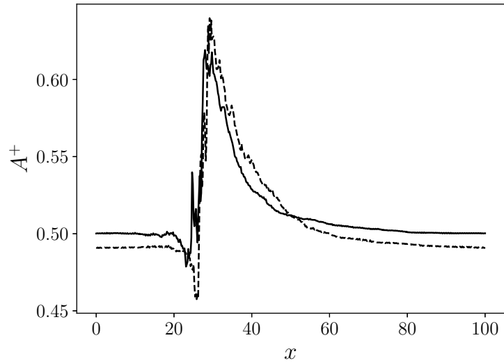
Figure 3.17: u > U_b area fraction for a puff at Re = 1600 in a bent duct at De = 30 (continuous line) and a straight duct ( De = 0 , dashed line).
