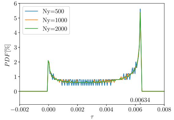
Figure 2.6: Viscous stress probability density function (PDF) and its convergence with varying number of grid points. Laminar flow in a square duct at Re = 1500
