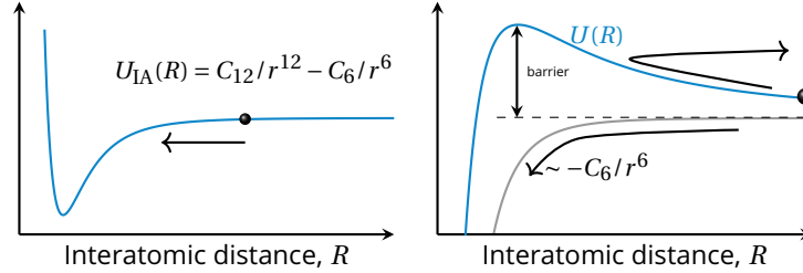
Figure 2.5: Left pannel : interatomic potential U_{IA}(R) as a function of R . This potential has bound states. Right pannel : an atom with l > 0 does not collide with another atom if its kinetic energy is lower than the centrifugal barrier.
