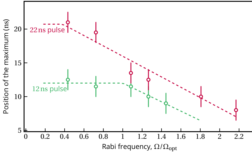
Figure 6.7: Measured maximum position of the photon emission for pulses of duration \tau_{opt} and 22ns as a function of the Rabi frequency of the driving pulse. Rabi frequencies are normalized by the value \Omega_{opt} found with a fit of the data.
