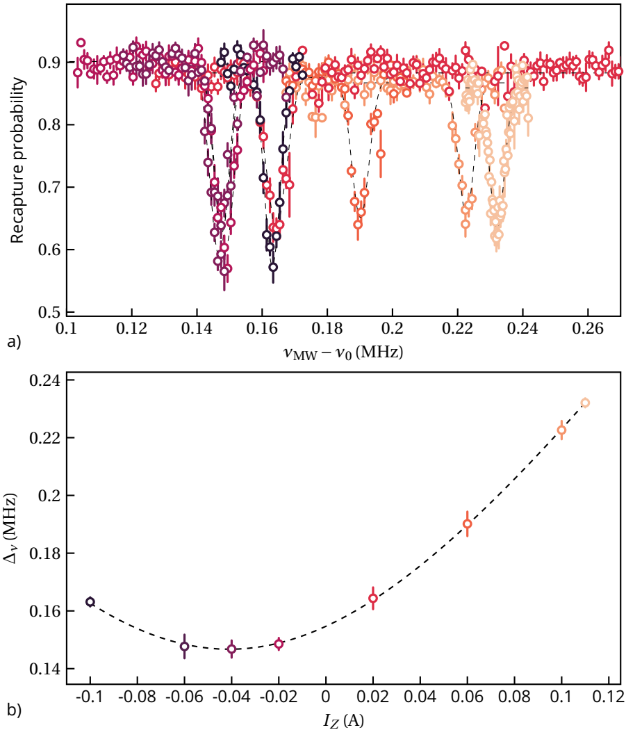
Figure 2.24: a) Loss spectra for different values of the bias field along \mathbf{z} , with lorentzian fits (dashed lines). b) Shift of the resonance frequency \Delta_\nu as a function of the current in the bias coil, with a parabolic fit (dashed line) to determine the minimum.
