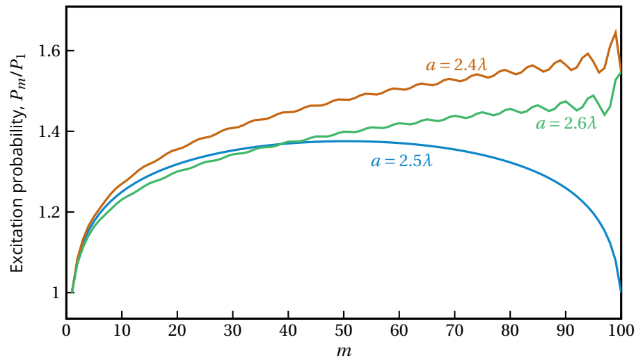
Figure 4.12: Probability of excitation of atom m divided by the single atom excitation probability for \delta = -1 and a = 2.5\lambda , a = 2.4\lambda and a = 2.6\lambda .
