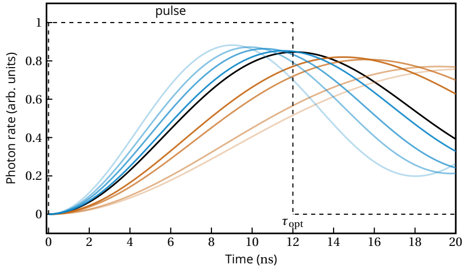
Figure 6.5: Calculated photon rates as a function of the time, for various Rabi frequencies around \Omega_{opt} . The shortest pulse (duration \tau_{opt} = 12 ns) is shown with a dashed line.
