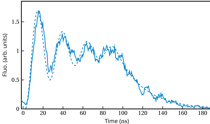
Figure 5.12: Fluorescence collected on an APD during resonant excitation of the cloud. The signal is fitted using the Optical Bloch Equations (dashed line).
