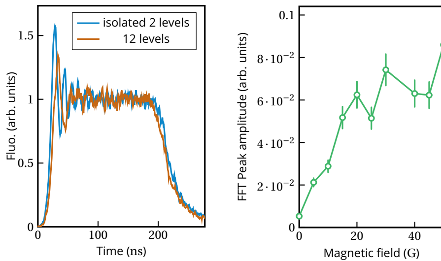
Figure 5.14: Left : Fluorescence collected on an APD during a resonant excitation of the cloud, using the two-level transition and without isolating the transition, using a 2 ns moving average. Right: FFT peak amplitude as a function of the magnetic field applied during the optical pumping. The error bars correspond to the uncertainty on the peak position.
