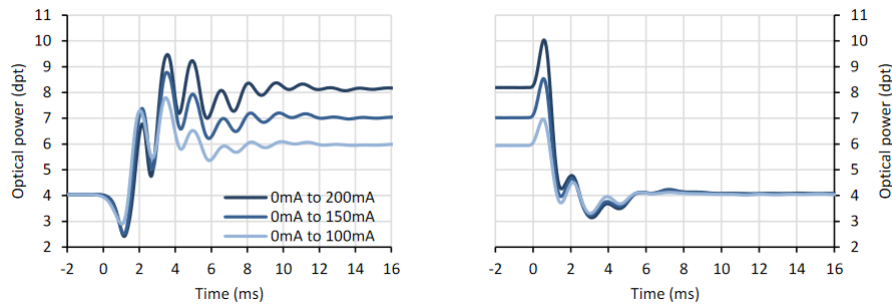
Figure 2.14: Typical optical response of the EL-10-30 a current step, from OptoTune® website.
