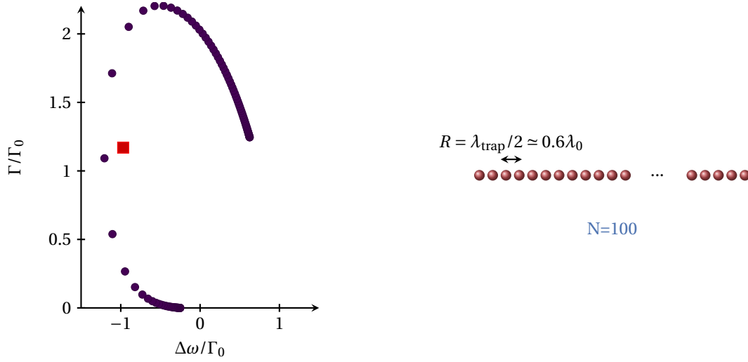
Figure 1.10: Collective decay and shift of a defect-free 1D chain of N = 100 atoms with interatomic distance 0.6\lambda_0 . The red square corresponds to the weighted average response (see text below).
