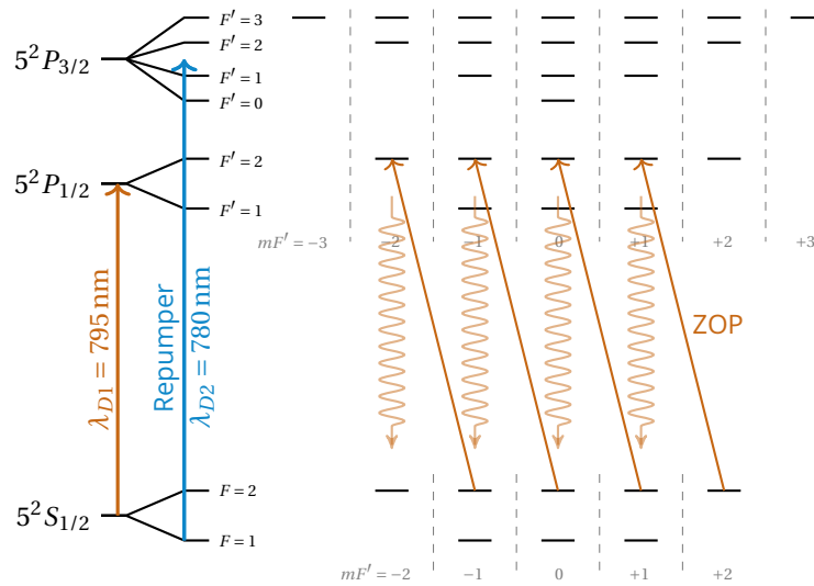
Figure 2.26: States and transitions used for the optical pumping to ( 5S_{1/2}, F = 2, m_F = -2 ). The solid arrows correspond to the stimulated \sigma_- transitions. The curved ones correspond to the other transitions. ZOP : Zeeman Optical Pumping
