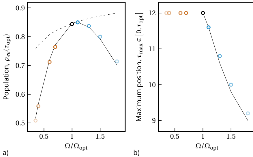
Figure 6.6: a) Population if the excited state at the end of the pulse as a function of the Rabi frequency. The maximum for any pulse duration is represented by the dashed line. b) Position of the maximum of the emission rate for t < \tau_{opt} as a function of the Rabi frequency. The colors are the same than in figure 6.5.
