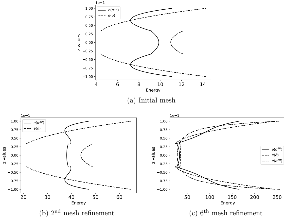
FIGURE 2.6 – Energy densities across the plate thickness computed for \boldsymbol{\sigma}^{3D} and \hat{\boldsymbol{\sigma}} at the plate edge for n = 3 . (Energy in "GPa", z in "cm").
