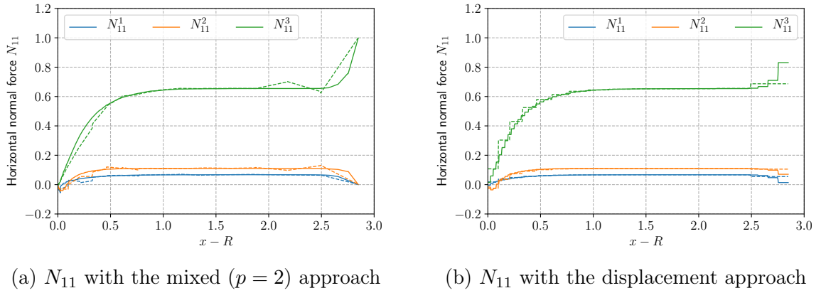
FIGURE 3.11 – Evolution of N_{11} along the plate length for a coarse (dotted line) and a fine (solid line) mesh
