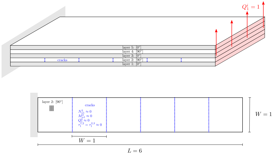
FIGURE 3.12 – cracked plate problem
