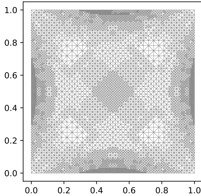
FIGURE 2.4 – Final refined meshes for the homogeneous plate for n = 1
