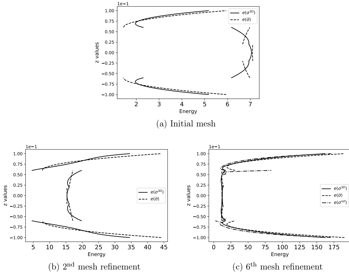
FIGURE 2.14 – Energy densities across the plate thickness computed for \sigma^{3D} , \hat{\sigma} and \sigma^{ref} at the plate edge for n = 5 . (Energy in "GPa", z in "cm").
