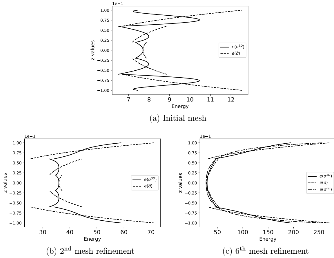
FIGURE 2.8 – Energy densities across the plate thickness computed for \sigma^{3D} , \hat{\sigma} and \sigma^{ref} at the plate edge for n = 5 . (Energy in "GPa", z in "cm").
