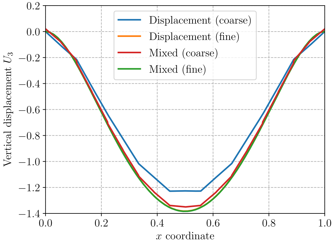
FIGURE 3.7 – Vertical deflection U_3 for the thin plate case (both solutions in the fine mesh case are superimposed)
