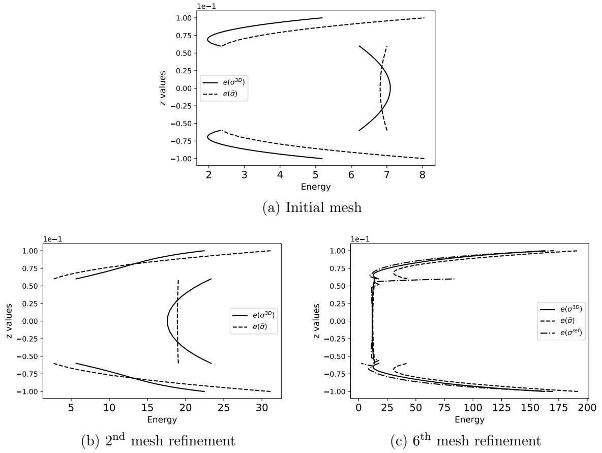
FIGURE 2.13 – Energy densities across the plate thickness computed for \sigma^{3D} and \hat{\sigma} at the plate edge for n = 3 . (Energy in "GPa", z in "cm").
