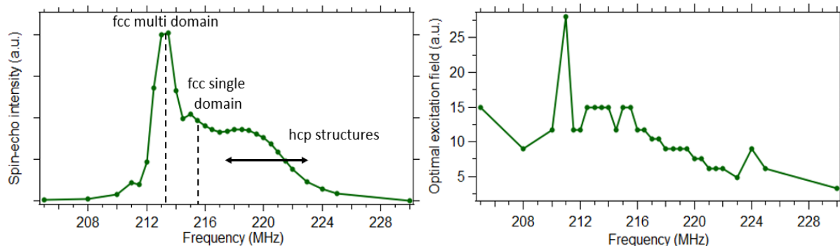
Figure 4: ^{59}\text{Co} IF NMR analysis of a CoO/Co OMG powder sample containing Co particles of various sizes. Left: Optimal spectrum, right: Optimal Power. Different peaks can be distinguished, giving information about the crystalline ( fcc or hcp ) and magnetic structure (single- or multi-domain) of the cobalt inside the sample.
