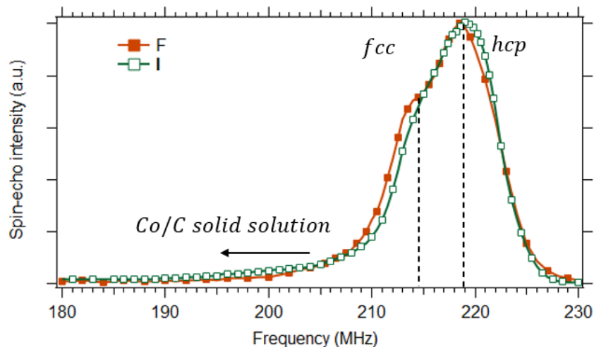
Figure 8: Comparison of the ^{59}\text{Co} IF NMR spectra of sample F : Activated for 15 h (WC balls, H_2 atmosphere) & milled for 48 h for CHG; with the one of sample I : Activated for 12 h ( ZrO_2 balls, H_2 atmosphere), without any milling for CHG. The lines and arrows indicate the different Co environments.
