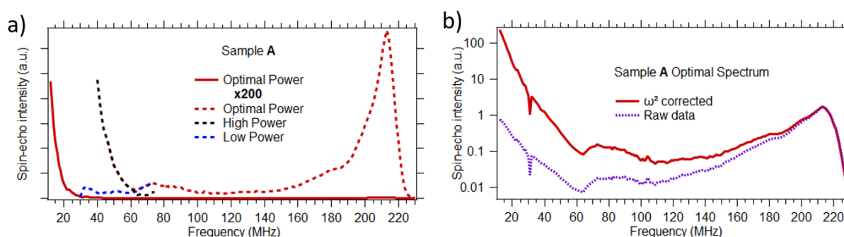
Figure 10: a) 59 Co IF NMR analysis of sample A: Optimal spectrum from 12 – 230 MHz (solid red line). The dotted red line corresponds to the high-frequency region multiplied by 200. The blue and black dotted lines correspond to the signal obtained using a low and a high pulse power respectively, and multiplied by 200. The low and high powers are chosen to be equal to the one given the strongest signal at 75 MHz and 12 MHz, respectively. b) Optimal spectra of sample A over the whole frequency range using a log scale for the y-axis. The red line corresponds to the signal intensity after \omega^2 correction and the purple one to the raw data without this correction.
