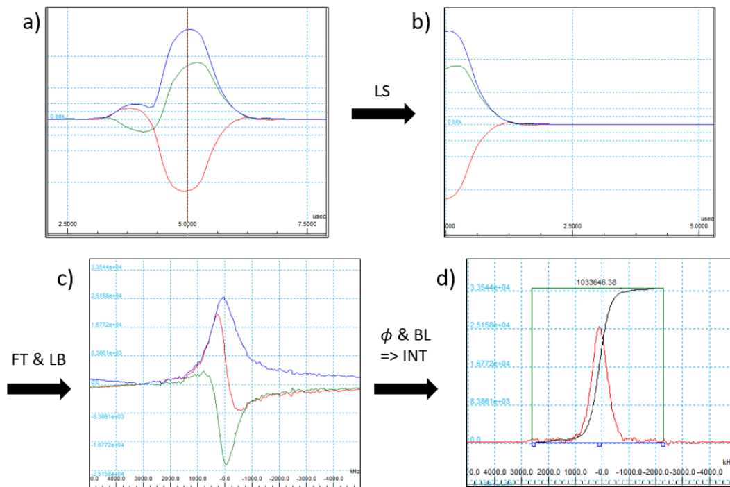
Figure 5: Typical data treatment procedure for the point-by-point spectrum acquisition using a spin-echo sequence. The signal was obtained from a CoO/Co sample at 213 MHz Red line: real part, green line: imaginary part, blue line: magnitude of the signal. Top left: the detected echo signal. LS: Left shift, FT: Fourier transformation, LB: line broadening, \phi : phasing, BL: baseline correction, INT: integration.
