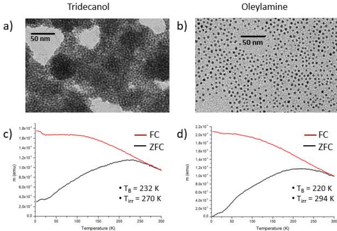
Figure 8: TEM and ZFC/FC magnetometry analysis of the NP_{4nm} samples with two different ligands. Top: TEM images. a) Tridecanol as ligand => Small interparticle distance. Particle size d = 4.4 \pm 0.4 nm. b) OAm as ligand => Large interparticle distance. Particle size d = 4.5 \pm 0.5 nm. Bottom: ZFC/FC magnetometry with the corresponding blocking ( T_B ) and irreversibility ( T_{irr} ) temperature of the sample with c) Tridecanol and d) OAm as ligand.
