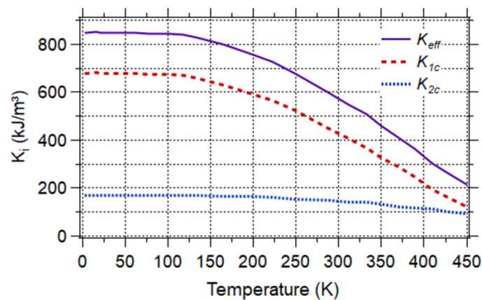
Figure 6: Evolution of K_{eff}(T) = K_{c1}(T) + K_{c2}(T) with temperature for hcp Co particle. Data taken from [29], [30]
