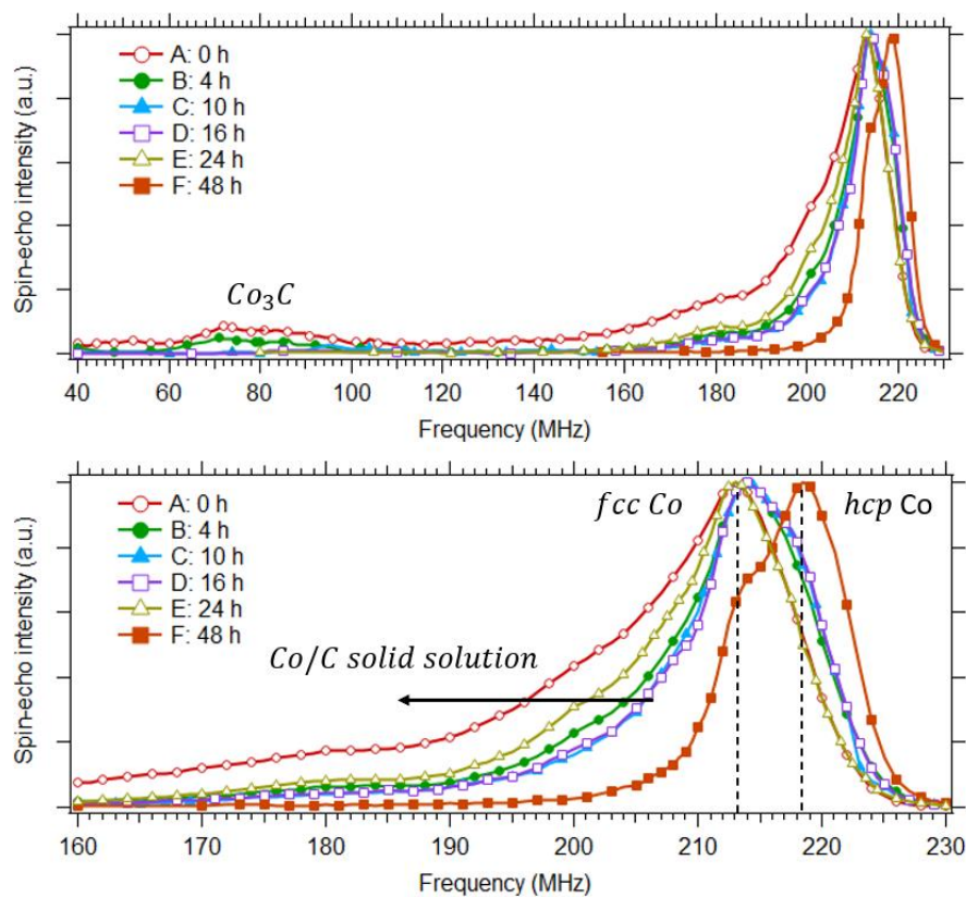
Figure 6: ^{59}\text{Co} IF NMR spectra of the samples A, B, C, D, E & F, milled for 0, 4, 10, 16, 24 & 48 h after activation, respectively. In the top spectrum, the region corresponding to \text{Co}_3\text{C} is highlighted. In the bottom a zoom of the spectra is shown, including indications of the different Co environments.
