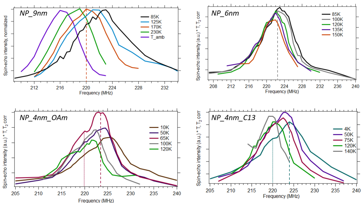
Figure 9: ^{59}\text{Co} IF NMR spectra taken at different temperatures of the four Co NPs samples presented in this work. Except for the NP_9nm sample, all spectra have been corrected for the Boltzmann distribution (multiplication by the temperature (K)) and the spin-spin relaxation (i.e., T_2 ) variation. The NP_9nm spectra have been normalized by their maximum. One or two main peaks can be differentiated in the spectra, indicated for one temperature for each sample as exemplification: dashed line = hcp Co, dotted line = fcc Co or hcp Co with defects, only differentiated for low temperature experiments.
