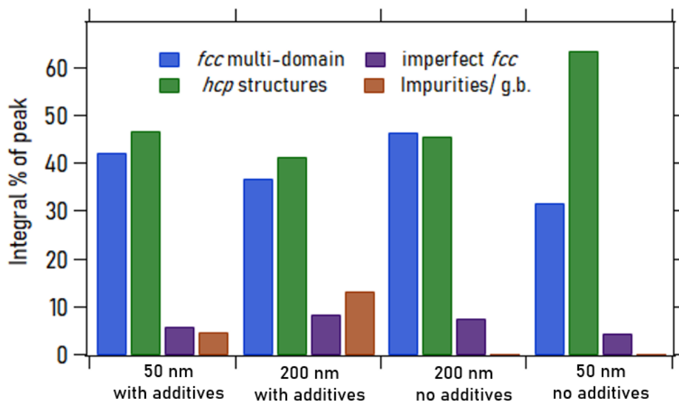
Figure 11: Quantitative distribution of the different crystalline/ magnetic phases detected by ^{59}\text{Co} IF NMR for the samples presented in this work. The corresponding spectra are shown in Figure 5 and Figure 10 .
