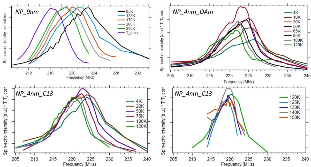
Figure 17: ^{59}\text{Co} IF NMR spectra at all the different tested temperatures of three Co NPs samples presented in this chapter. Except for the NP_9nm sample, all spectra have been corrected for the Boltzmann distribution (multiplication by the Temperature (K)) and the T_2 variation. The NP_9nm spectra have been normalized by their maximum.
