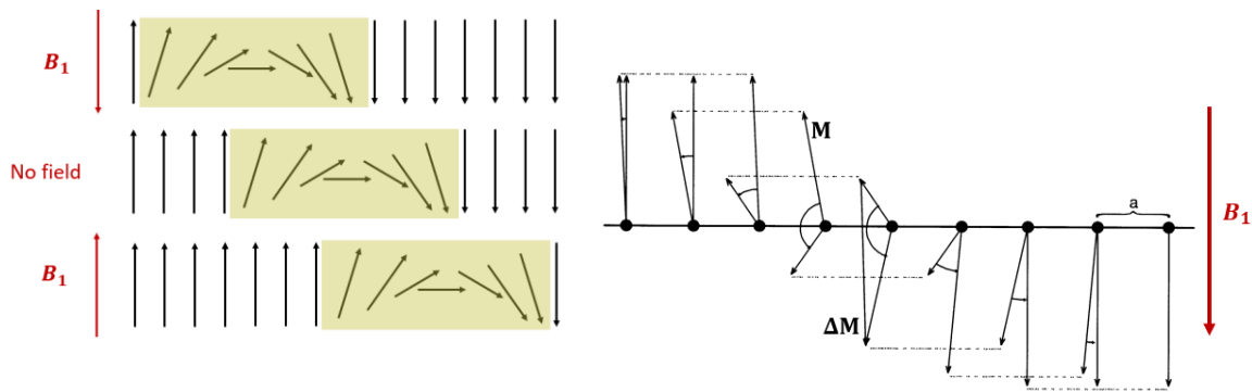
Figure 3: Left: Schematic representation of a 180° domain wall (light green background) and its displacement under the influence of an external magnetic field B_1 (static or rf ) in different direction. Right: Illustration of the rotation of the magnetic moments inside the domain (showing a local magnetization M ) and the resulting change of the local magnetization \Delta M (adapted from [3]). The domain walls illustrated here are Néel domain walls, but the mechanism is similar for different types of 180° walls (such as Bloch walls).
