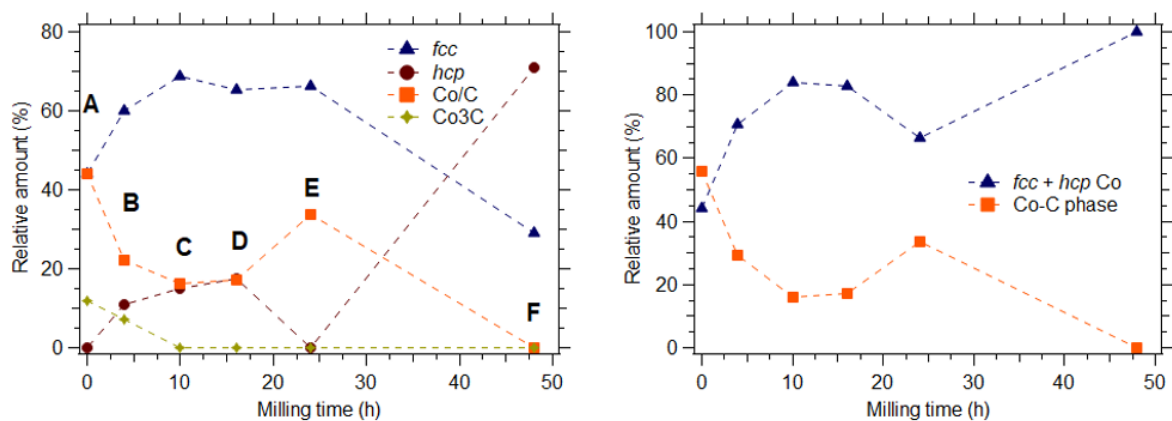
Figure 7: Left: Estimation from IF NMR of the different Co environments: pure fcc & hcp cobalt, \text{Co}/\text{C} solid solution (sum of the peaks of Co with 1-4 C NN), \text{Co}_3\text{C} . Right: Evolution of the total amount of pure Co ( hcp + fcc ) compared to \text{Co}-\text{C} intermediates ( \text{Co}/\text{C} + \text{Co}_3\text{C} ).
