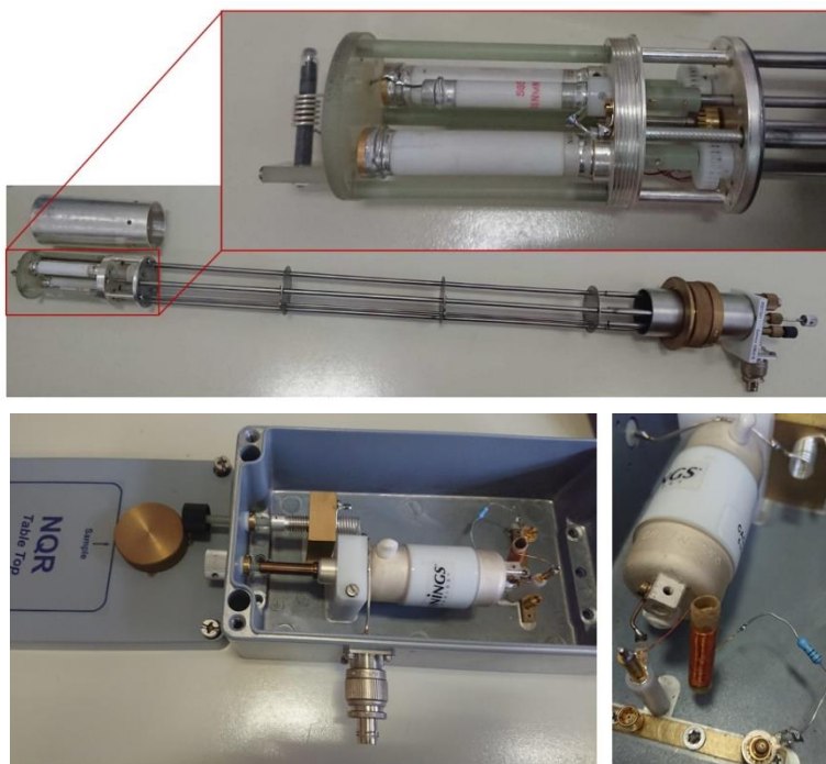
Figure 1: Pictures of two of the employed probes - Top: NMR-service low-temperature NMR/NQR probe, with a 5 mm coil. The sample is the black powder in the sealed glass tube. Bottom: NMR-service NQR tabletop probe, with a home-made 5 mm coil and a 15 \Omega resistance in the circuit.
