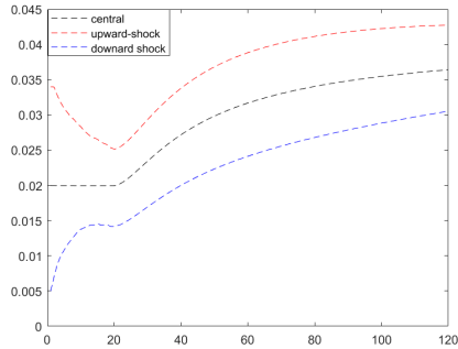
Figure 3.2 – Calibrated SW yield curve t \mapsto R(0, t) in central and shocked framework Figure 3.3 – Calibrated SW curve curve t \mapsto F(0, t) with T_\infty = 60 years
