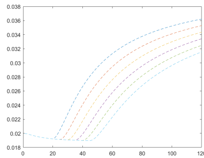
Figure 3.4 – Calibrated SW yield curve t \mapsto R(0, t) for different UFR values Figure 3.5 – Calibrated SW yield curve t \mapsto R(0, t) for different LLP values
