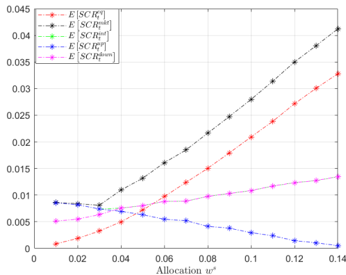
Figure 4.8 – Values of the SCR modules in function of the constant allocation weight w^S in equity for t = 0 .
