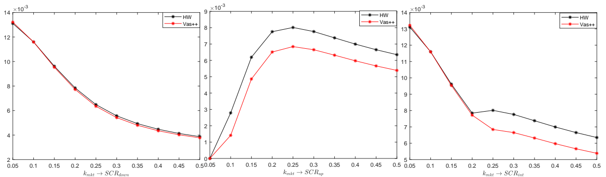
Figure 2.3 – SCR values with Vasicek++ and Hull and White models in function of k for SCR_{down} (left), SCR_{up} (middle) and SCR_{int} (right).
