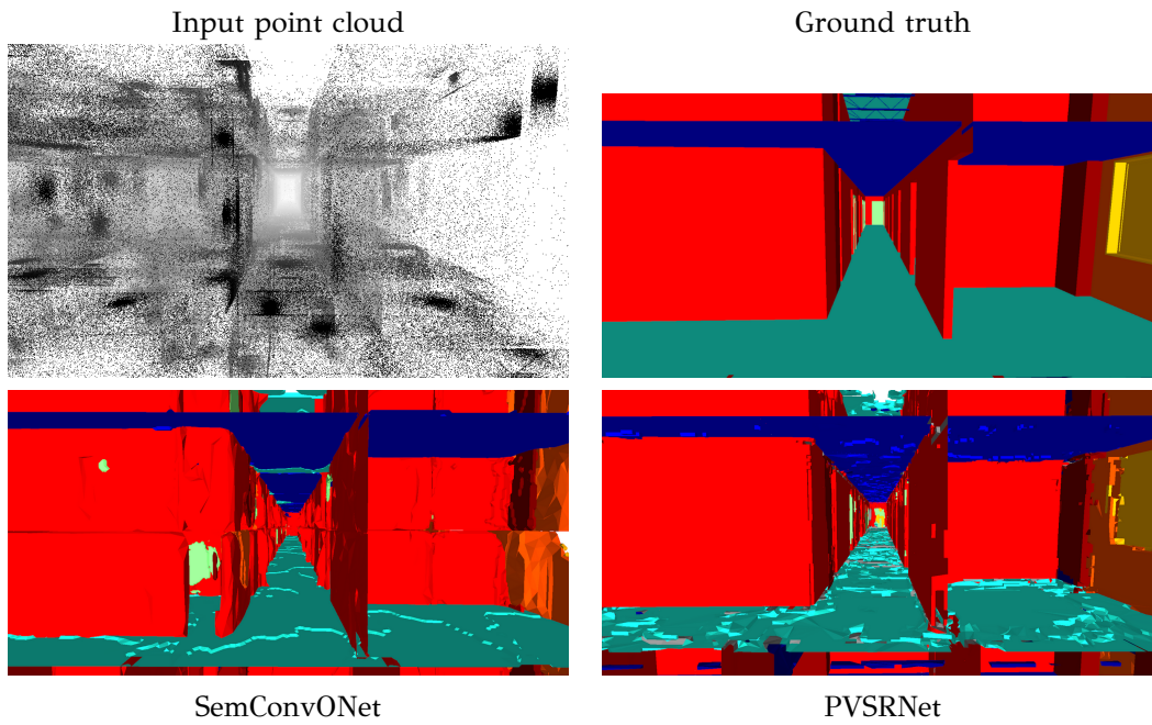
Figure 11.2: Qualitative results on the test set (NBU_MedicalClinic).
