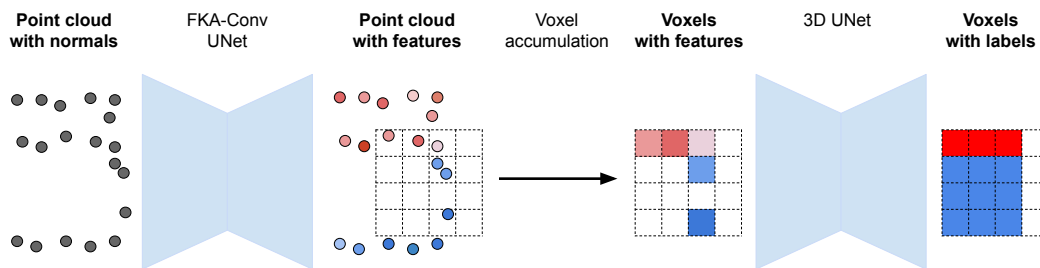
Figure 10.1: PVSRNet is composed of two networks, one operating on a raw point cloud for rich semantic feature extraction (FKACnv sub-network) and the second one on voxels for semantic volume occupancy (3D UNet).
