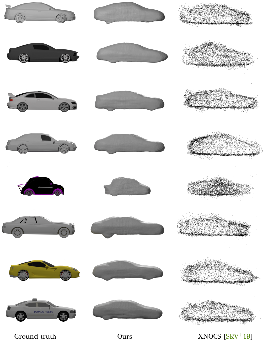
Figure 7-4: Qualitative results on the car category.
