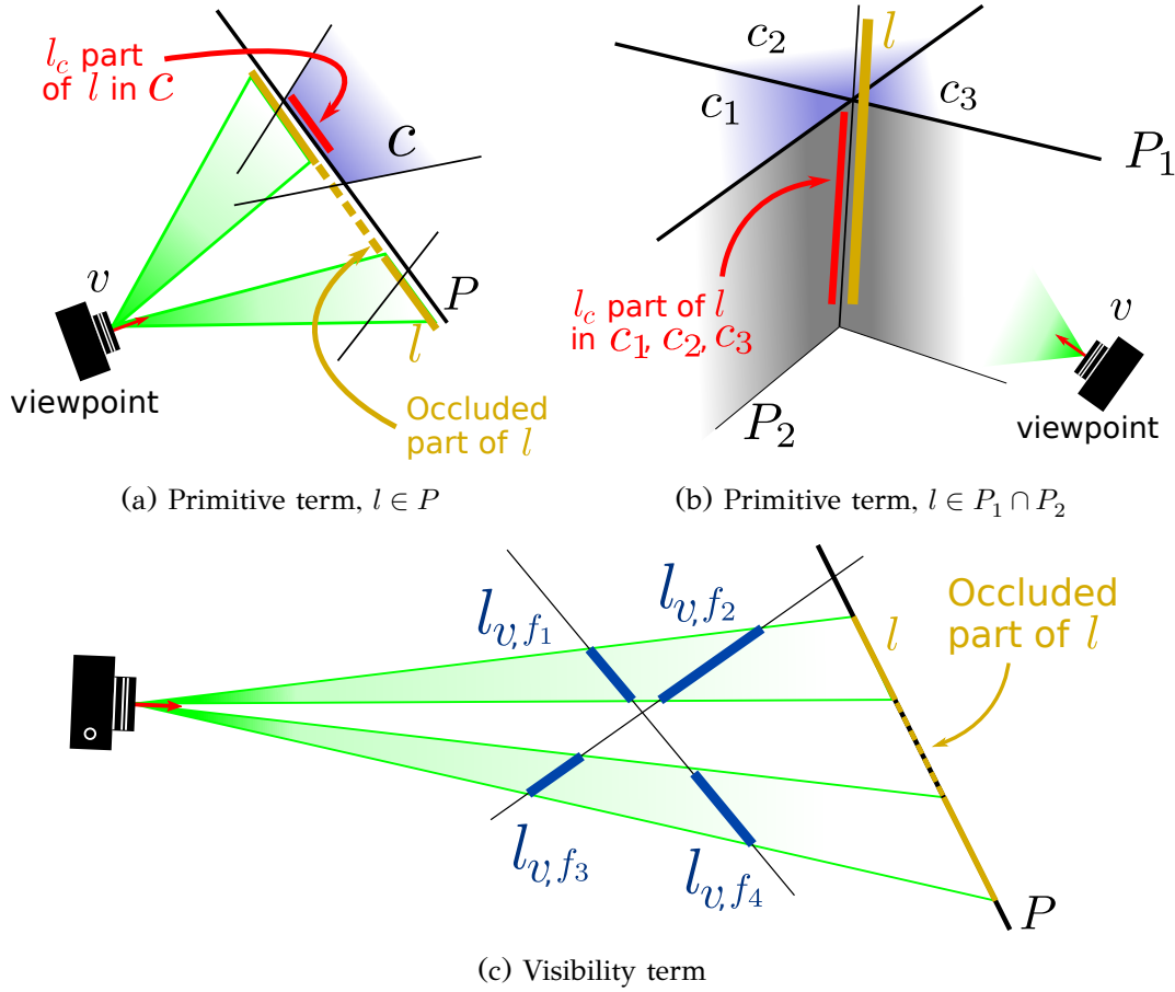
Figure 3.7: Primitive and visibility terms.
