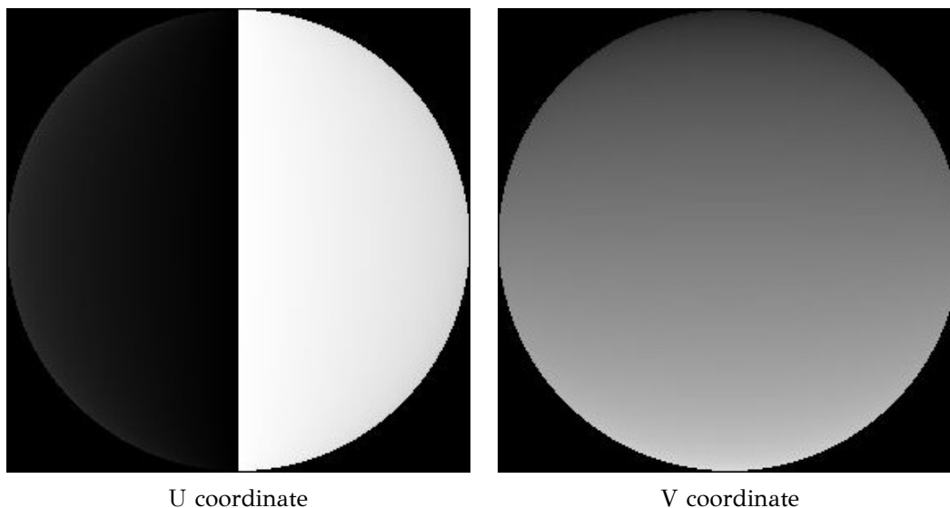
Figure 6.6: Rendering of the UV coordinates (Black: 0, White: 1) for a unit sphere
