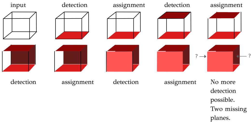
Figure 3.3: Because line segments are sparse, removing the inliers immediately after a plane detection leads to missing planes in the simple case of a cube whose detected lines are the edges (in red: the detected planes at each step).
