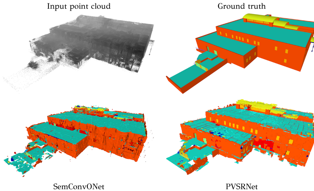
Figure 11.6: Qualitative results on the test set (NBU_MedicalClinic).
