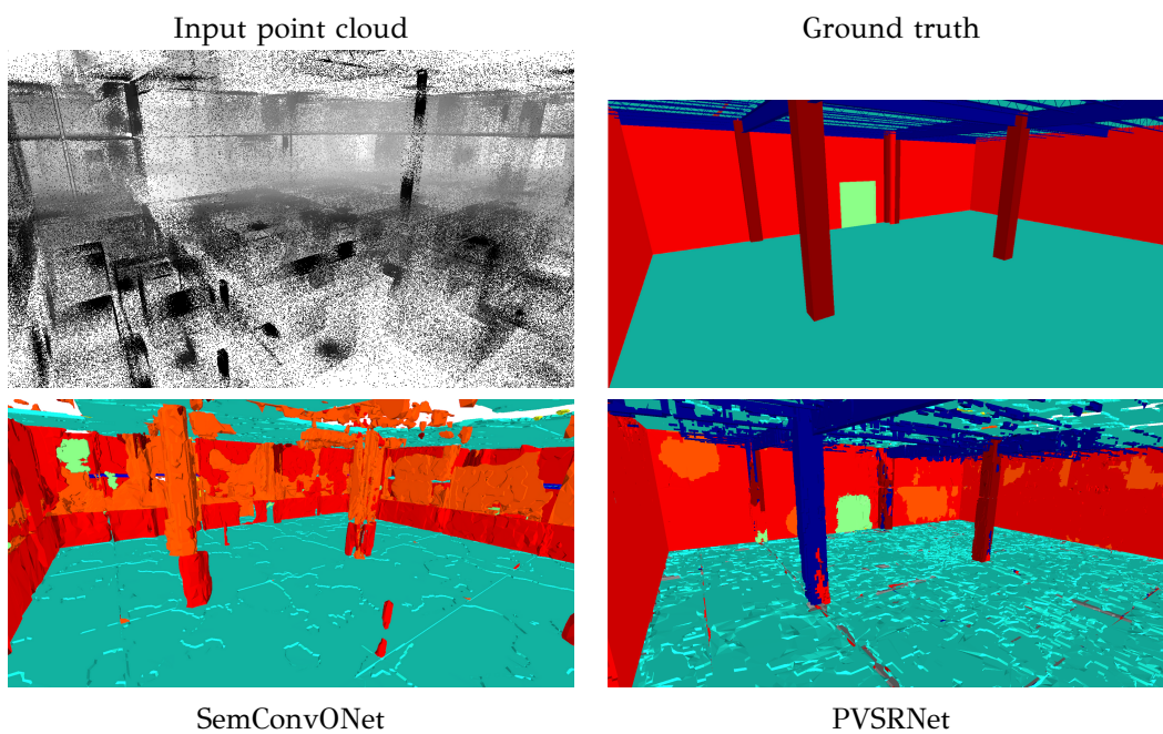
Figure 11.3: Qualitative results on the test set (NBU_MedicalClinic).
