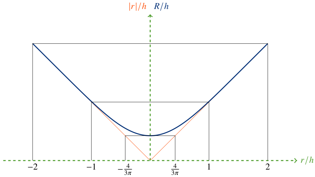
Figure D.23: Renormalisation factor in axisymmetric SPH ( R_a = \int_{\Omega_a} w|r|drdz ) against the radial direction.
