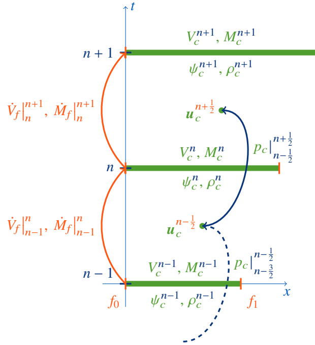
Figure C.1: Second-order in time time stepping for the finite volumes approach in ALE framework, variables localisation.
