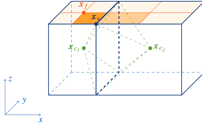
Figure 1.4: Labelling of information used for a mesh in code_saturne . In green, \mathbf{x}_{c_i} is the barycentre of one cell c_i whereas \mathbf{x}_{c_j} is the one of c_j . Each face f is split into portions of faces associated to a vertex. The portion of face f associated to a vertex v is drawn in solid orange, and is defined by \mathbf{x}_f , the barycentre of f , the middle of the two edges of f passing through vertex v , and \mathbf{x}_v itself.
