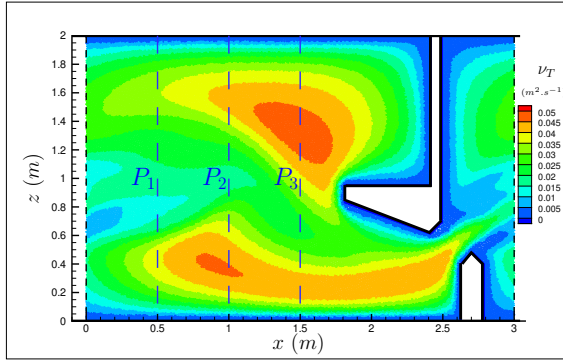
(c) Turbulent viscosity \nu_T field with SPARTACUS-2D .
