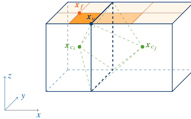
Figure 4.1: Labelling of information used for a mesh. In green, \mathbf{x}_{c_i} is the barycentre of one cell c_i whereas \mathbf{x}_{c_j} is the one of c_j . Each face f is split into portions of faces associated to a vertex. The portion of face f associated to a vertex v is drawn in solid orange, and is defined by \mathbf{x}_f , the barycentre of f , the middle of the two edges of f passing through vertex v and \mathbf{x}_v itself. The dual barycentric cell around a vertex v is defined by connecting surrounding cell centres, face centres and edge centres.
