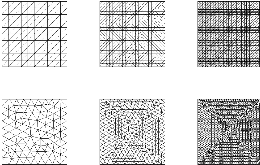
Figure D.7: Discretisations of the plane walls.
