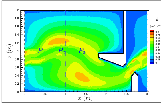
(e) Kinetic energy k field with SPARTACUS-2D .
