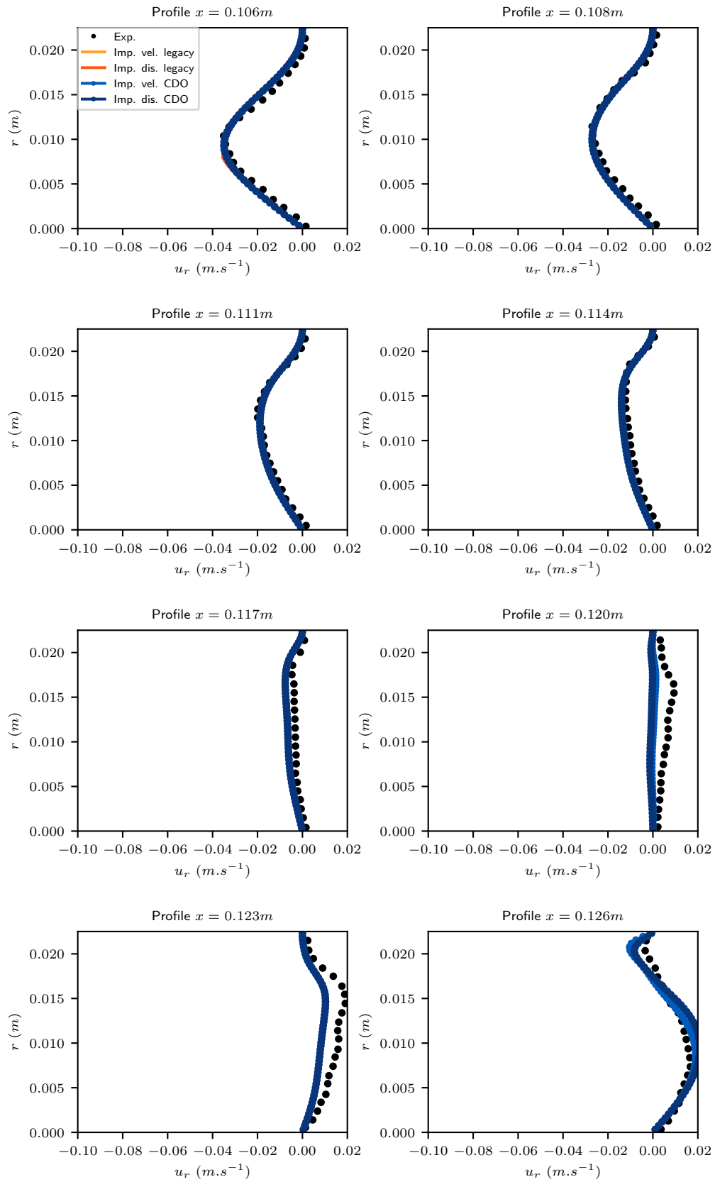
Figure 4.7: Radial velocity profiles at different positions x for the compression step ( x_p = 0.127 m ).
