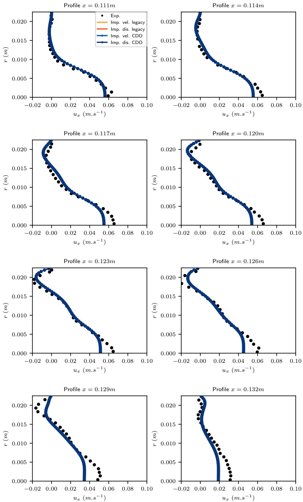
Figure 4.8: Axial velocity profiles at different positions x for the injection step ( x_p = 0.135 m).
