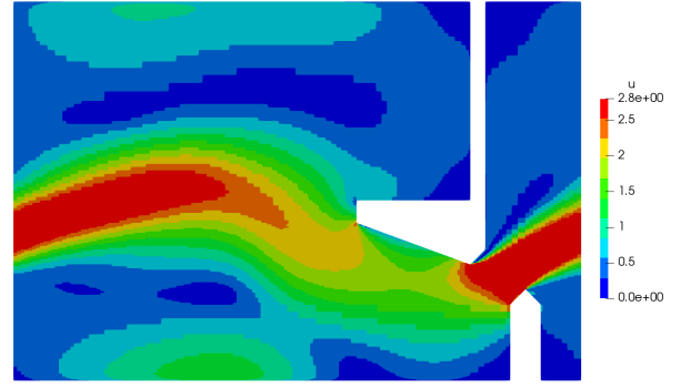
(b) Magnitude of the velocity field with code_saturne .
