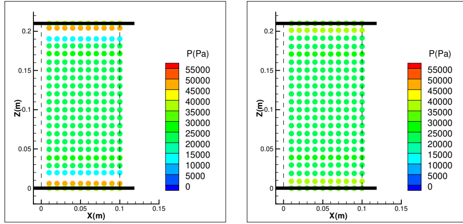
(a) Kulasegaram et al.'s gradient operator (2.17) is unable to maintain uniform pressure field. Particles move to a non-physical equilibrium. (b) The present gradient operator (2.23) is able to almost maintain uniform pressure field as an equilibrium.
