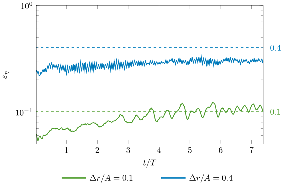
Figure 3.14: Errors on the free surface for simulations with an imposed velocity profile on the open boundaries for two particle spacings \Delta r . The dashed line shows the two values \Delta r/A .
