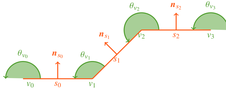
Figure 2.2: Boundary property definitions. Boundary with vertex semi particles v (in green) and with segments s which have a surface S_s and an inward normal \mathbf{n}_s .
