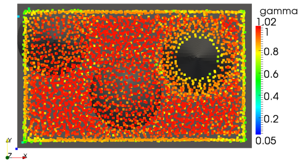
(a) Approximate \nabla\gamma_{as} , Equation (D.28)
