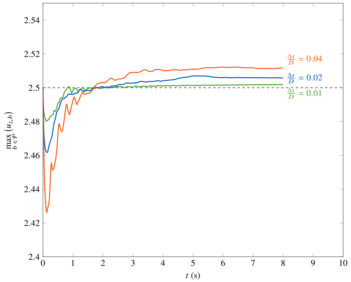
Figure D.27: Time evolution of the maximum velocity in the direction e_z .
