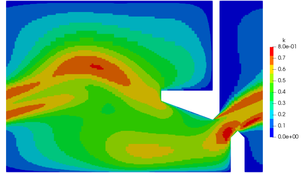
(f) Kinetic energy k field with code_saturne .
