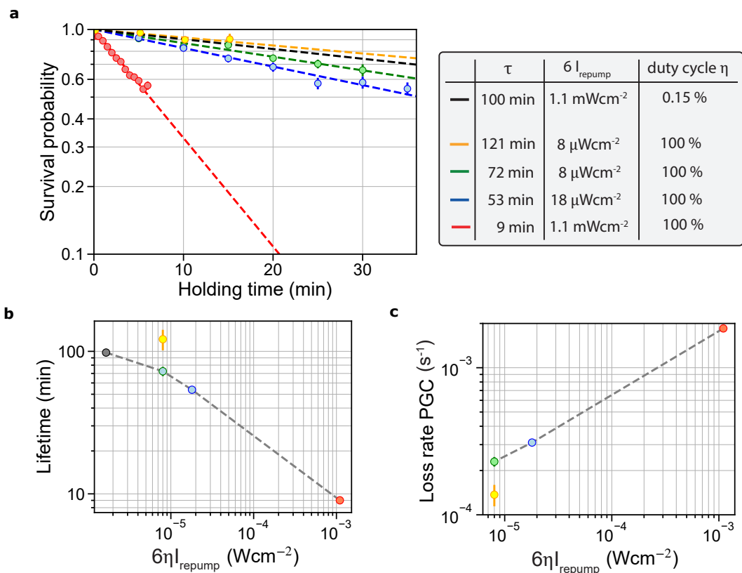
Figure 5.9: Influence of the Repump intensity on the lifetime a : Three different lifetime measurements with continuous PGC conditions on a 9 \times 9 array with open oven valve (red, blue, green), a measurement with continuous PGC condition on a 6 \times 6 array with closed oven valve and the black dotted line represents the measured lifetime of 100 min (pulsed PGC, closed valve). b : Demonstration of the extracted lifetime as a function of the repump intensity. c : Loss rate for the PGC beams, assuming that for the 100 min lifetime measurement in pulsed conditions, the losses are negligible.
