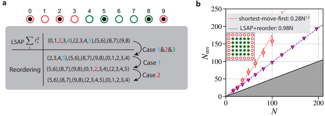
Figure 3.3: The LSAP2 algorithm. a Illustration of the different steps of the algorithm (see text). b : Comparison of the scaling of the number of moves N_{mv} with the number of target traps N for compact arrays (for exemplary array see inset), between the old shortest-move-first algorithm and the different steps of the LSAP2 algorithm. The black line indicates N/2 , the number of on average unoccupied target traps.
