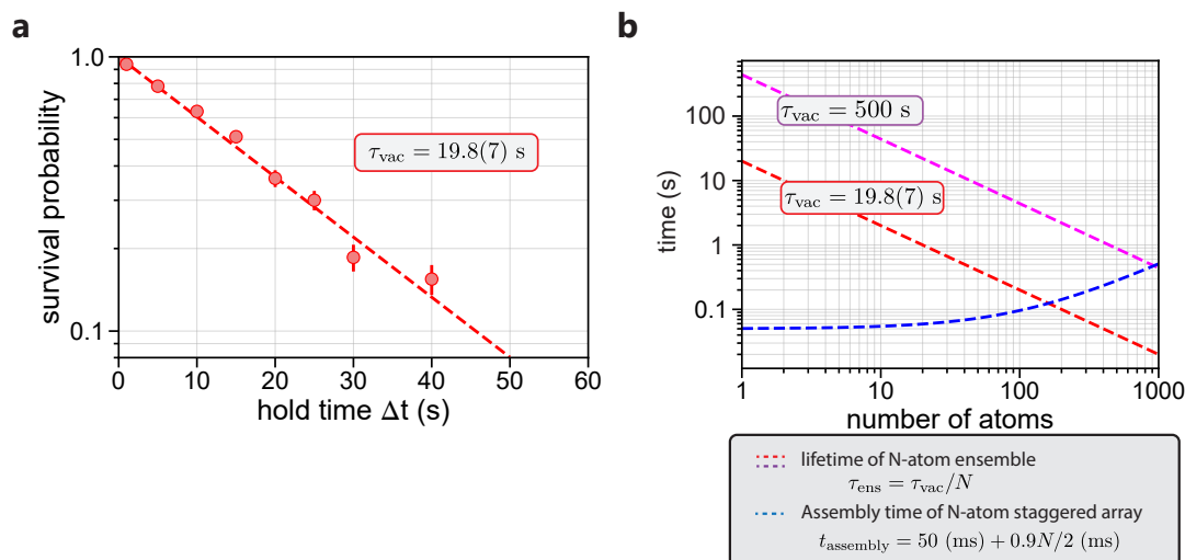
Figure 2.10: Lifetime of room-temperature setup a : Measurement of the vacuum lifetime \tau_{\text{vac}} b : Comparison of the N-atom lifetime and another experimental timescale, the assembly time of a N-atom staggered array.
