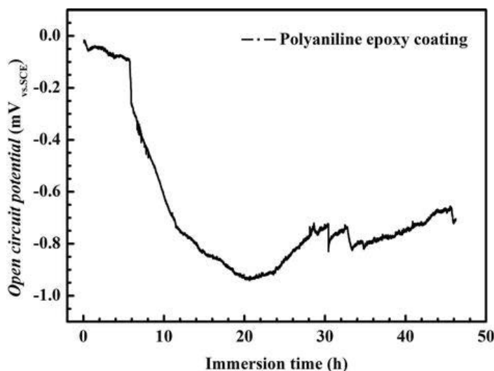
26 27 Figure 21: OCP curve for 2% PANI coated aluminium in 5% NaCl solution for 48h. Adapted from [102]
