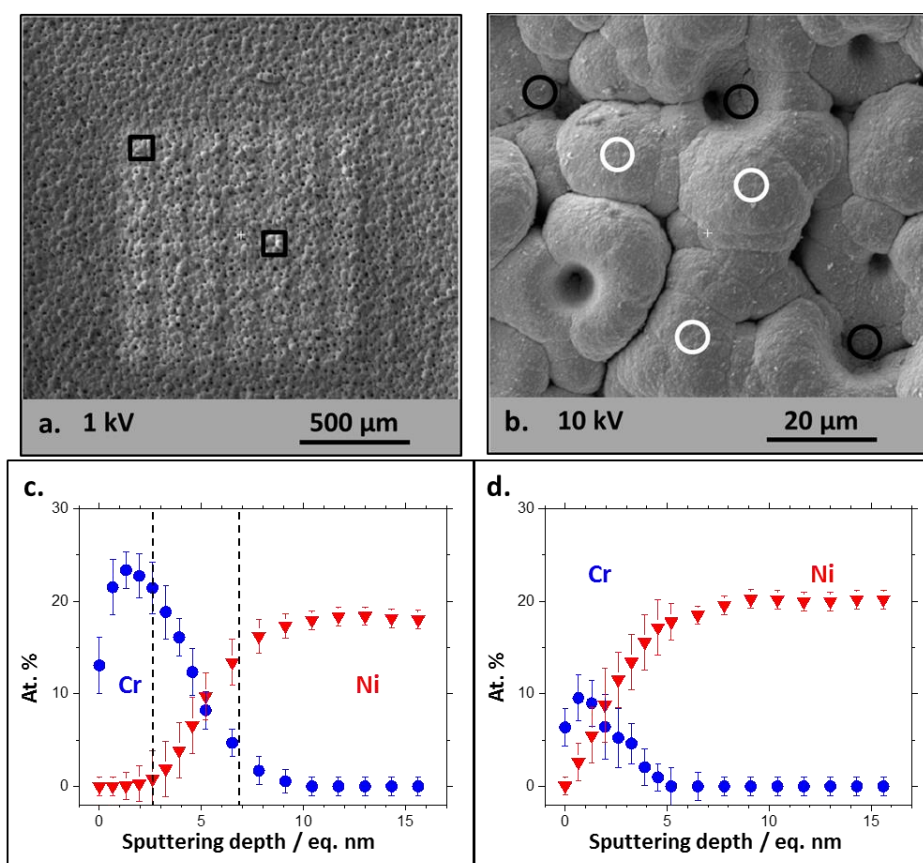
17 18 Figure 4.7: SEM images and Nano Auger elemental profiles in the vicinity of the sputtered area generated by ToF-SIMS. (a) 19 General view showing sputtered and non-sputtered zones, (b) magnification showing an example of the zone selected for AES 20 profiling inside the defect (valley-type zones are shown with black circles while hill-type are shown by white circles). (c) 21 Example of in-depth chemical profiling of chromium and nickel in the valley-type zones inside the crater, (d) Example of in-depth chemical 22 profiling of chromium and nickel on the hill-type zones of the crater.
