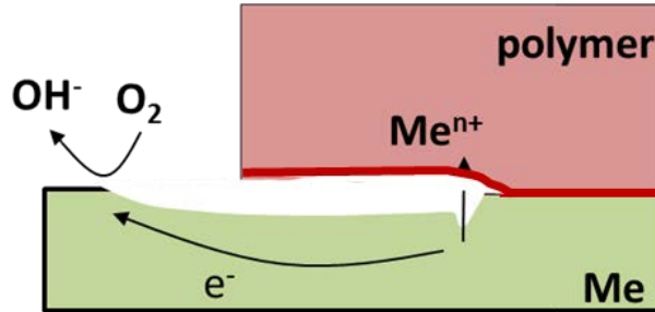
6 7 Figure 1.12: General scheme of anodic undermining mechanism
