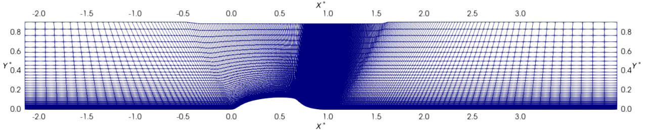
Figure 3.3: NASA hump mesh and geometry.
