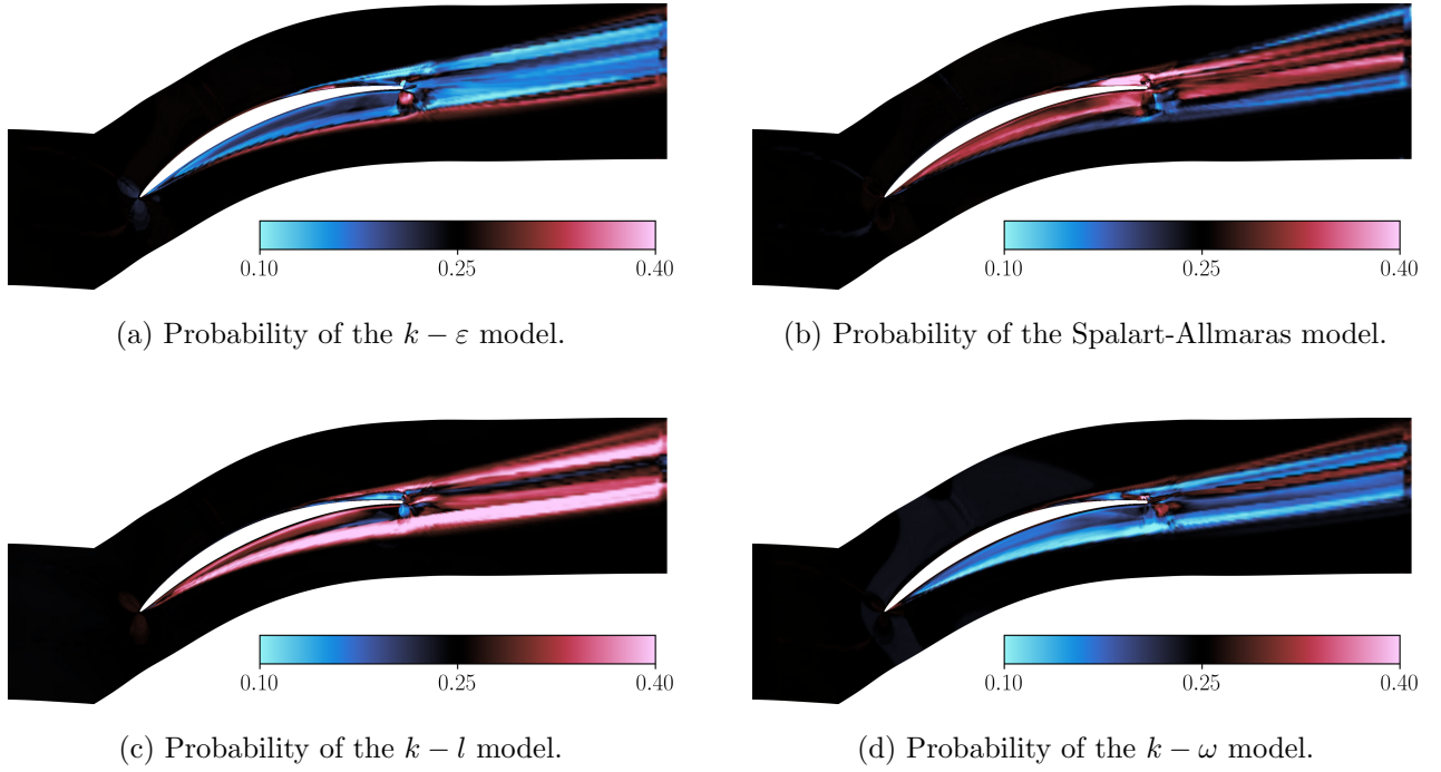
Figure 6.15: Probability of the four RANS models when only LES data are considered in the training. Training on \{S_2, S_3, S_4\} and prediction on S_1 .
