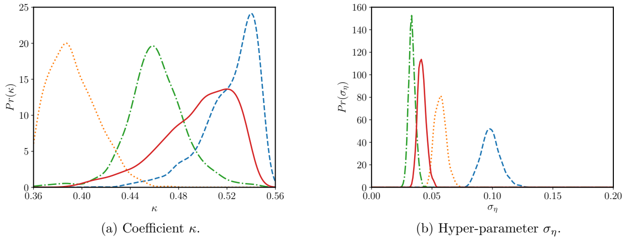
Figure 5.2: Posterior probabilities in case of Spalart–Allmaras model: Scenario 1 (---), Scenario 2 (.....), Scenario 3 (-.-.) and Scenario 4 (—). Priors has been chosen uniform on [0.36, 0.56] and [0, 1] respectively.
