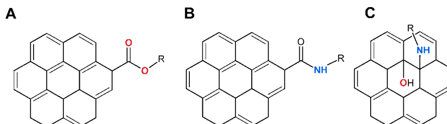
Figure 1.4 Different species can be formed after the covalent functionalization of GO: a) esters, b) amides and c) secondary amines.
