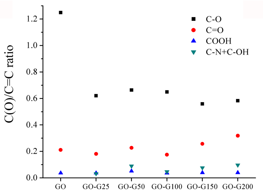
Figure 2.6 Ratio area of C(O) bonds to the C=C bonds
