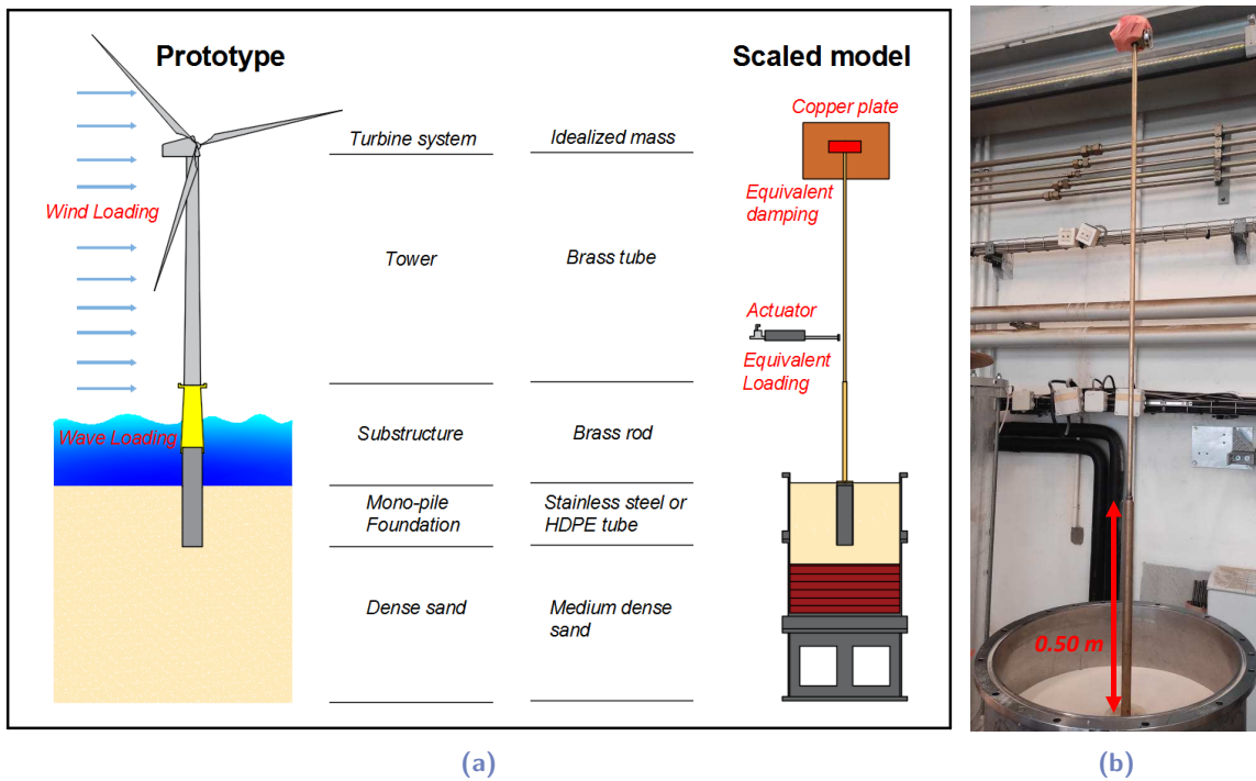
Fig. 2.18.: (a) Schematic of similarity between the designed scale models and the prototype; (b) photo of scale model M2
