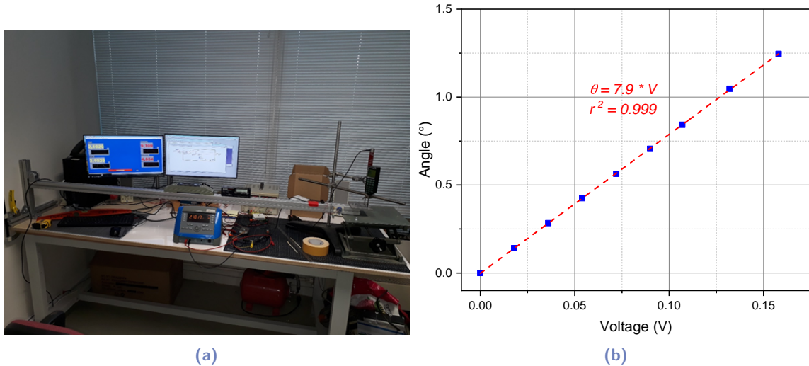
Fig. A.4.: Calibration of inclinometer used in the monotonic and cyclic test procedures: (a) photo, (b) results
