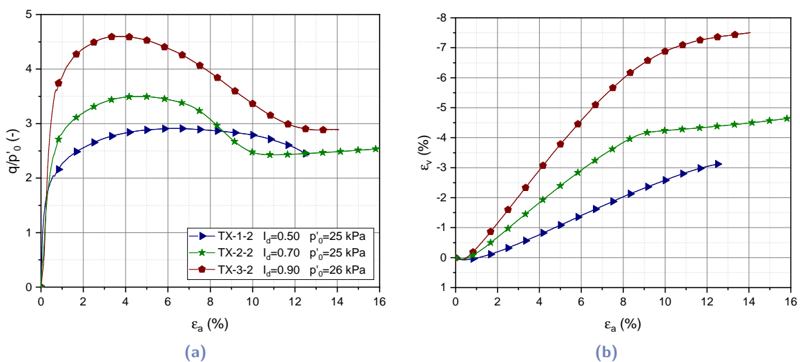
Fig. 3.17.: Influence of relative density index on sand behavior at low confining stress level ( p'_0 = 25 \text{ kPa} ): (a) q - \epsilon_a (b) \epsilon_v - \epsilon_a
