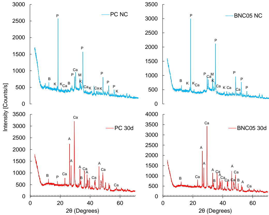
Fig. 4.45: XRD patterns of non-modified cement (PC) and modified cement (BNC05) cured at 90°C before carbonation (NC), and after 30-days of carbonation (C).
