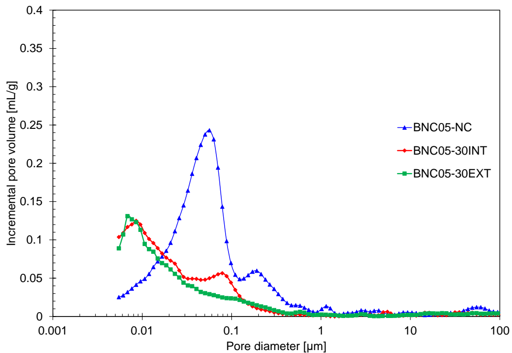
Fig. 4.40: Pore size distribution of 30-days carbonated and non-carbonated BNC05 samples cured at 90 °C. The red curve corresponds to the cement core, while the green curve corresponds to a sector near the exposed surface.
