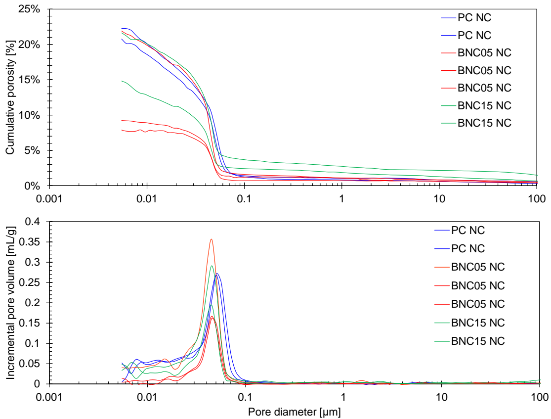
Fig. 4.13: Cumulative porosity and pore size distribution of PC, BNC05 and BNC15 in non-carbonated samples. Results are shown up to values of 0.006 \mu\text{m}
