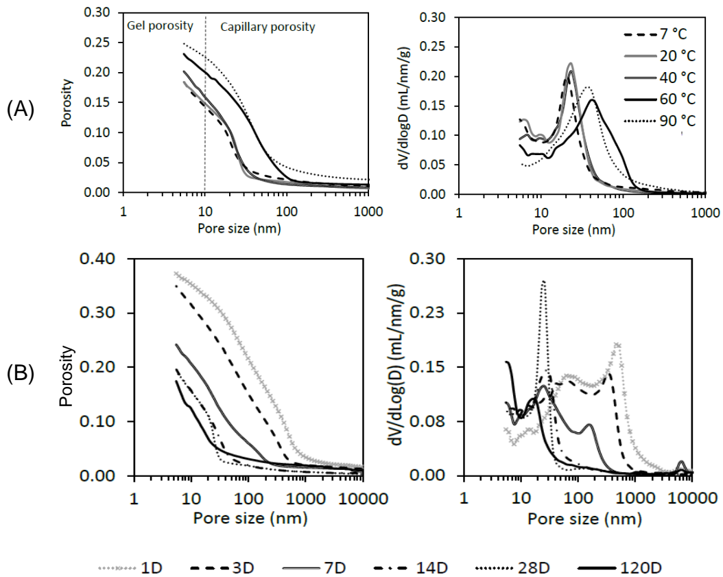
Fig. 2.13: (A) Porosity and incremental pore volume as a function of temperature after 28 days of curing, (B) Variation of porosity and incremental pore volume as a function of time for samples cured at 20 °C (after Bahafid [60]).
