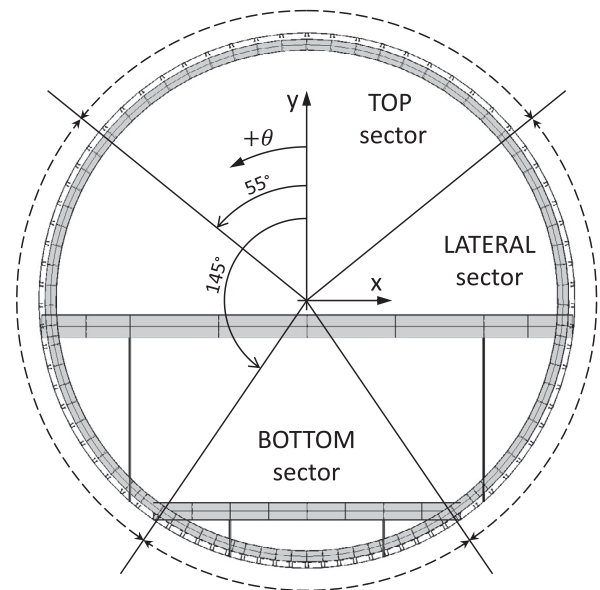
Fig. 3. Fuselage cross-section.
