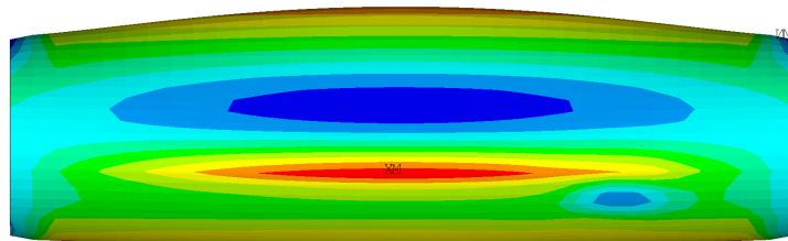
(a) Contour plot of the hoop stress in skin under BLC_p
