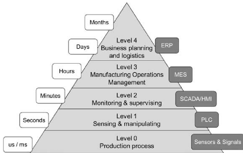
Figure 2.6 The automation pyramid (ANSI/ISA-95, 2013)
