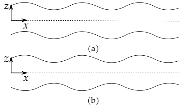
Fig. 3.6 Particle motion associated to antisymmetric (a) and symmetric (b) fundamentals Lamb waves modes.
