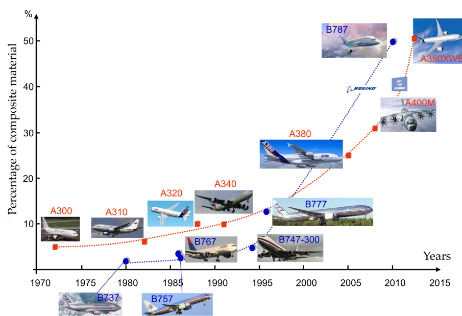
Fig. 3.2 Evolution of composite material percentage in commercial aircrafts composition. Adapted from [9].
