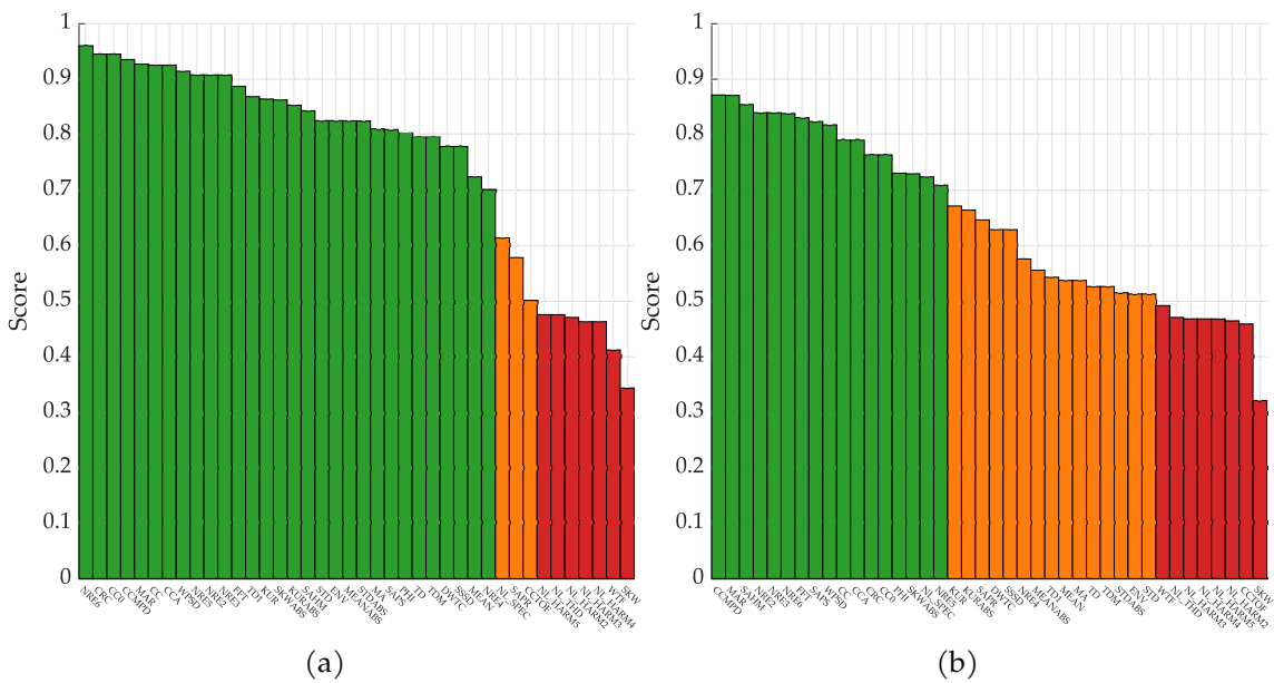
Fig. 4.27 Score of all DI at an excitation frequency of 200 kHz for second L1 campaign for an excitation frequency of 100 kHz (a) and 200 kHz (b). Bars in green correspond to score above 0.7, orange to a score above 0.5 and red to a score under 0.5.
