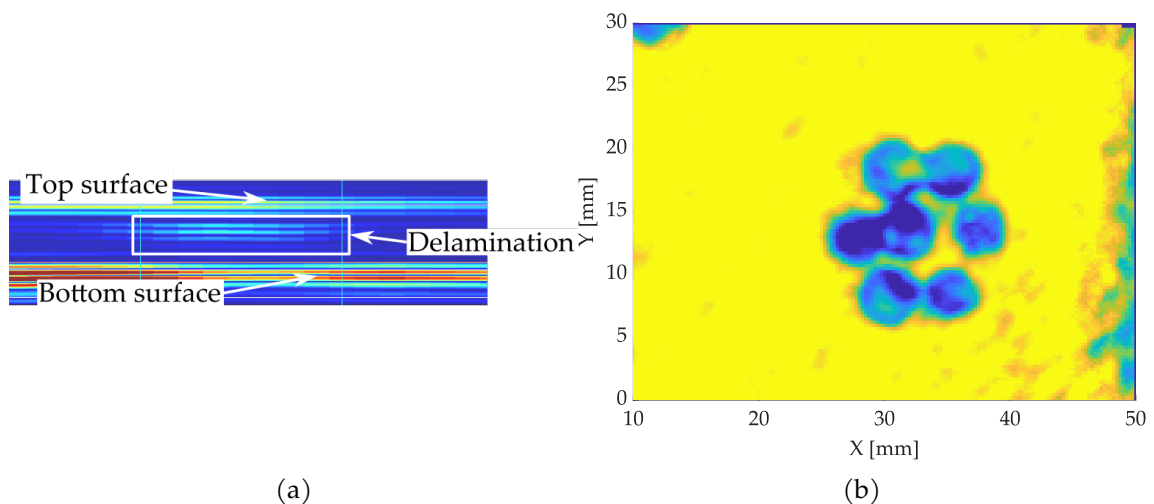
Fig. 4.22 A-scan of the laser shocked area of the L1 coupon (a). C-scan of the laser shocked area of the L1 coupon (b).
