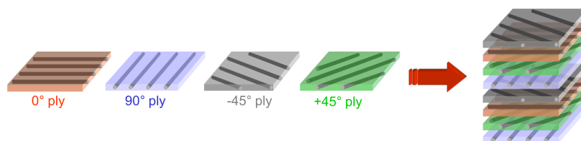
Fig. 3.1 Illustration of draping process. Adapted from [9].
