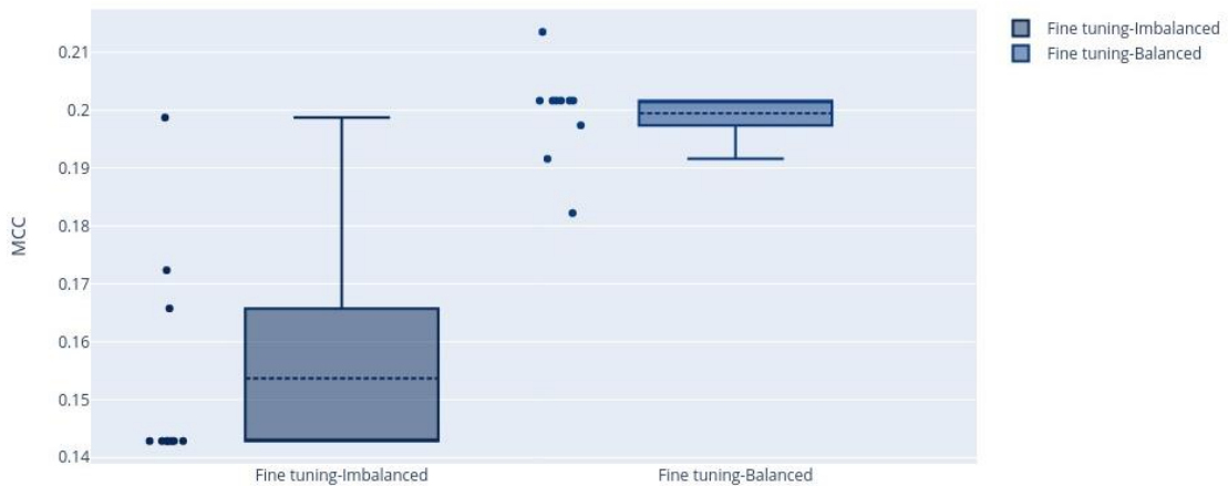
Figure 5.15 Box plots for the validation of MCC in fine-tuning mode for a workload cluster classification.
