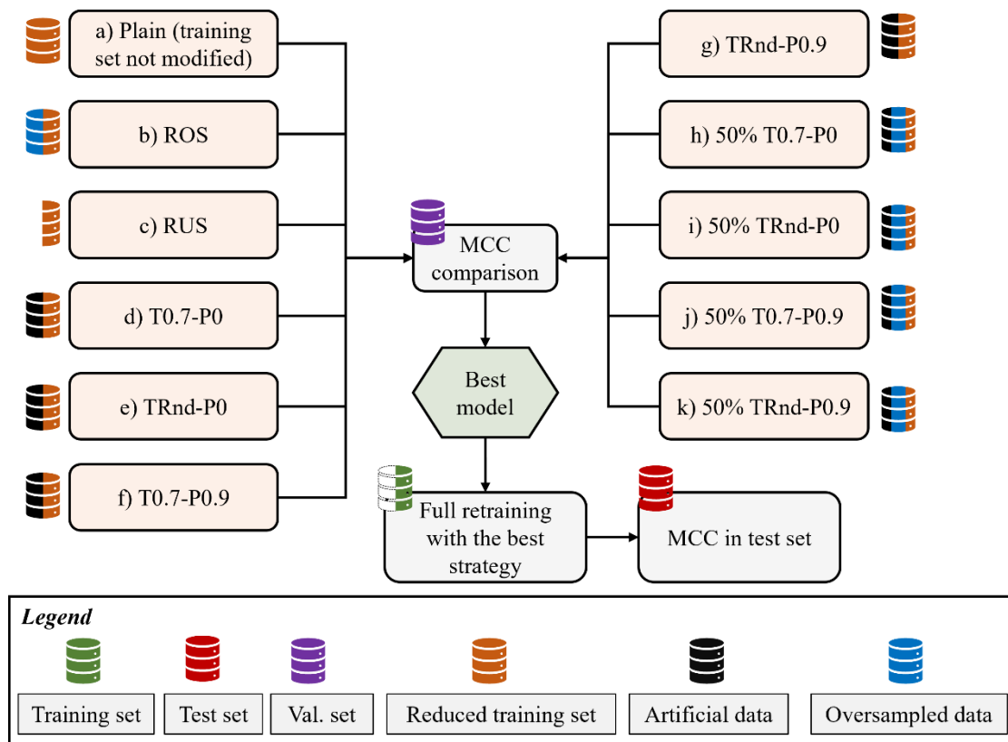
Figure 7.2 Training policy for the issue classification module.
