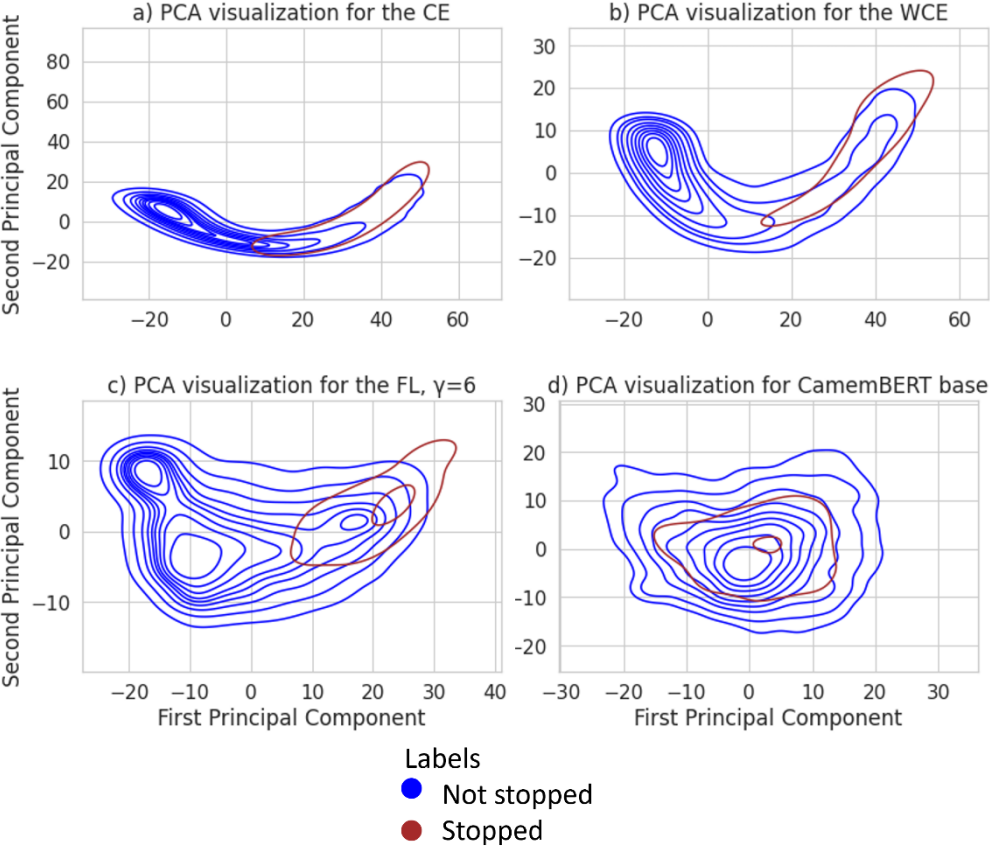
Figure 8.3 Kernel density plots for CamemBERT using cross-entropy (a), weighted cross-entropy (b), focal loss with \gamma=6 (c), and with no fine-tuning (d)
