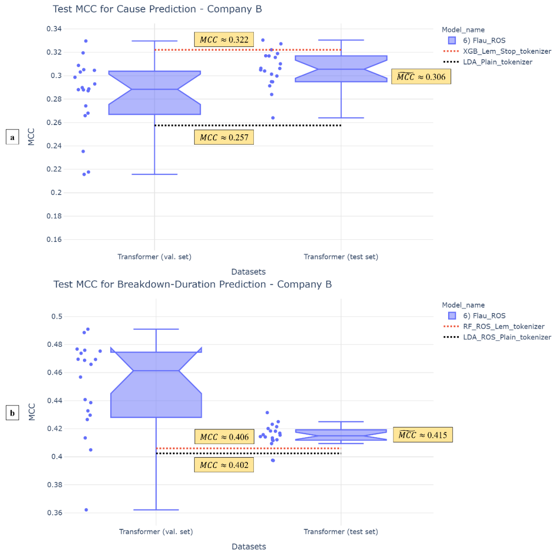
Figure 6.9 Test MCC box plots for (a) cause and (b) breakdown-duration prediction in Company B.
