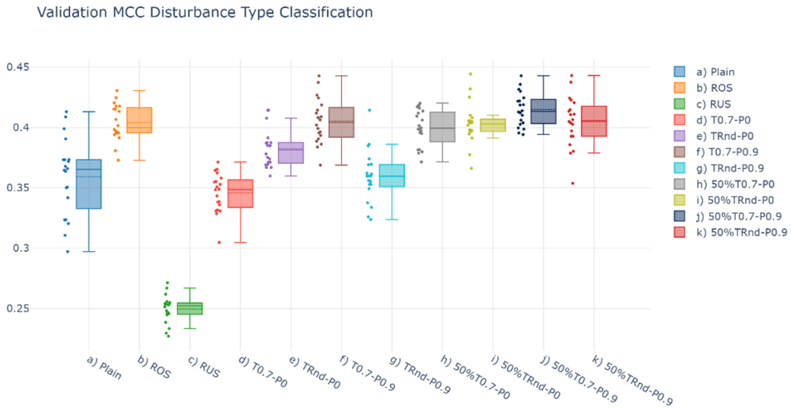
Figure 7.4 Validation MCC for the eleven CamemBERT models.
