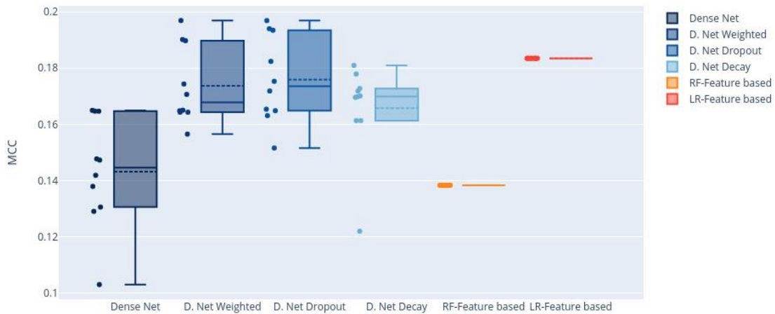
Figure 5.14 Box plots for the validation MCC in a feature-based mode for workload cluster classification.
