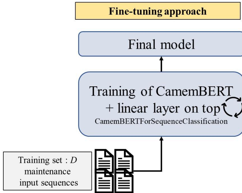
Figure 5.9 Functioning of the fine-tuning approach with CamemBERT.
