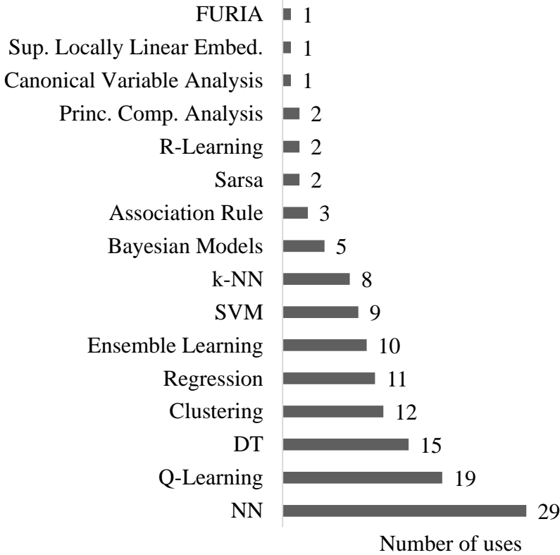
Figure 4.7 Number of uses by technique family.
