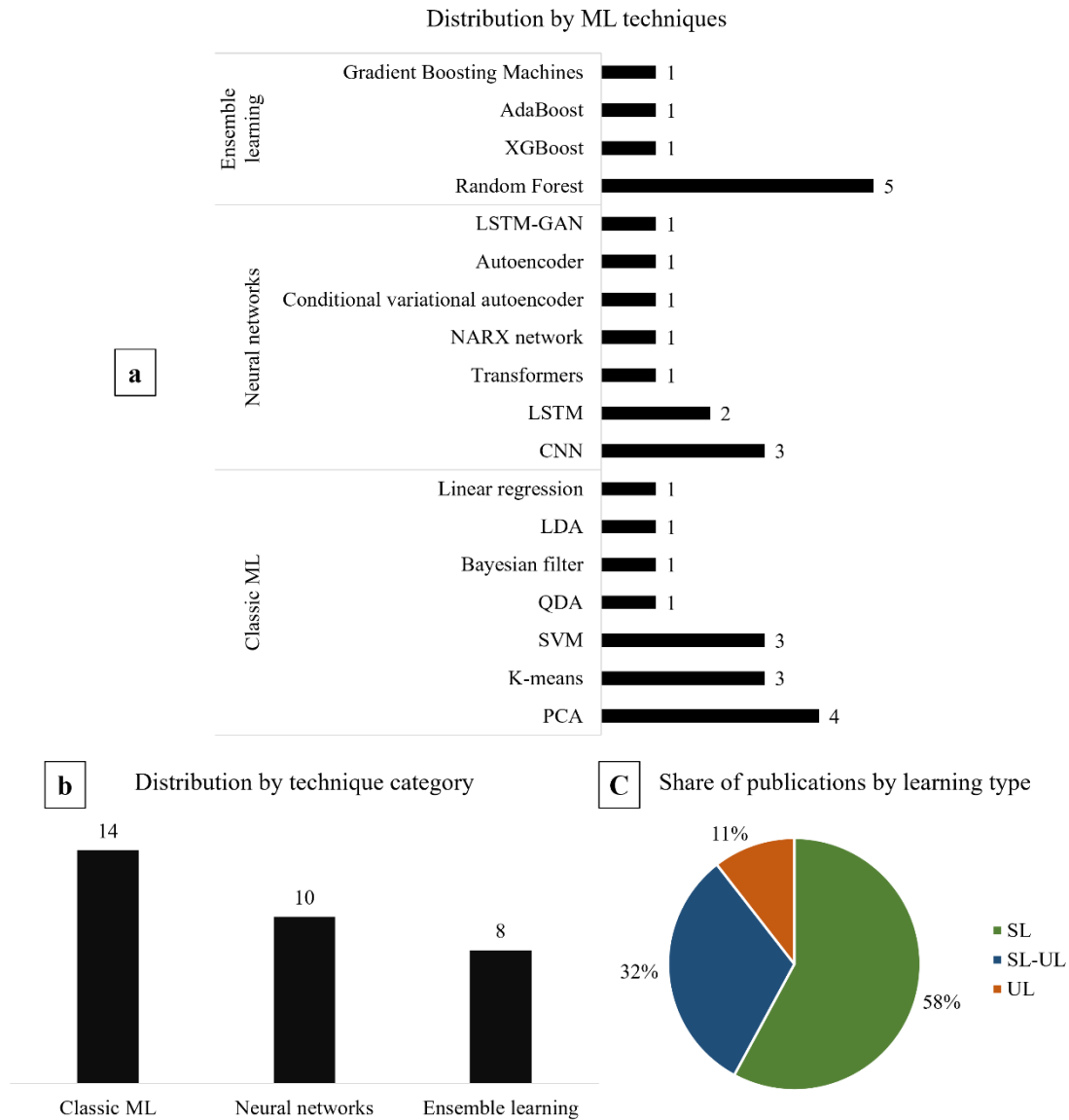
Figure 2.4 Results for the second axis of the analytical framework: ML techniques (a), technique categories (b), and learning types (c)
