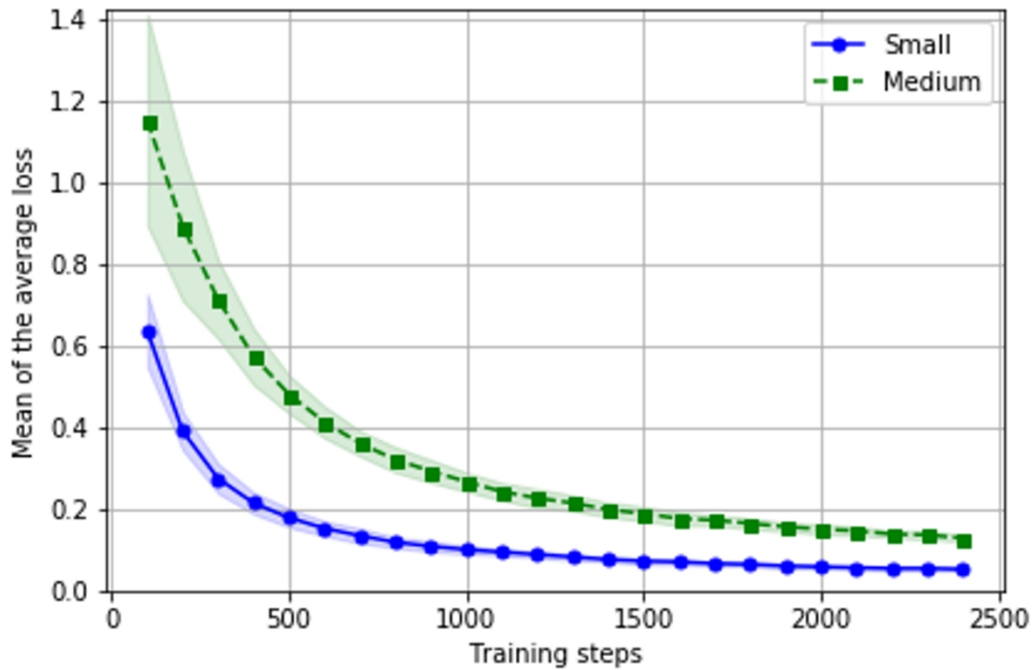
Figure 7.3 Mean average training loss for the small (blue) and medium (green) GPT-2 model. Findings suggest that the language model that better fits the text descriptions for dominant disturbances is the small model. This may indicate that when language models have relatively little data to learn (around 1300 examples), smaller models perform better. Thus, the small architecture was used to generate the artificial data for the following experiments. Finally, it is worth noting that the GPT-2 model used from (Woolf, 2019) was originally designed for English. Thus, the generated texts dropped all of the uniquely French characters.
