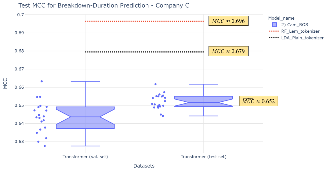
Figure 6.10 Test MCC box plots for breakdown-duration prediction in Company C.
