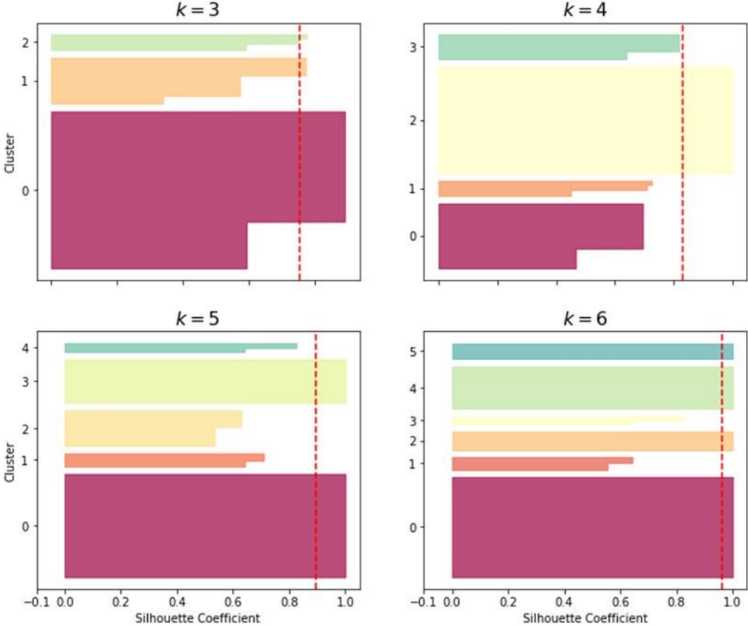
Figure 5.7 Silhouette diagrams with a different number of clusters.
