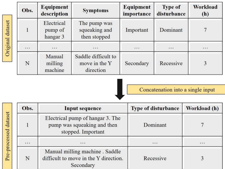
Figure 5.3 Example of the pre-processing that was performed.
