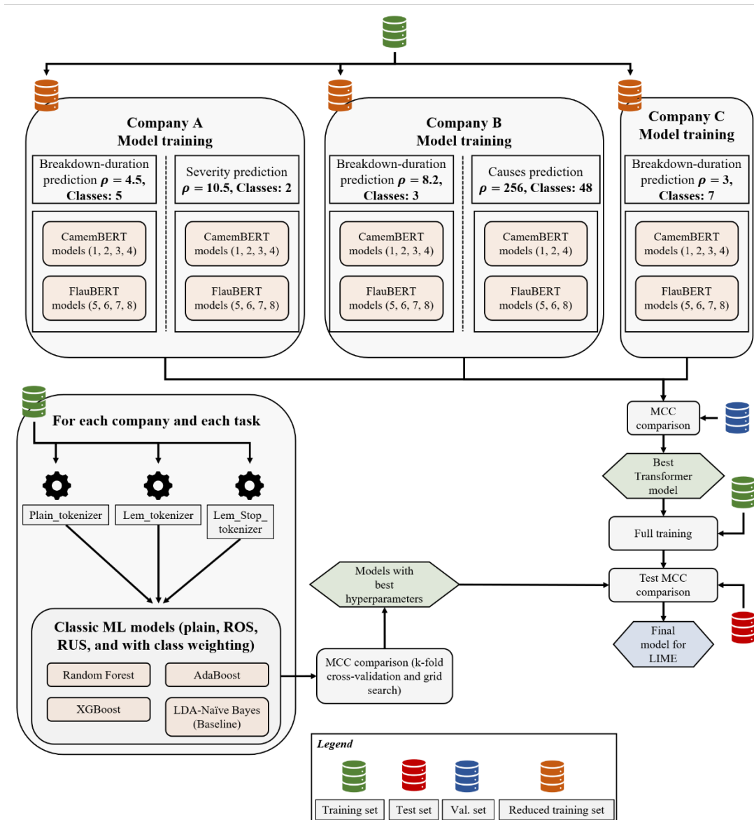
Figure 6.4 Training policy and model selection.
