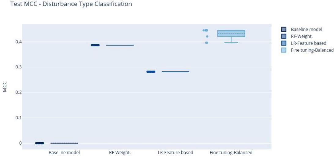
Figure 5.13 Box plots for the test MCC in a disturbance classification.
