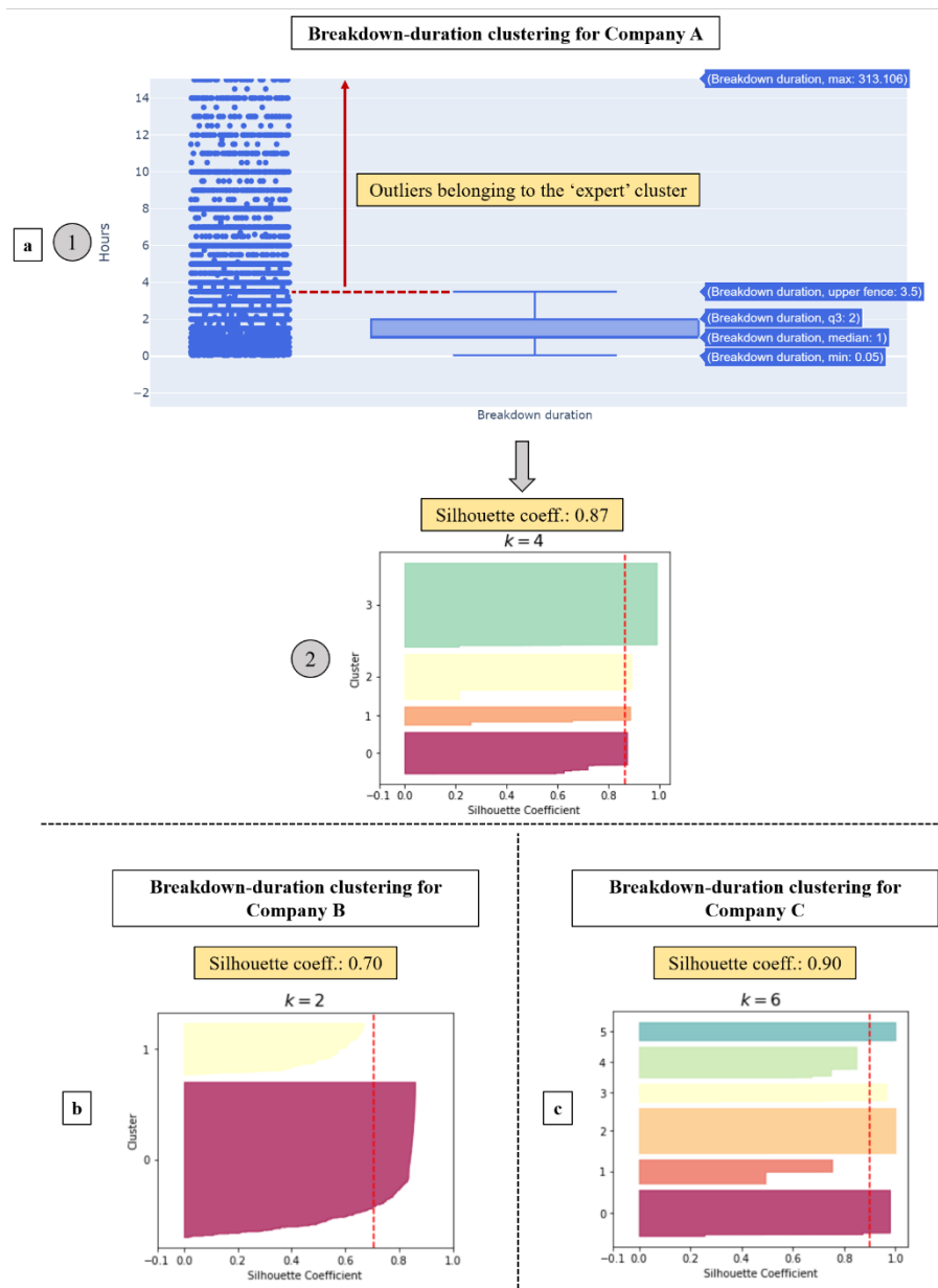
Figure 6.3 First two pre-processing steps for breakdown-duration clustering in Company A (a), and results of the second step for Companies B (b) and C (c).
