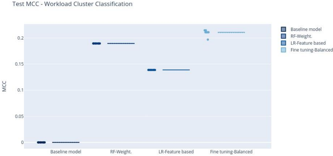
Figure 5.16 Box plots for the test MCC.
