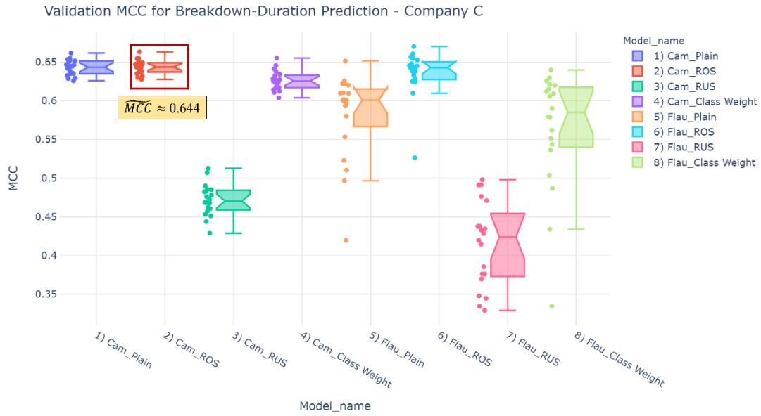
Figure 6.7 Validation MCC box plots for breakdown-duration prediction in Company C.
