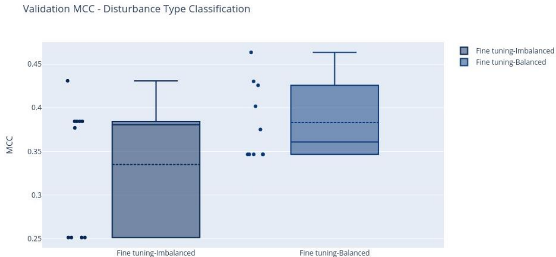
Figure 5.12 Box plots for the validation MCC in fine-tuning mode for disturbance classification.
