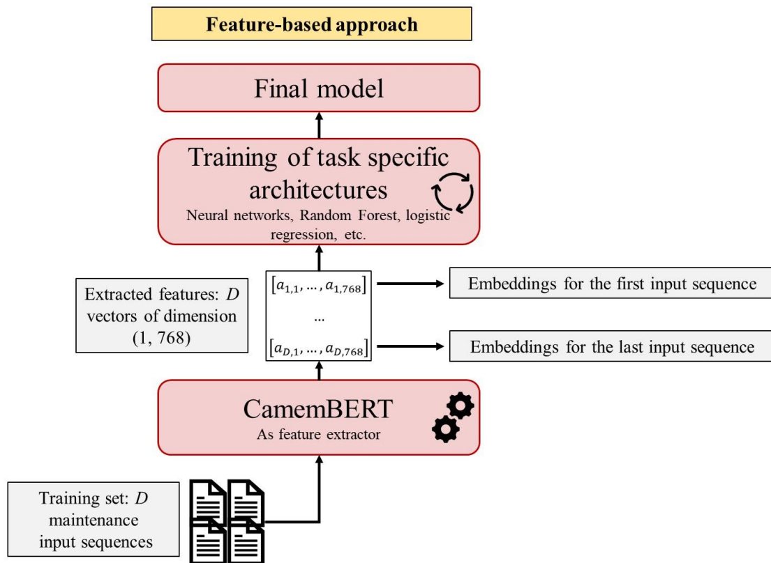
Figure 5.8 Functioning of the feature-based approach with CamemBERT.
