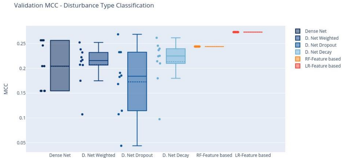
Figure 5.11 Box plots for the validation of MCC in feature-based mode for disturbance classification.
