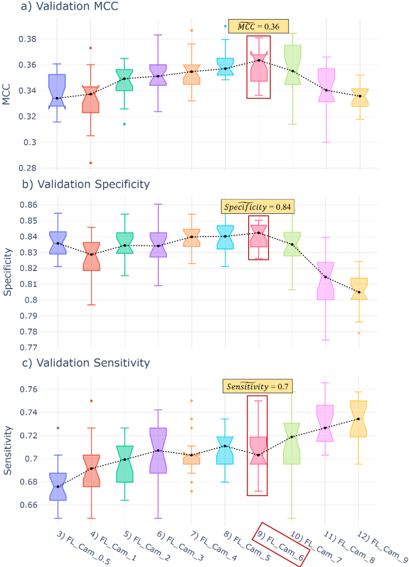
Figure 8.1 Validation of MCC (a), specificity (b), and sensitivity (c) for different focusing parameter values
