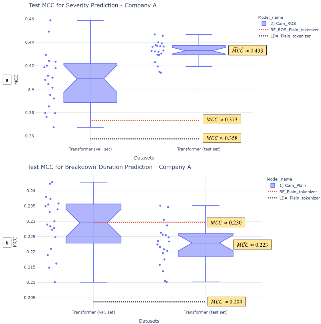
Figure 6.8 Test MCC box plots for (a) severity and (b) breakdown-duration prediction in Company A.
