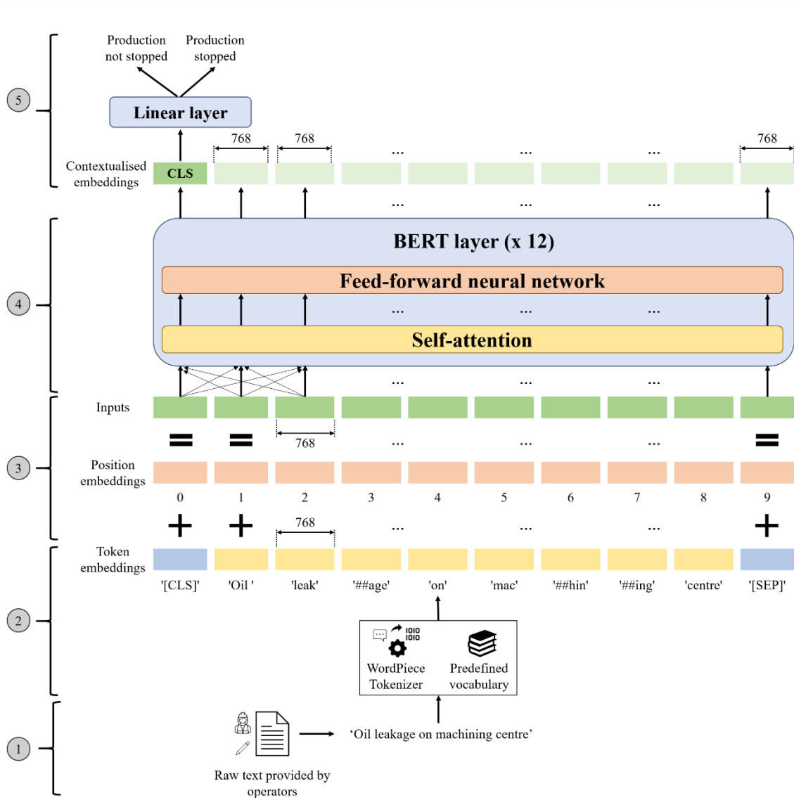
Figure 6.1 Example of a trained BERT for text classification.
