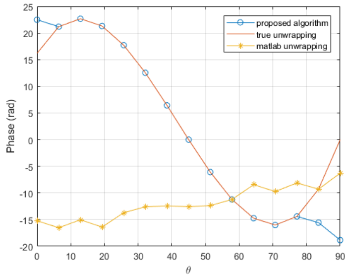
Figure 2.6 – Comparison of the proposed procedure and the Matlab unwrapping function in a coarse mesh consisting of 15 nodes with the 1/k_f factor 20% higher
