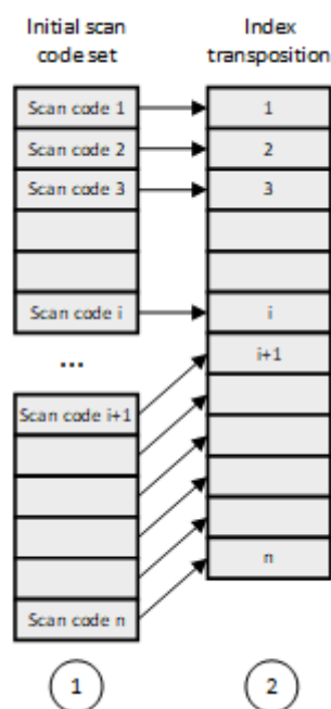
Figure 6.7: Transposition from scan code to index.
