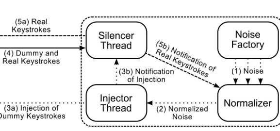
Figure 5.19: Architecture of noisykey.dll .
