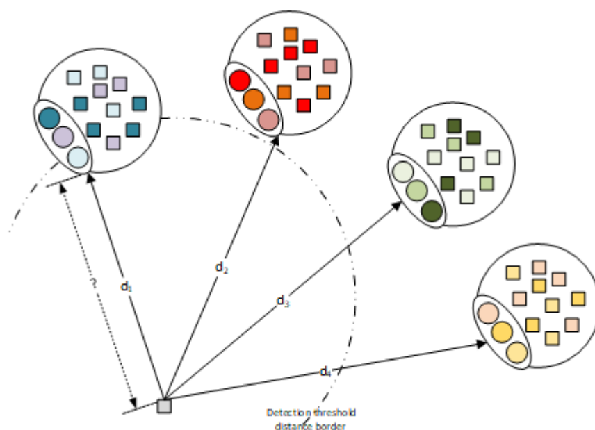
Figure 7.14: Classification of a new element in our unsupervised data-mining clustering system.
