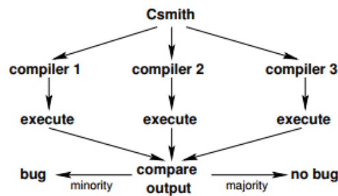
Figure 2.4: Csmith’s finding bugs procedure.
