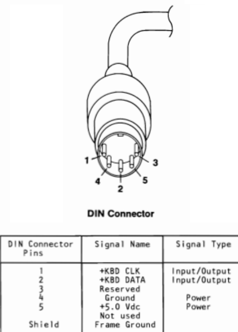
Figure 4.12: Representation of DIN connector.
