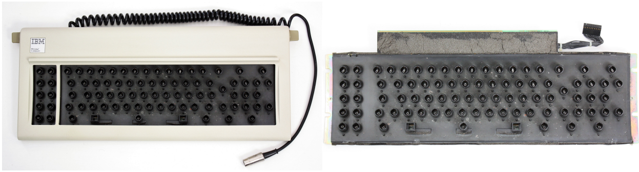
Figure 4.4: Keyboard IBM-PC model F type 1 mechanism from top without key.
