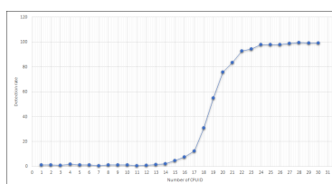
Figure 3.34: Linux Host.
