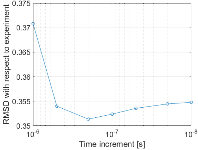
FIGURE 4.4: RMSD of first wave packet between simulated and experimental responses with different time increments.
