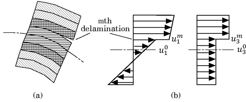
FIGURE 2.10: Kinematic assumptions of generalized laminate theory with single delamination [24]. U^m indicates the displacement of m th delamination along x -axis.
