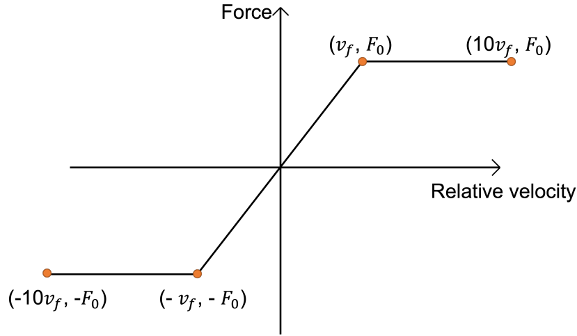
FIGURE 4.26: Schematic of nonlinear in-plane interaction model
