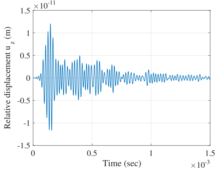
FIGURE 4.43: Relative displacement in out-of-plane direction of the center node for k^{spr} = 0 case of the two-impact plate.
