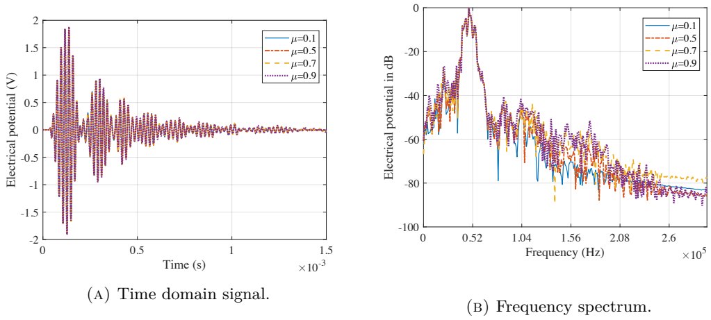
FIGURE 4.53: Electrical output signals in both time and frequency domains from three-impact plate using contact/friction model with different friction coefficients.
