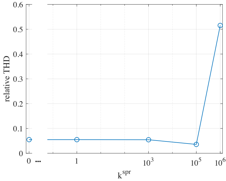
FIGURE 4.59: Effect of spring stiffness on relative THD of the electrical output signals of the three-impact plate.
