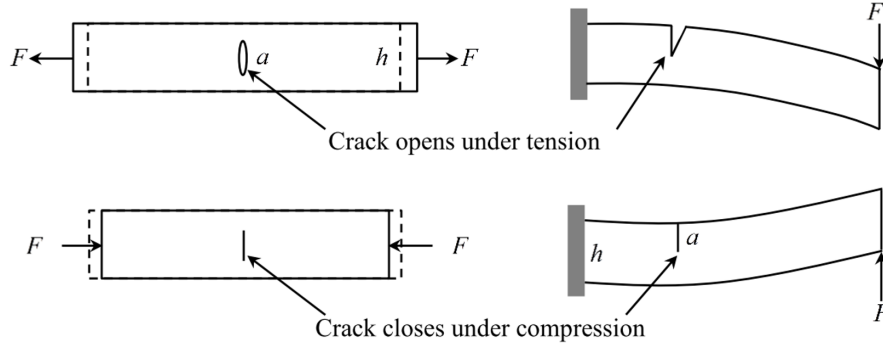
FIGURE 2.6: Schematic of the "breathing" type crack in structures having a bi-linear contact behavior [20].
