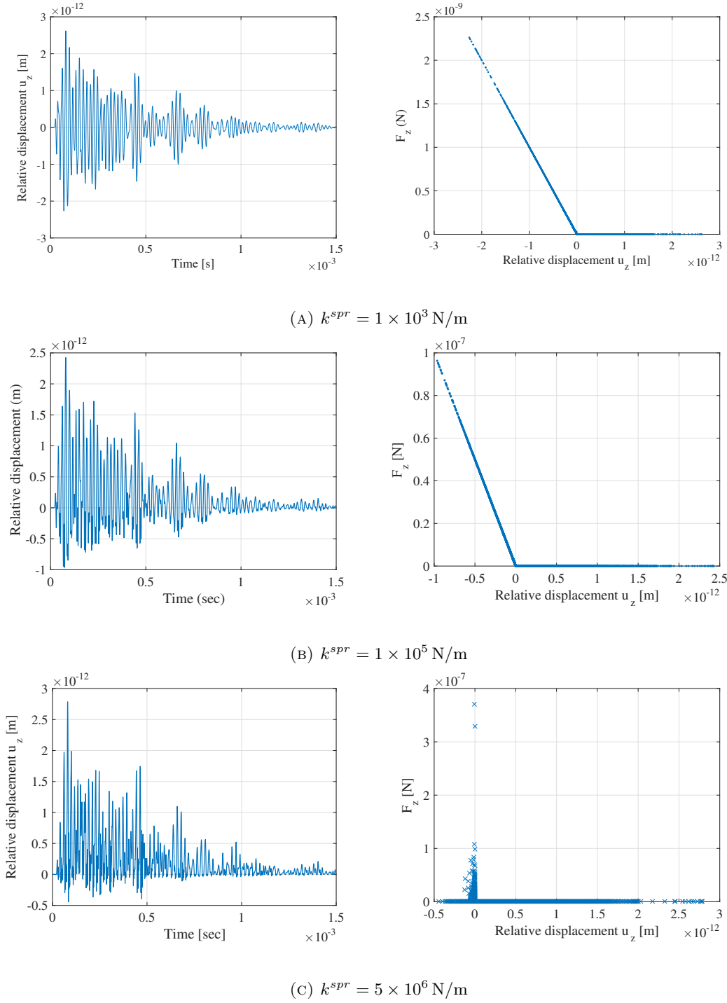
FIGURE 4.41: Mechanical behavior of the center point of the delamination from one-impact plate with different spring stiffness values. Left: relative out-of-plane displacement of the center point. Right: relationship between spring force and relative displacement in out-of-plane direction.
