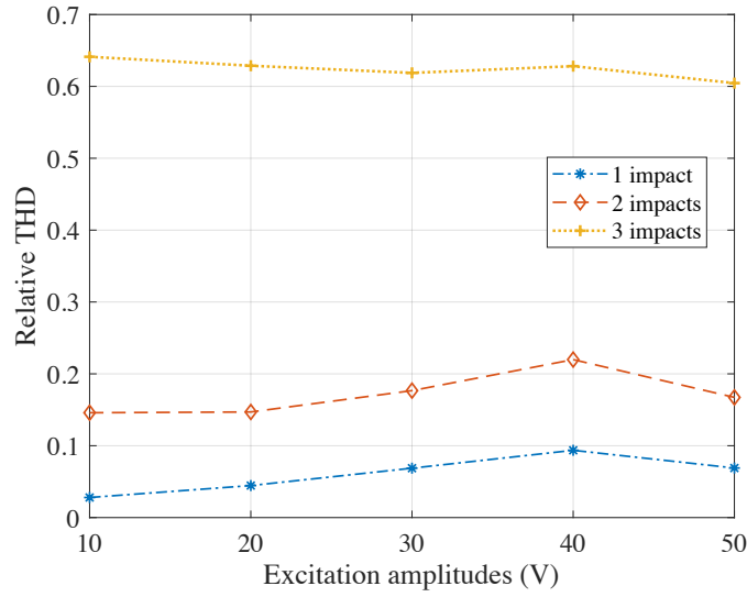
FIGURE 3.15: Variation of DI based on relative total harmonic distortion (THD) against excitation amplitude on different specimens.
