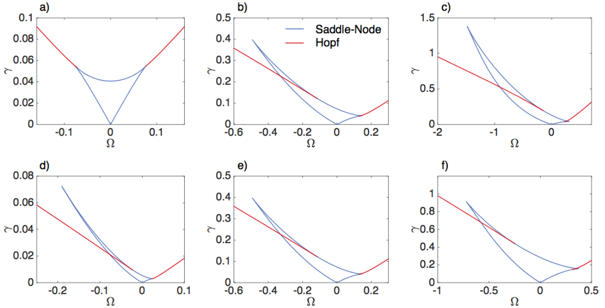
Figure 6.11: Analytical simulations of the 12 \text{ }\mu\text{m} Fabry-Perot QCL subject to optical injection. First row: constant bias current I = 1.5 \text{ A} with a) \alpha = 0 , b) \alpha = 1.5 and c) \alpha = 3 . Second row: fixed \alpha = 1.5 and d) I = 1.25 \text{ A} , e) I = 1.5 \text{ A} , f) I = 2 \text{ A} .
