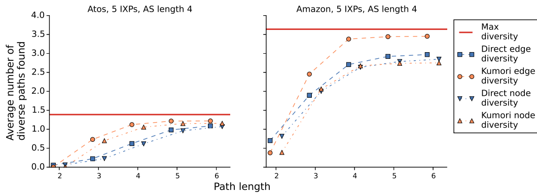
Figure 6.5 – Average number of diverse path found per maximum path length for Amazon and Atos
