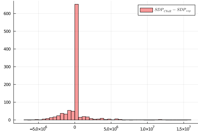
Figure 7.9: Histogram of the score difference between SDP_{esp} and SDP_{CVaR} over the assessment set
