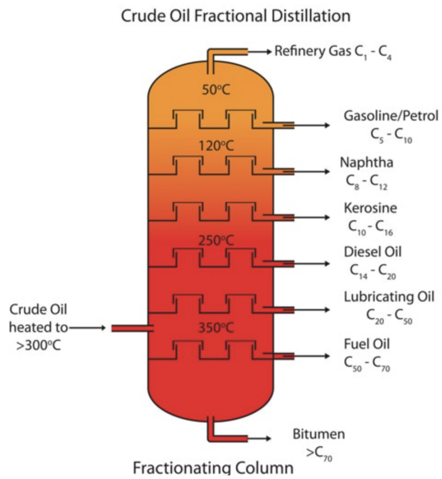
Figure 3.4: Simplified view of a distillation column
