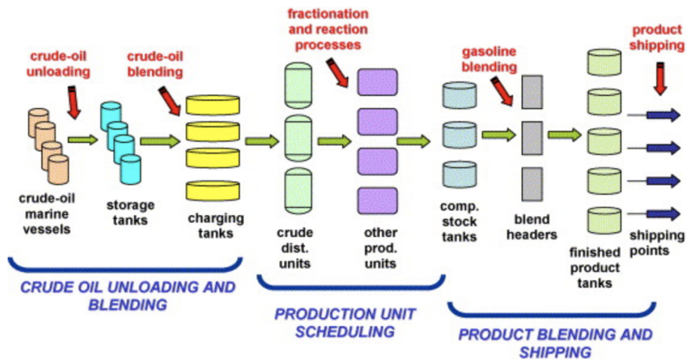
Figure 1.5: Schematic representation of the processing steps inside a refinery
