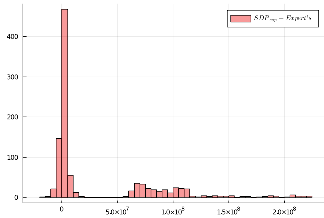
Figure 7.7: Histogram of the difference between SDP_{esp} and Expert across 1000 assessment scenarios.
