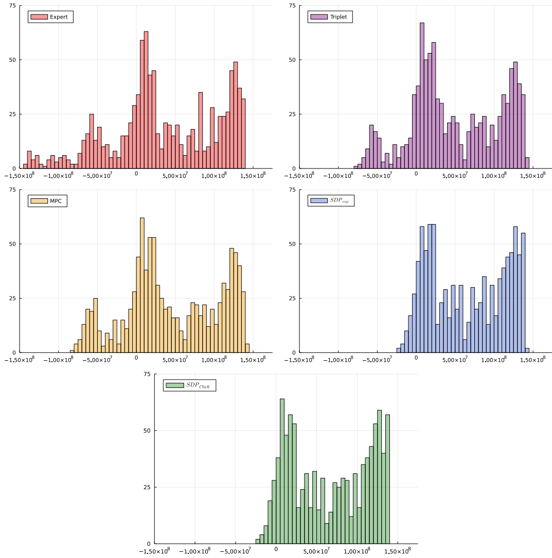
Figure 7.6: Histogram of operating margins over Monte-Carlo for five policies: Expert , Triplet , MPC , SDP_{esp} and SDP_{CVaR} .
