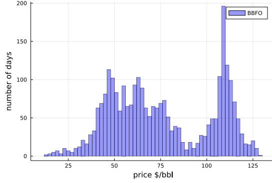
Figure 7.3: Histogram of the daily reference quotations over a 10-years period (n=2778)
