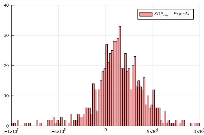
Figure 7.8: Zoom of Figure 7.7 on the interval [-1.10^7, 1.10^7]
