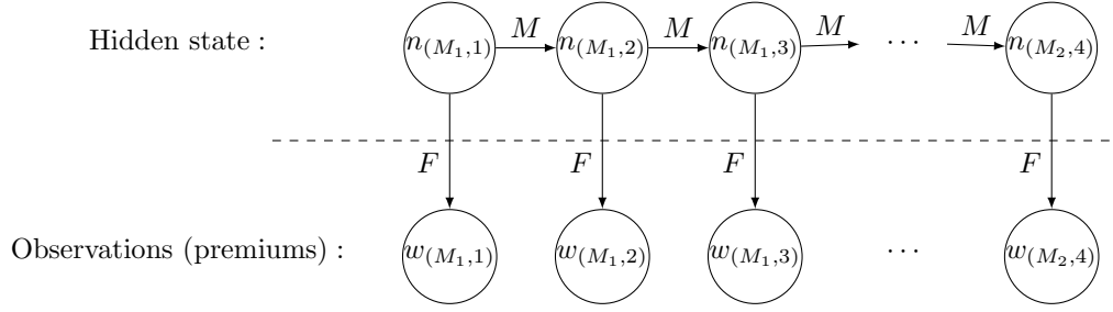
Figure 4.2: Illustration of the hidden markov chain modeling the crude oil premiums
