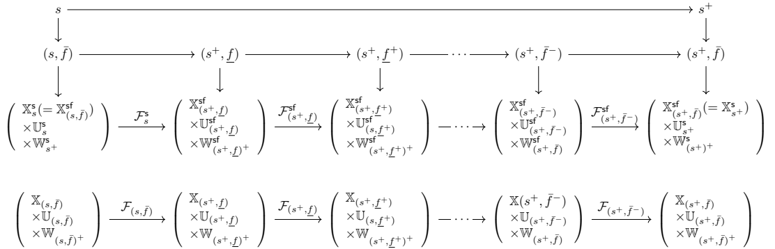
Figure 9.3: Original dynamics and their reformulation on the product timeline on the slow time interval [s, s^+]
