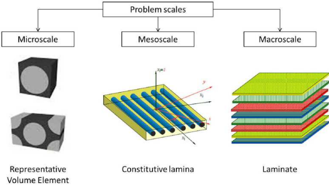
Figure 2.1: The different scales involved in the design problem of multilayer structures [5].
