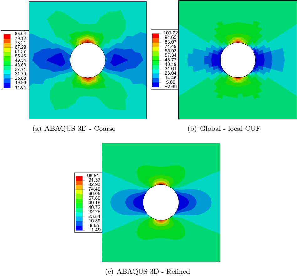
Figure 3.23: Axial stress \sigma_{xx} [MPa] in the plane x - z of the notched plate.
