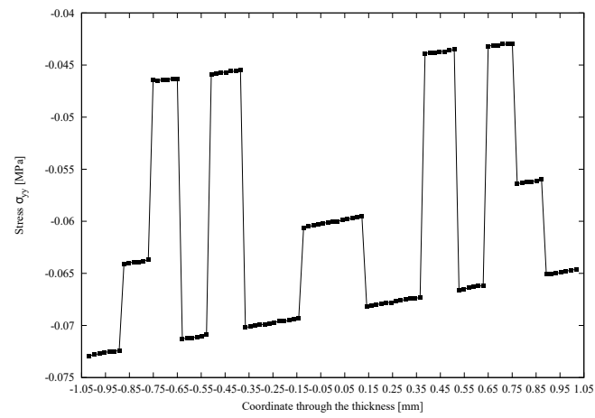
(b) \sigma_{yy}
