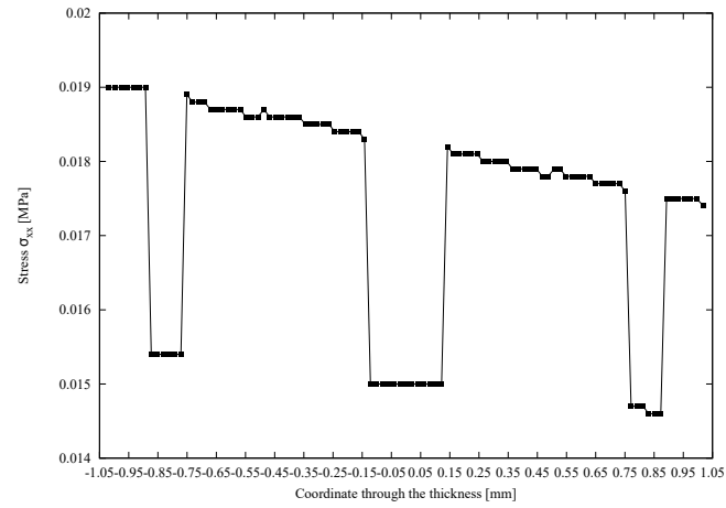
(a) \sigma_{xx}
