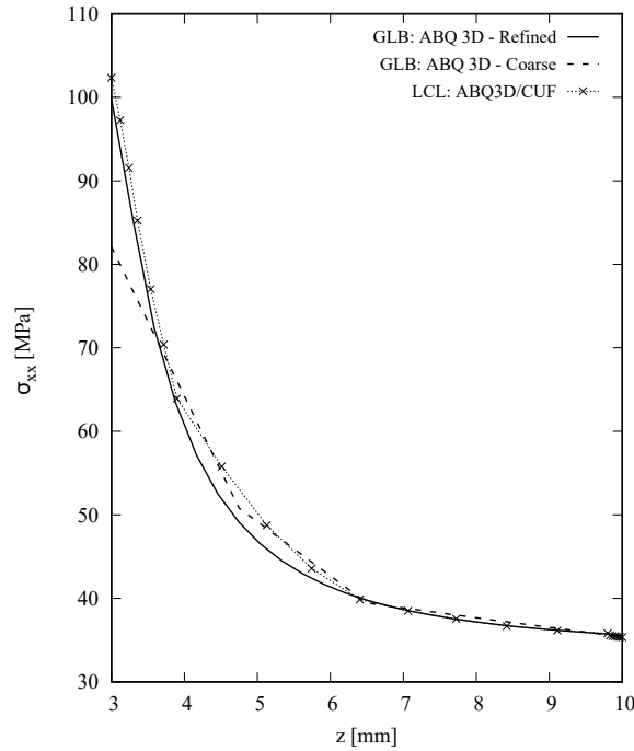
Figure 3.22: Axial stress \sigma_{xx} along the z axis.
