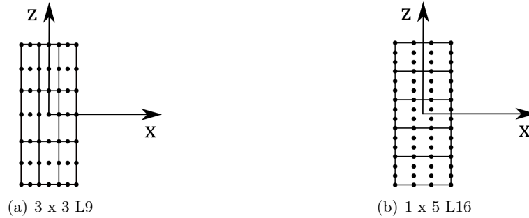
Figure 3.12: Sub-domain distributions over the cross-section of the local CUF beam model
