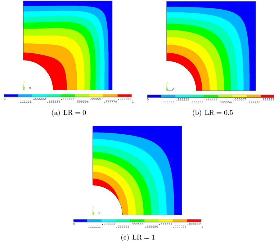
Figure 6.11: Mode shape related to the first buckling load for the optimised solutions listed in Table 6.11.
