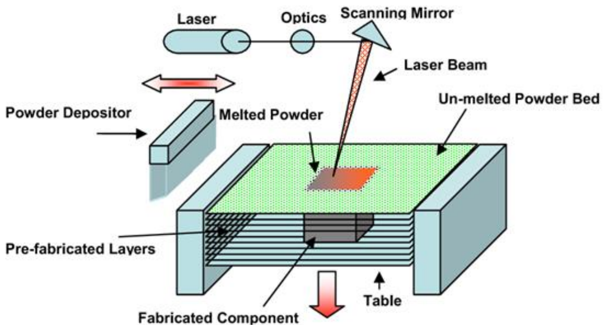
Figure 1.12. A schematic representation of an SLM configuration [65].
