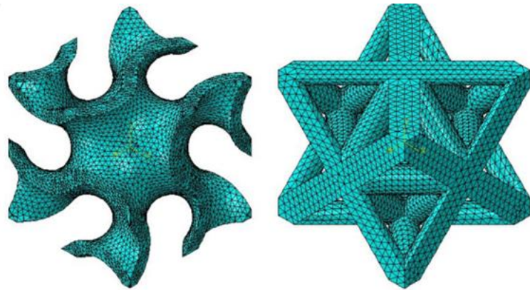
Figure 2.13. Gyroid sheet and Octet-truss unit cells as meshed with tetrahedral elements in Abaqus software.
