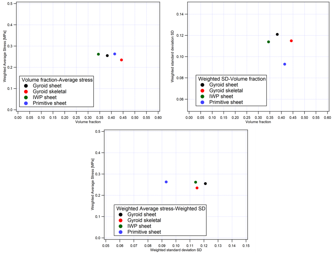
Figure 4.13. a) volume fraction-weighted average stress, b) weighted SD-volume fraction, and c) weighted average stress-weighted SD graphs for all the studied unit cells.
