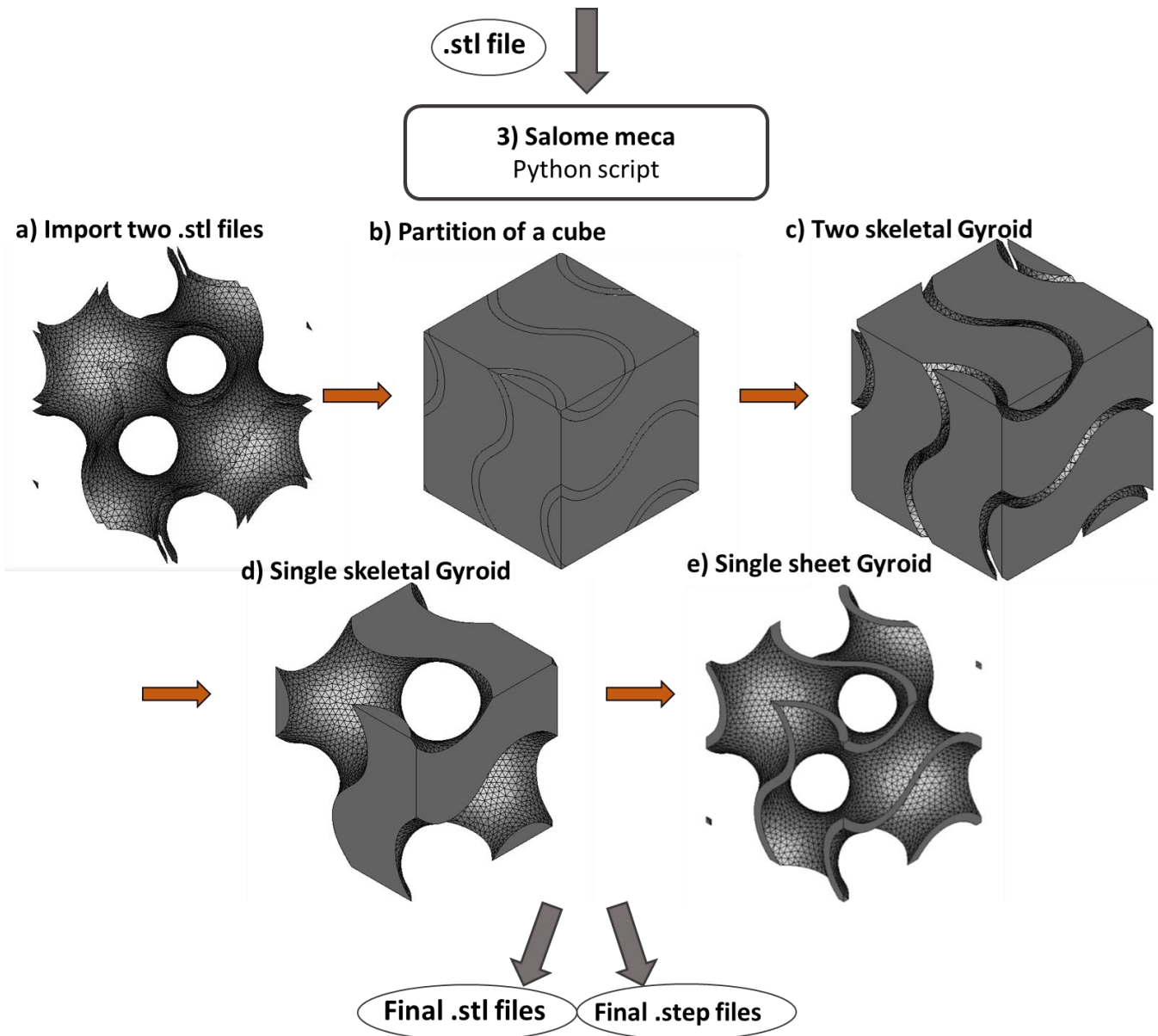
Figure Appendix.1. Complete numerical chain regarding the design of Gyroid unit cells.
