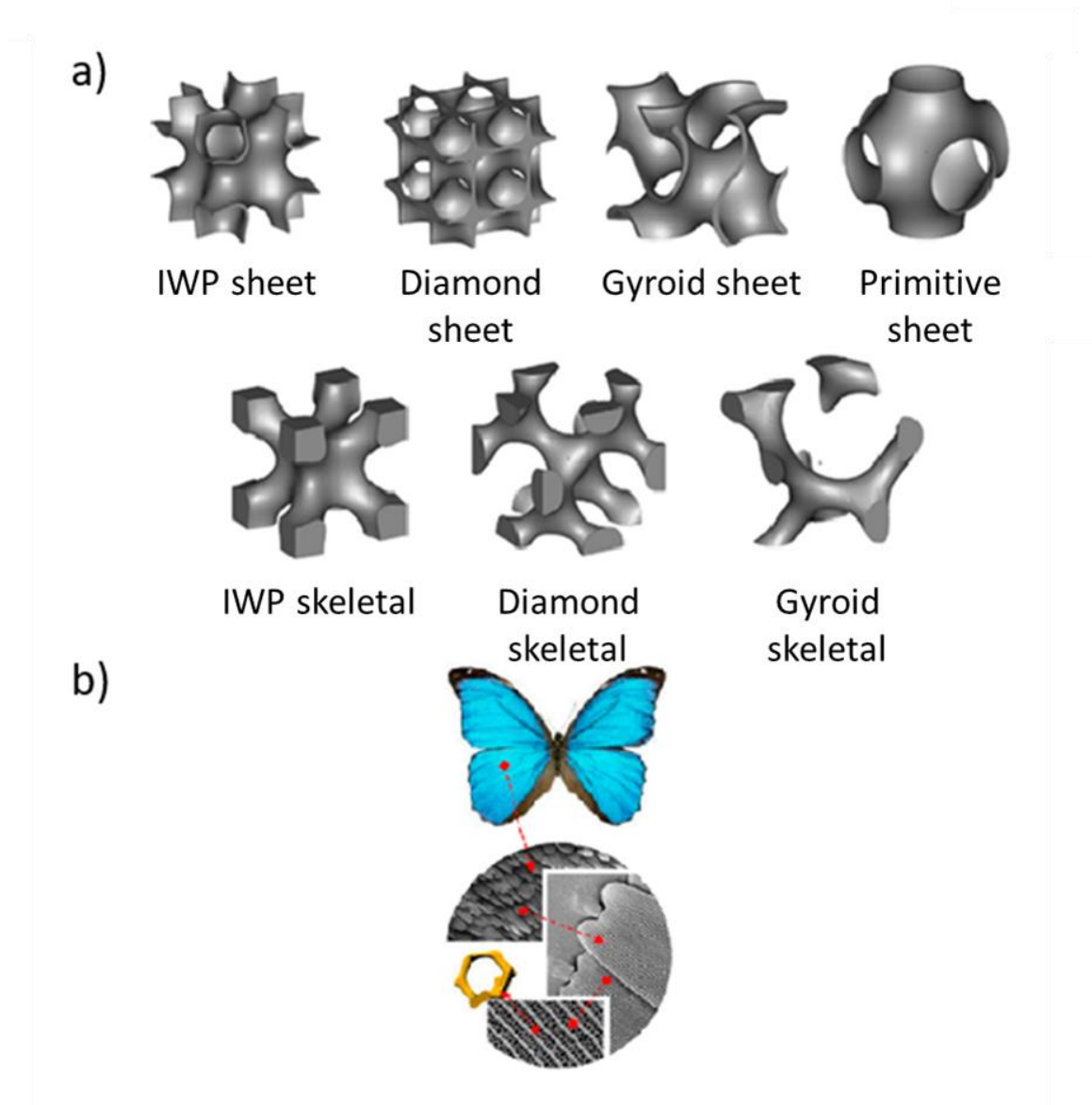
Figure 1.7. a) Several TPMS unit cells in the domain [0-2*\pi] and their names [40], b) the wings of a butterfly with a Gyroid-like structure [48]
