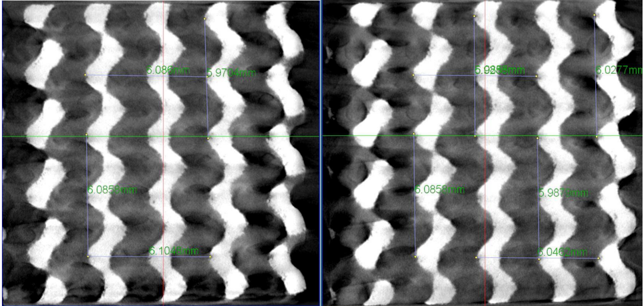
Figure 3.6. Two planes with multiple length measurements between two peaks of the Gyroid skeletal topology at a compressive load of 90\% * F_{max} \approx 20500 N .
