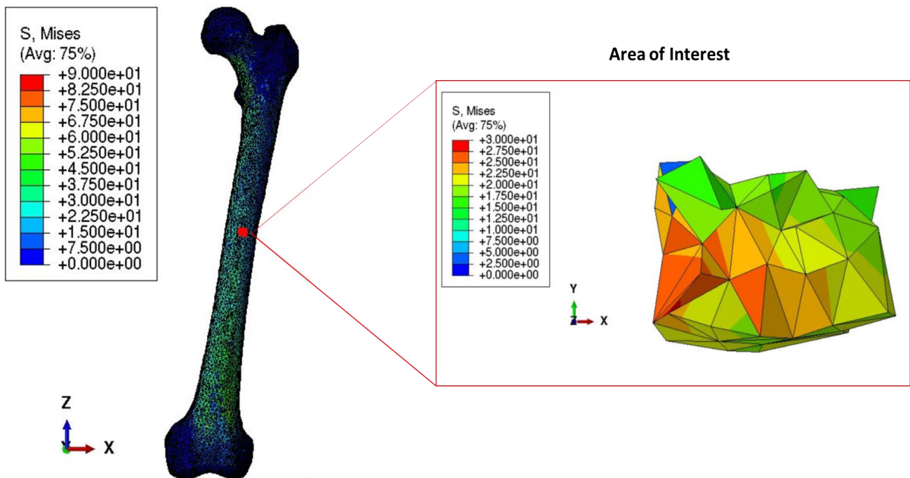
Figure 4.9. Von Mises stress contour of the whole femur and the AoI and the relevant contour legends.
