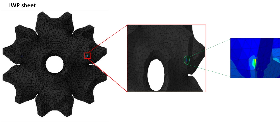
Figure 4.11. A neglected singularity in a relevant element for the IWP sheet topology caused by errors that arise either from the interpolation of the PBC or by the edges.
