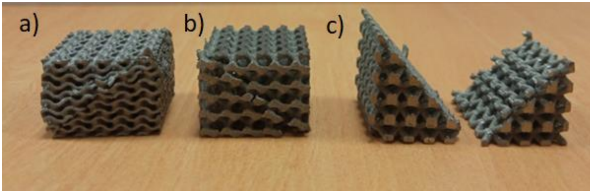
Figure 3.10. Macroscopic fracture at 45^\circ for three lattice topologies, i.e. a) Gyroid sheet, b) Gyroid skeletal, and c) Diagonal topology.
