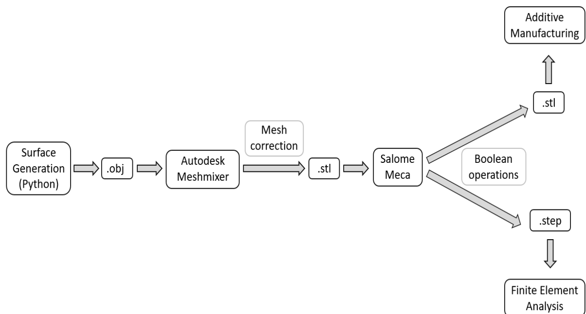
Figure 2.1. Complete numerical chain for the design process followed in this study.
