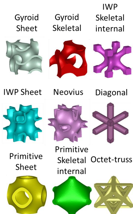
Figure 2.5. All numerically investigated unit cell topologies.
