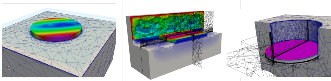
Figure 3.7: Sketches of geometries studied in our numerical applications: simple compression, plane strain and oedo test.
