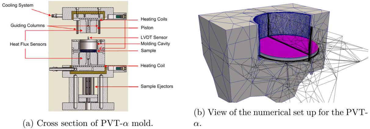
Figure 4.4: (a) Details of experimental mold for sample of 6 mm \times 50 mm dimension. Location of LVDT and other sensors. (b) visualization of immersed mold and sample into computational domains.
