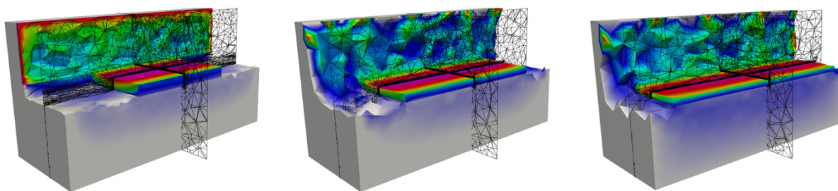
Figure 3.23: Plane strain: Compression of SMC within a channel.
