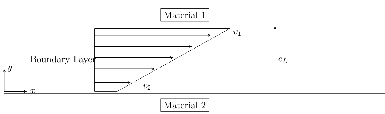
Figure B.1: Representation of the boundary layer
