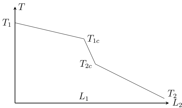
Figure C.1: Temperature field along the bodies in contact : Contact thermal resistance modeling by the insertion of a third thin body of thickness e .
