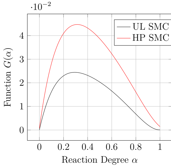
Figure 4.1: Thermo-kinetic function G(\alpha) for ultra light (UL) and high performance (HP) SMCs. Figure 4.2: Thermo-kinetic Function K(T) for ultra light (UL) and high performance (HP) SMCs.
