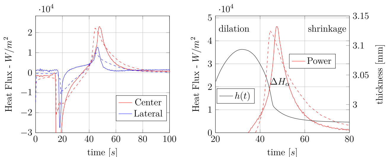
(a) Evolution of heat flux in T1 and T2
