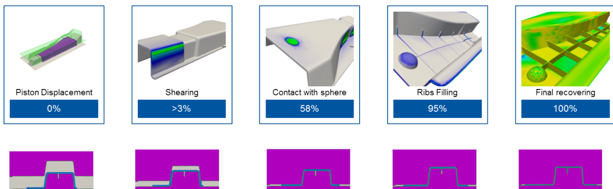
Figure 4.28: Molding Compression - Dedicated mold
