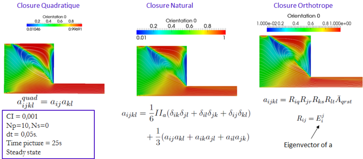
Figure F.2: Closure approximation effect on fiber orientation response.
