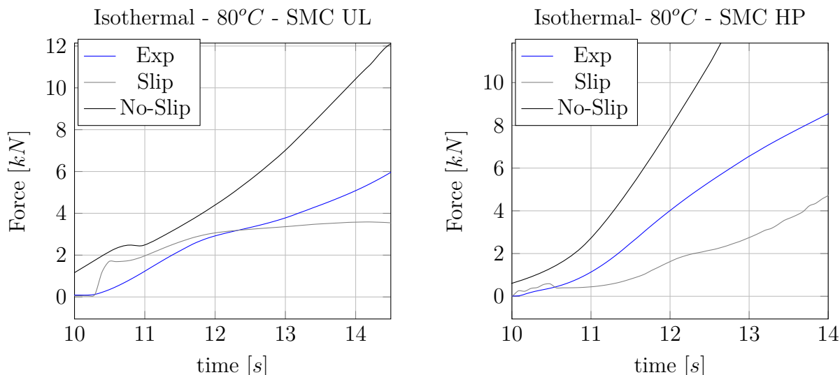
(a) Compression stress mold side lateral position for SMC UL, T=80^\circ\text{C} , h_0 = 7.27\text{mm}
