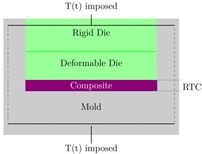
Figure 4.5: Numerical modeling of PVT- \alpha test. Imposition of temperature in the domain and thermal contact resistance (RTC).
