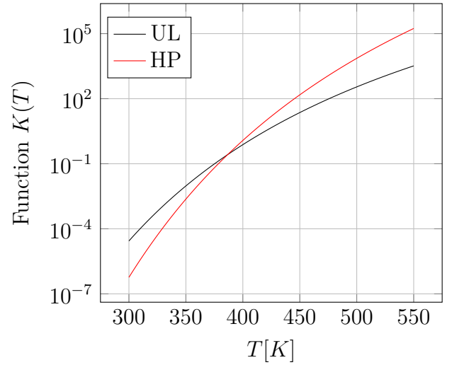
Figure 4.1: Thermo-kinetic function G(\alpha) for ultra light (UL) and high performance (HP) SMCs. Figure 4.2: Thermo-kinetic Function K(T) for ultra light (UL) and high performance (HP) SMCs.
