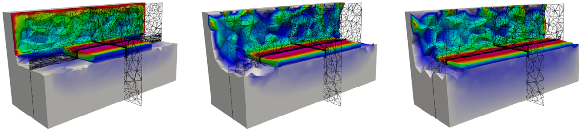
Figure 4.14: Plane strain compression velocity. SMC materials flows within a channel. Snaps of deformation for various times
