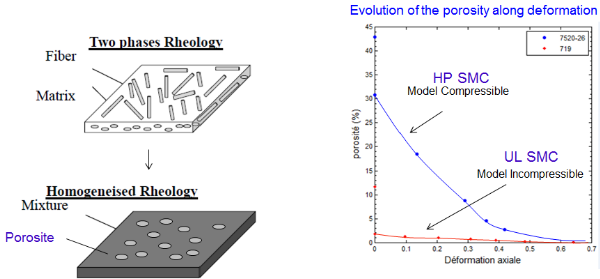
Figure 13: Evolution of the porosity as function of the equivalent deformation. High Performance SMC are compressible whereas Ultra Light one can be considered as incompressible
