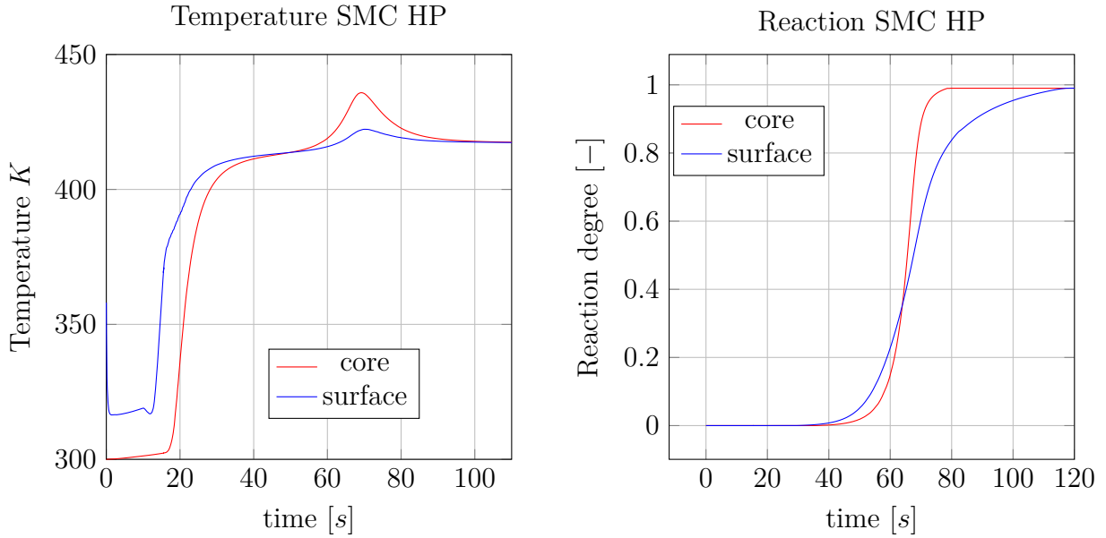
(a) Temperature evolution during compression
