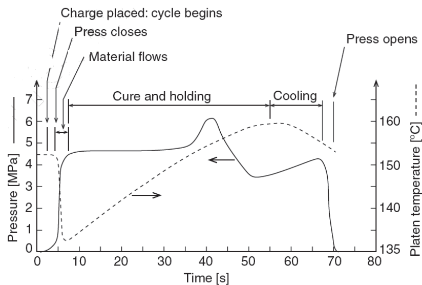
Figure 5: Temperature and pressure during a complete cycle [1]
