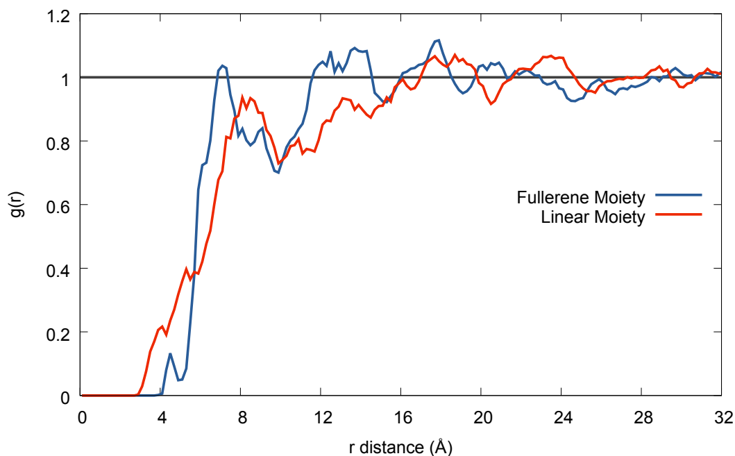
Figure 4.9 – Radial pair distribution functions for the donor (red) and acceptor (blue) moieties of DPP-Ful.
