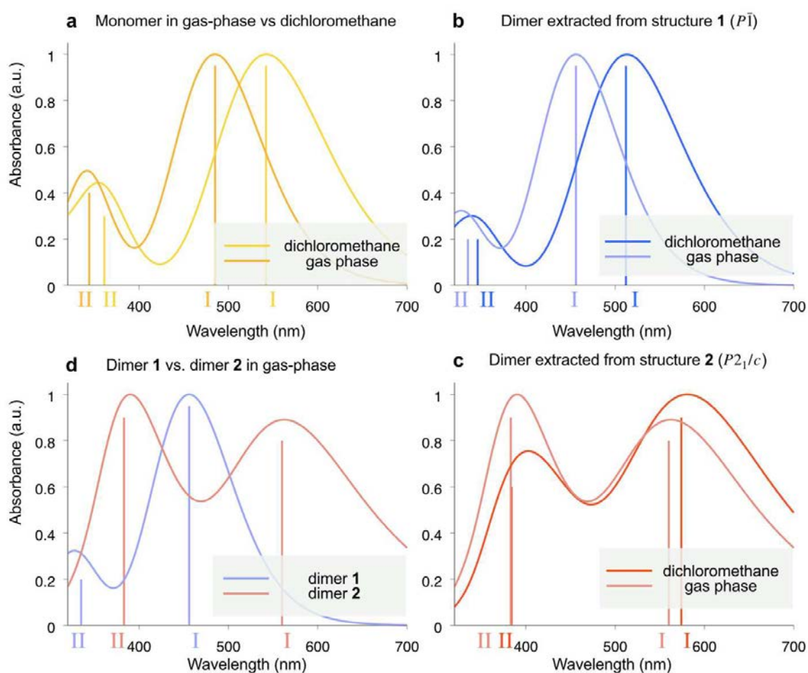
Figure 3.4 – Predicted absorption spectra for a monomer in gas phase relaxed geometry in vacuum and in dichloromethane, b dimer with geometry extracted from structure 1 in vacuum and dichloromethane, c dimer with geometry extracted from structure 2 in vacuum and dichloromethane. d shows the comparison between the two dimers in vacuum. All calculations have been performed at B3LYP/6-311+G(d,p) level of theory, solvent when included is treated according to the polarisable continuum model (PCM) 174 . Spectra are normalised according to their maximum value.
