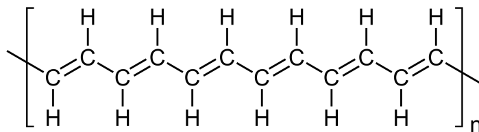
Figure 1.7 – Trans polyacetylene monomeric unit with the alternating double-single bond structure in evidence.
