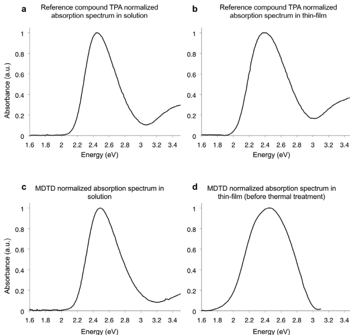
Figure 3.7 – Normalised experimental absorption signals taken from ref. 156 . Panel a&b report the spectra for the reference compound triphenylamine from which MDTD is derived. TPA and MDTD performances are compared in ref. 156 . As already remarked, the similarity between the solution and thin film spectra suggests a low degree of crystallinity of TPA thin films. Panel c&d show the spectra for MDTD in solution and in thin film conditions before thermal treatment (used in the second constrained fit). All reported spectra are transformed in absorbance vs energy (eV) to appropriately visualise the broadening.
