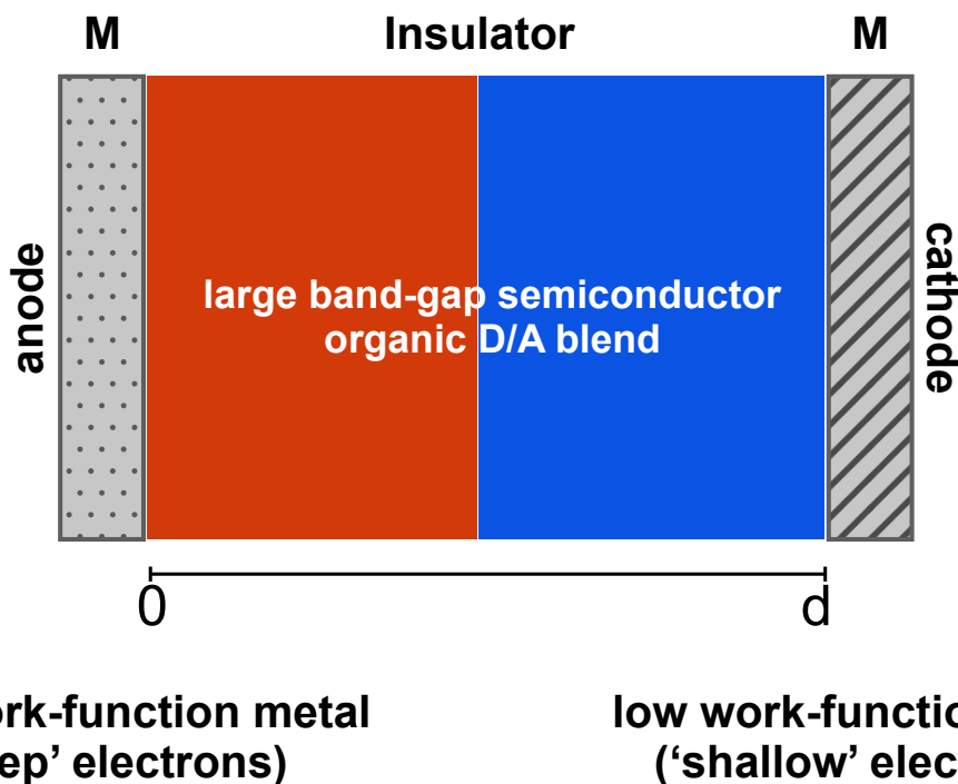
Figure 1.6 – Schematic depiction of a MIM junction that best captures the general working principle of an organic solar cell. The left electrode is the anode while the right electrode is the cathode.
