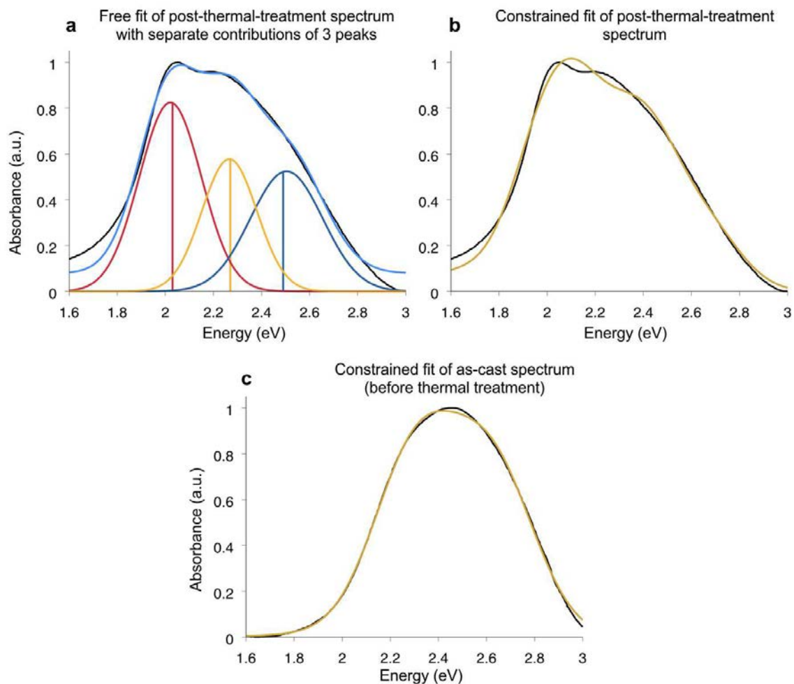
Figure 3.6 – Plots of all the performed fits to the available experimental signals (black solid lines). Panel a reports the free fit and also shows the single components identified, numerical values can be found in Table 3.4. Panels b & c show the plots of the constrained fits mixing the predicted transitions between 1.8 and 3.0 eV for all components (structure 1, 2 and amorphous). Fitted curves are reported in golden colour and, when necessary, extrapolated beyond the fitting range.
