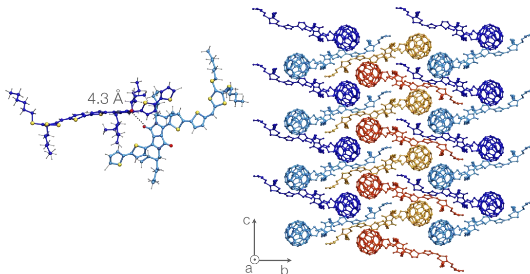
Figure 4.7 – Structural features of the polymorph 3 obtained after a full DFT optimisation: the shortest distance between for a DPP pair ( left ) and a view of the bc-plane ( right ).
