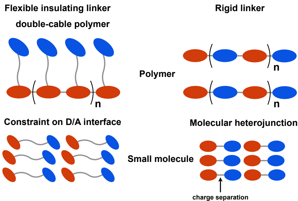
Figure 1.8 – Schematic representation of the general architecture for SMOSC materials. Depending on the character of the linker the two moieties may be combined in a single architecture with markedly different character. On the left , an insulating linker produces assembly of molecules whose phase separation is mechanically controlled by the linker while most of the other properties of donor and acceptor moieties are preserved. On the right , the corresponding structures generated from a rigid linker. Structures are more compact and the isolated properties less preserved. These architectures should be able to achieve efficient dissociation on the molecule itself and ensure transport over the morphology. The D/A interface is no longer needed to dissociate the exciton. Red elements indicate donor blocks while blue ones represent acceptor blocks.
