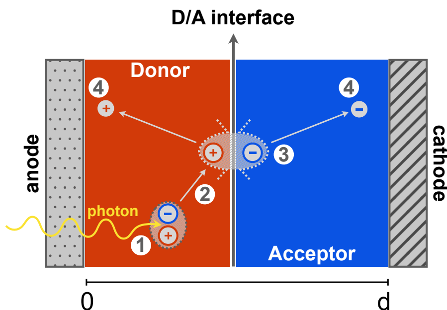
Figure 1.1 – Illustration depicting all the 4 steps in which the photovoltaic process may be divided. (1) photon absorption and exciton generation, (2) exciton diffusion and encounter with the interface (3) exciton dissociation (4) charge collection at the electrodes.
