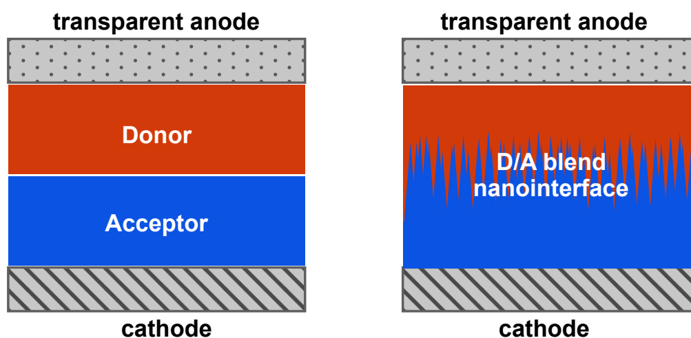
Figure 1.3 – Representations of the most common heterojunction devices for donor and acceptor blends. The planar heterojunction ( left ) with layers stacked one upon the other and an ideally planar interface. The bulk heterojunction ( right ) with a structured interface diffuse over the whole volume of the layer.
