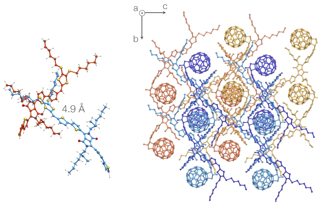
Figure 4.8 – Structural features of the polymorph 4 obtained after a full DFT optimisation: the shortest distance between for a DPP pair ( left ) and a view of the bc-plane ( right ).
