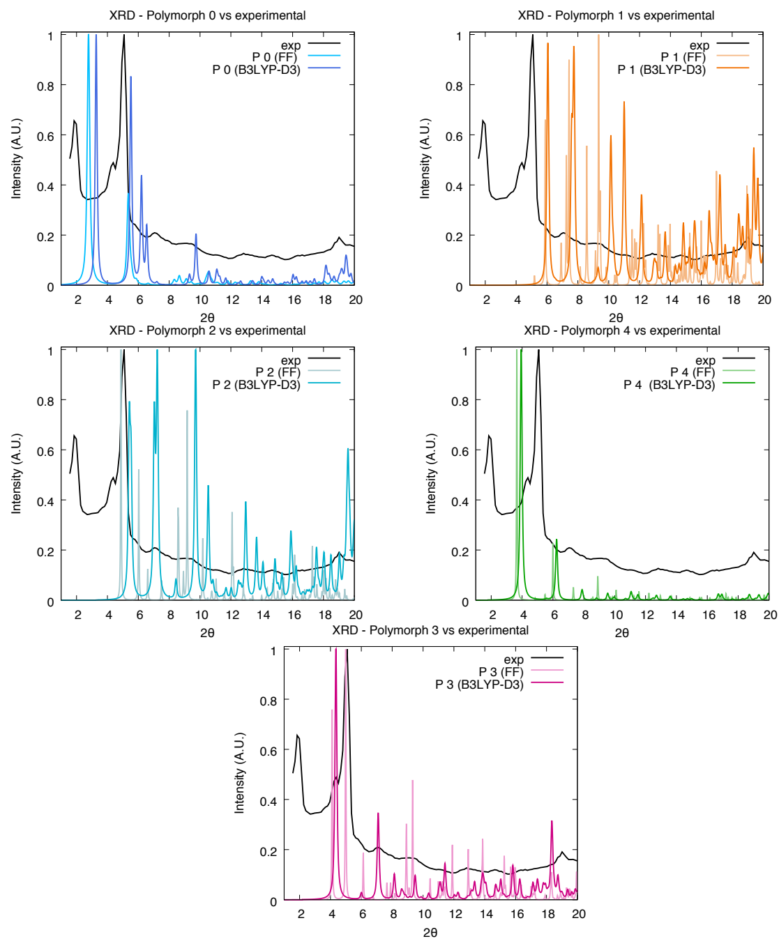
Figure 4.4 – XRD patterns for all the considered polymorphs. The two superimposed spectra have been obtained from the force-field structure (FF) and the B3LYP-D3 refinement.
