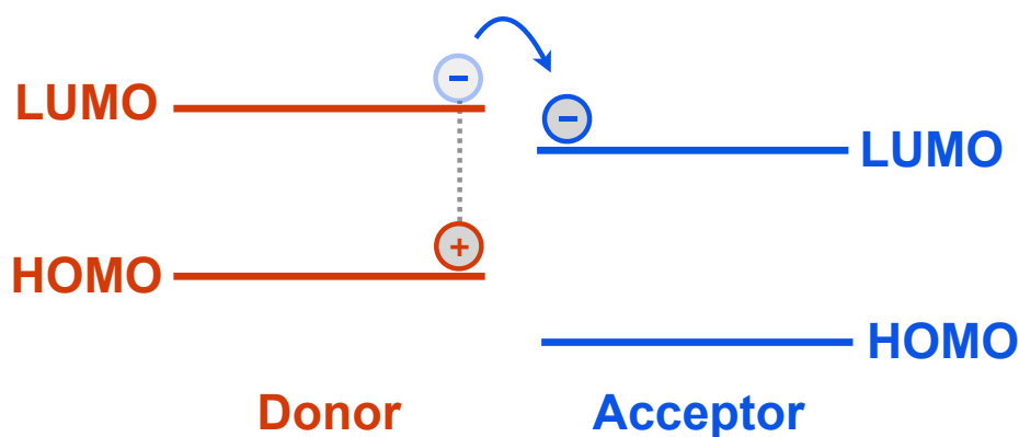
Figure 1.2 – Matching of the energy levels at the donor acceptor interface that ensure the dissociation of the exciton into free charges. This is valid for both planar and bulk heterojunction. Any neighbouring pair of a donor and an acceptor may realise the exchange according to this scheme.
