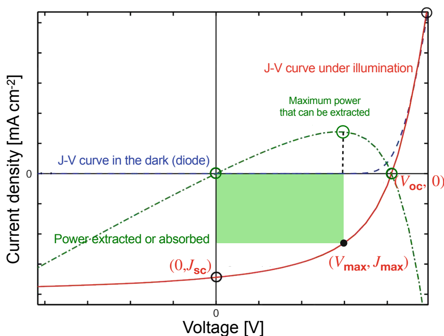
Figure 1.5 – Plot of a typical J-V curve, the green rectangle represents the fill factor FF.
