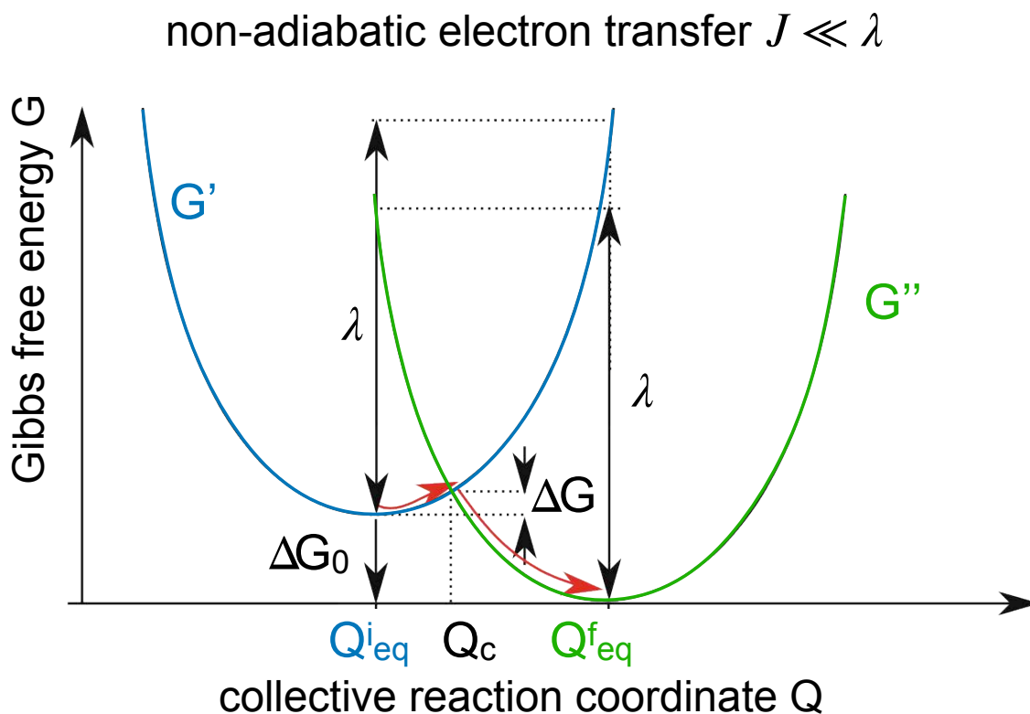
Figure 2.2 – Depiction of the energy surfaces responsible for the “hopping” in the non-adiabatic regime of charge transfer. The interaction between the two states, i.e. the two molecules, is assumed sufficiently small as to leave the energy surfaces unchanged. Red arrows indicate the oscillations needed for the transfer between the two equilibrium positions. The transition can only happen at Q_c since the energy cannot change (the energy value is fixed) and the Frank-Condon approximation imposes that the nuclear configurations are the same ( Q value is fixed).
