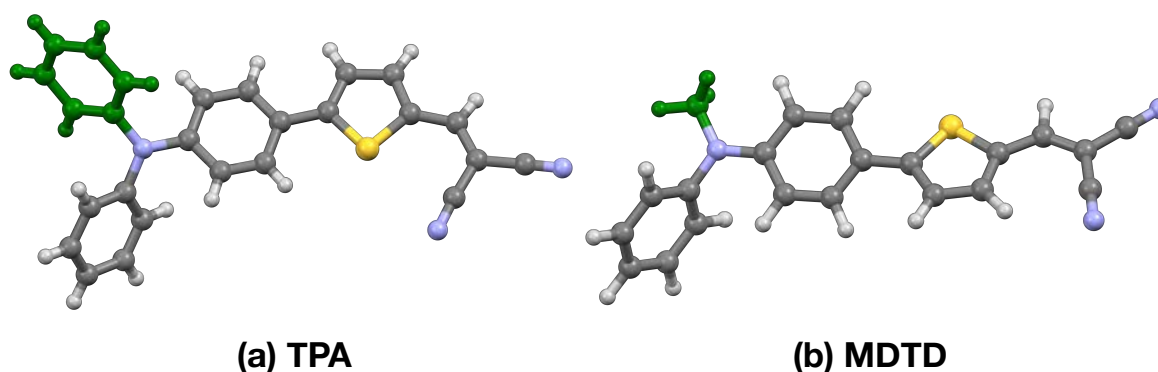
Figure 3.1 – Molecular representations of TPA ( left ) and MDTD ( right ) with the residues involved in the substitution depicted in green.
