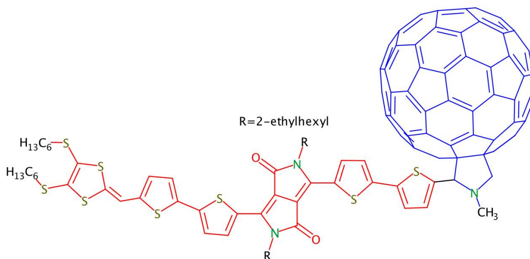
Figure 4.1 – Chemical structure of DPP-Ful with [60]-fulleropyrrolidine (Ful) acceptor moiety in blue and the diathiafulvalene-functionalised diketopyrrolopyrrole (DPP) donor moiety in red.
