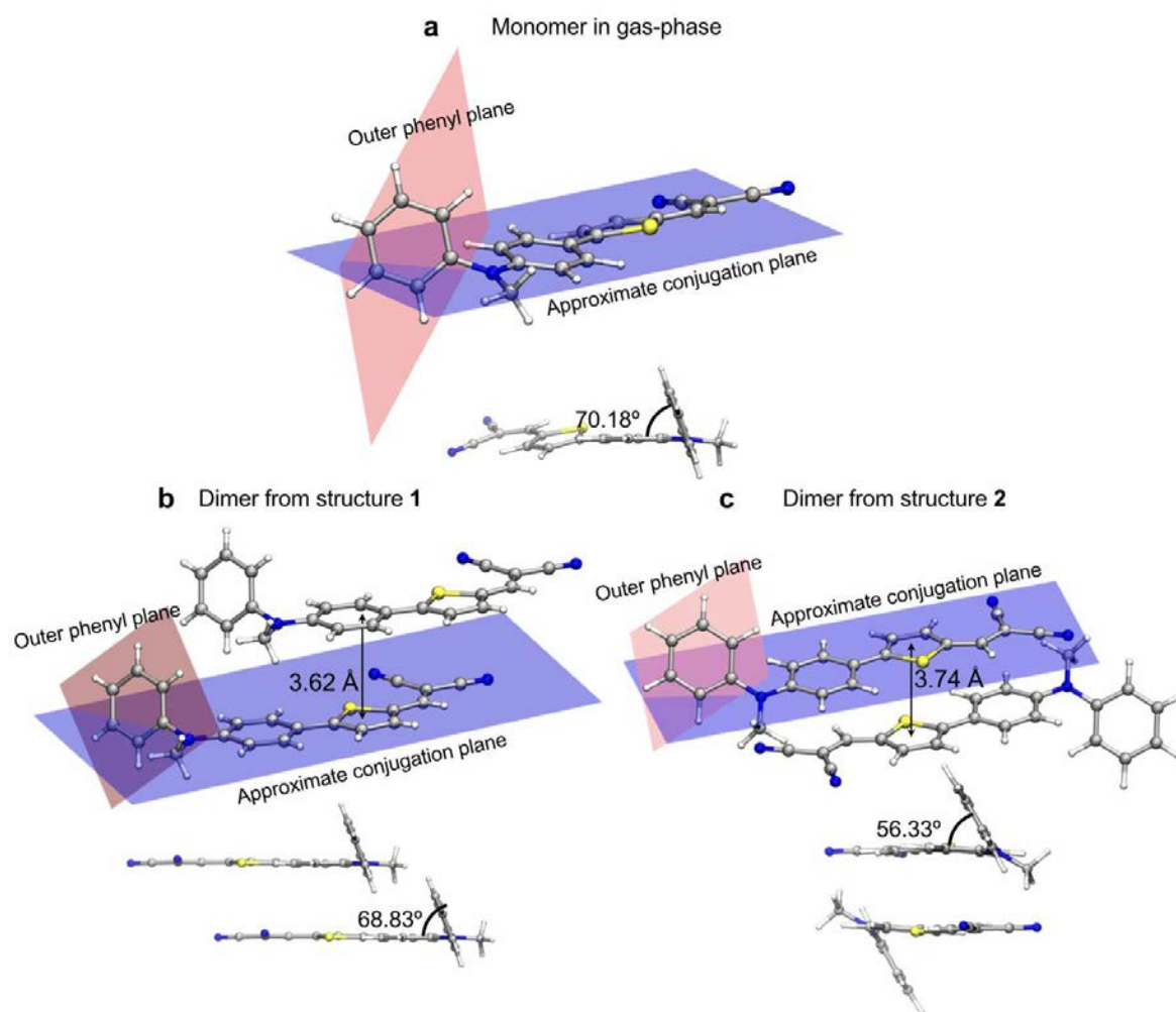
Figure 3.3 – Molecular representation of the monomer geometry relaxed in gas phase a, and the dimers issued from structure 1 and structure 2, b & c. For each geometry the angle between the plane of the external phenyl ring and the conjugation plane is highlighted. All calculations have been performed at B3LYP/6-311+G(d,p) level of theory.
