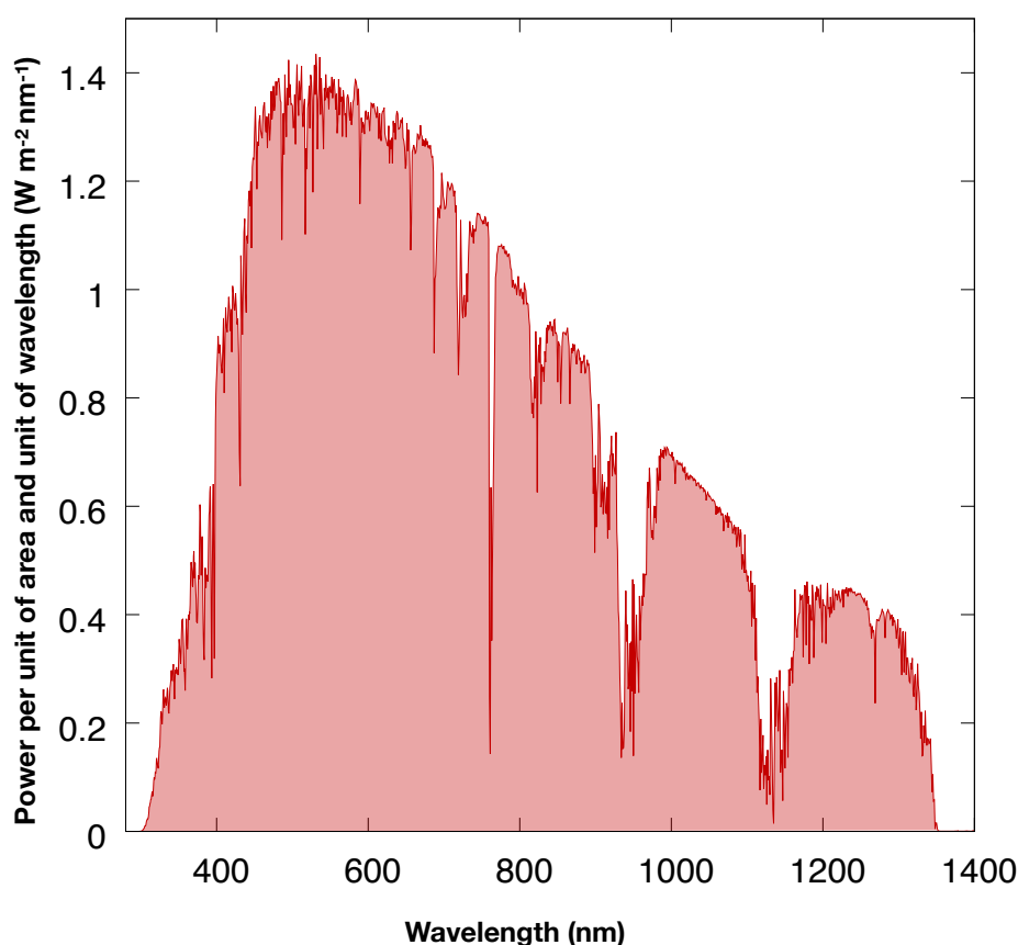
Figure 1.4 – Sun spectrum after being filtered by an air mass equivalent to the atmosphere crossed by rays at 48.2^\circ of zenith angle. Conventionally this condition is referred to as “solar spectrum AM 1.5”.
