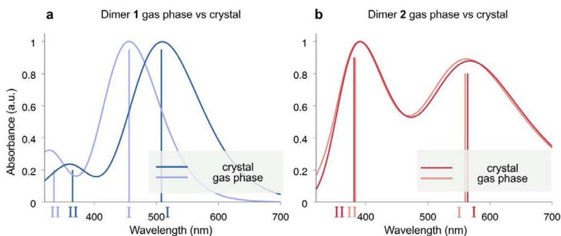
Figure 3.5 – Predicted absorption spectra for a dimer 1 in the geometry found in crystal structure 1, b dimer 2 in the geometry found in crystal structure 2, both computed in vacuum and in the presence of the embedding charges. Transition with largest oscillator strengths are indicated with a vertical bar. All spectra are normalised.
