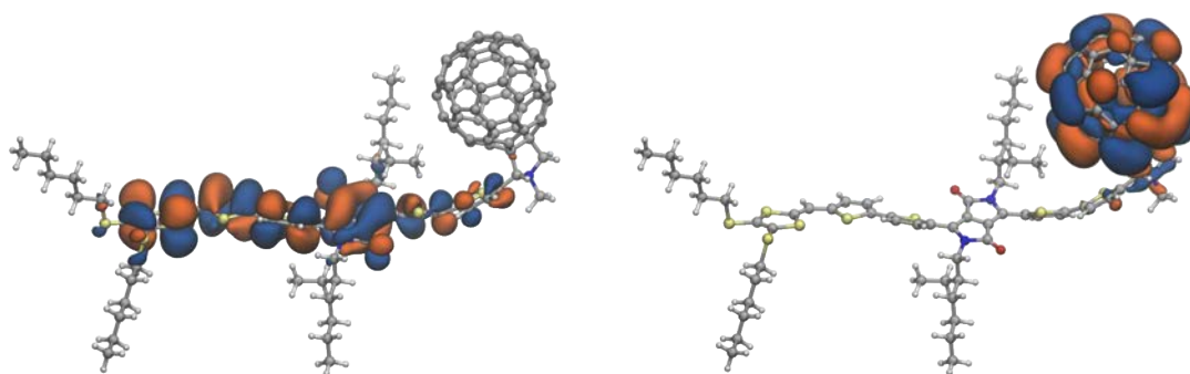
Figure 4.2 – Isosurface (values \pm 0.005 ) representation of frontier orbitals. (left, HOMO; right, LUMO).
