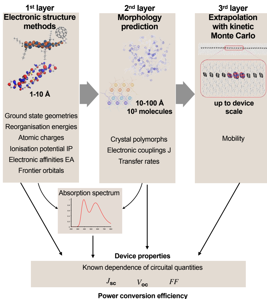
Figure 2.3 – Scheme summarising the adopted protocol. Electronic structure methods are employed to generate accurate information on the orbital energies, geometries and charge distributions of the molecules, this is the first layer of computational methods employed. The next layer combines the information coming from the previous one (atomic charges, geometry, ...) to compute the most plausible packings of molecular assemblies, ordered or disordered, on the basis of electrostatic and dispersion interactions. This information can be used to refine electronic structure calculations by including details about the local molecular environment (absorption spectra) and can be also passed to the third layer. Kinetic Monte Carlo methods are used to extrapolate the information generated in the second layer and simulate processes happening at larger scales (charge transport). All data from the three layers can be used to give a general assessment of photovoltaic performance. A preliminary assessment can be given based on the estimates of relevant quantities: HOMO and LUMO, absorption spectrum, charge mobility. Quantitative assessment can also be foreseen by using the empirical relations that have been derived to link these quantities to the circuital quantities characterising a solar device, J_{sc} , V_{oc} and FF and ultimately give an estimate of the PCE.
