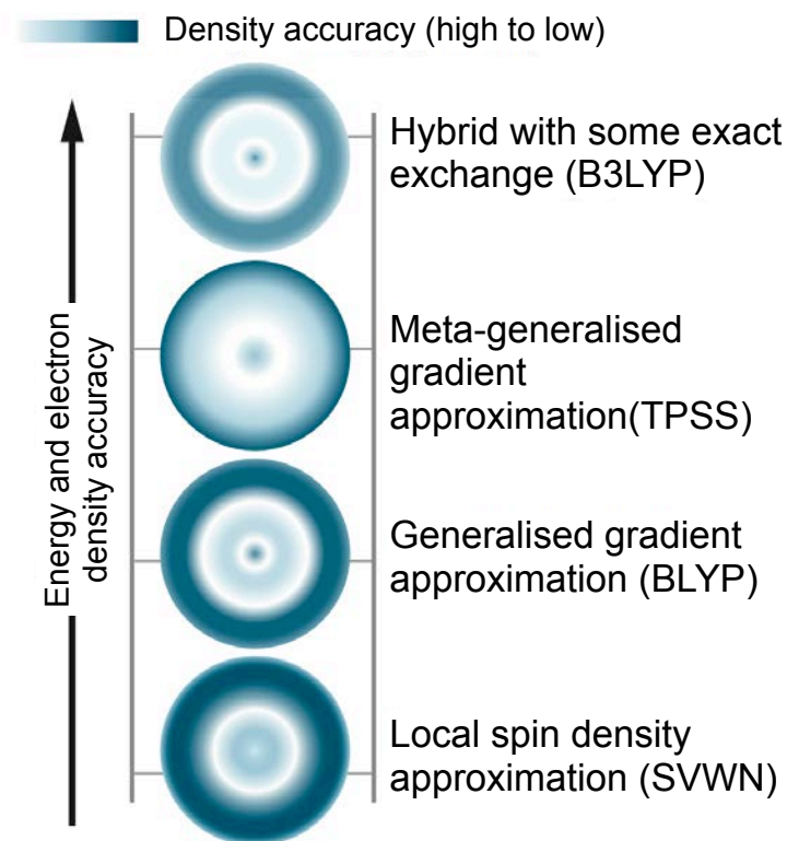
Figure 2.1 – Graphical representation of the Jacob's ladder of chemical accuracy [108] adapted from ref. [113] . For each rung in the ladder an indication of the accuracy is given according to the heat map shown. In addition, an example of a DFT approach corresponding to each rung is given.
