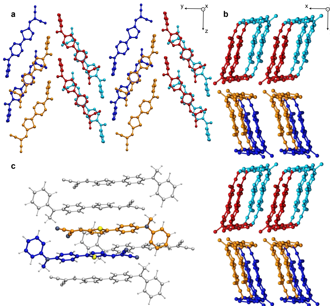
Figure 3.9 – Representations of a 2 \times 2 \times 2 supercell of structure 1. Panel a shows the bc crystal plane with the four molecules transformed according to the space group elements in red, blue, cyan and orange. Panel b shows the stacking of the structure formed across bc in the a direction, that corresponds to x. Panel c features the group of neighbours considered for hole transport when the carrier is localised on the orange molecule.
