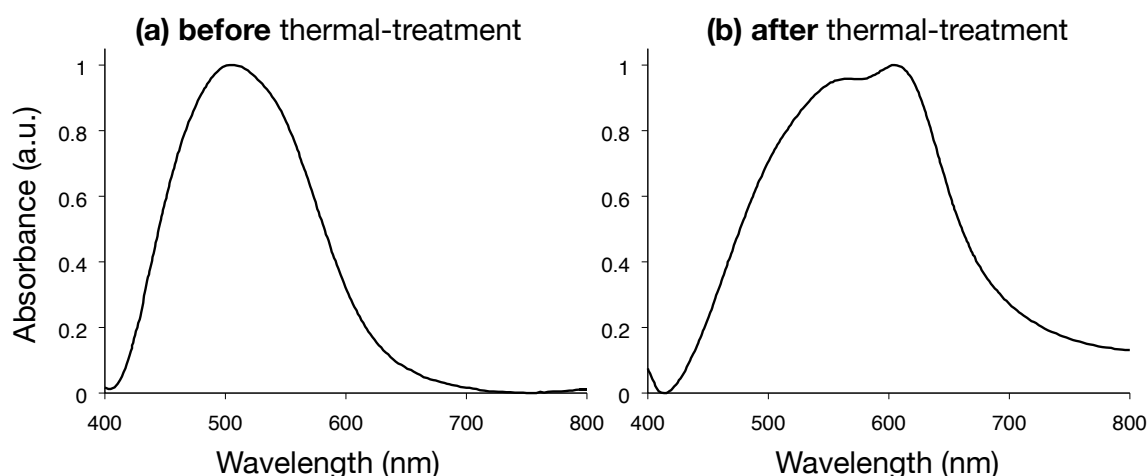
Figure 3.2 – Experimentally measured absorption spectra for the thin film as-cast ( left ) and for the thin film after thermal treatment ( right ).
