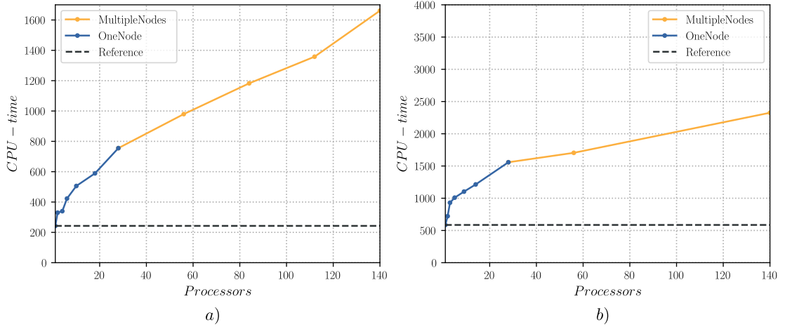
Figure 4.28: CPU-times at the end of the simulation for the test with a DSPP of: a) 2 \text{ mm}^2 and b) 4 \text{ mm}^2 per core.
