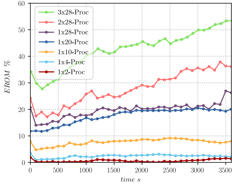
Figure 4.15: Range of the number of elements over the Mean number of elements per core (index EROM ) for the test with a surface of 50 \text{ mm}^2 performed in 10, 20, 28, 56 ( 2 \times 28 ) and 84 ( 3 \times 28 ) cores. The percent value increases with the number of cores plotted every 10 increments.
