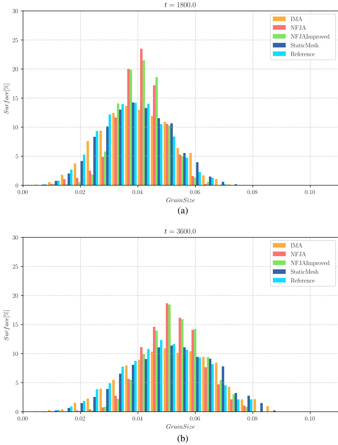
Figure 2.30: Grain size distributions weighted by surface for the different models and for a mesh size h = 0.004 . (a) state at time t = 1800 , (b) state at time t = 3600
