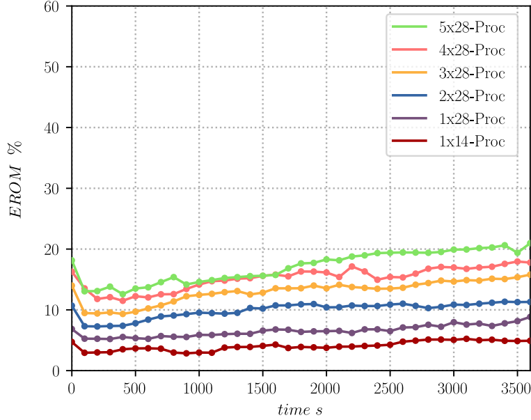
Figure 4.20: Range of the number of elements over the Mean number of elements per core (index EROM ) for the test with 560 \text{ mm}^2 of surface performed in 14, 28, 56 (2x28), 84 (3x28), 112 (4x28) and 140 (5x28) cores. The percent value increases with the number of cores plotted every 10 increments.
