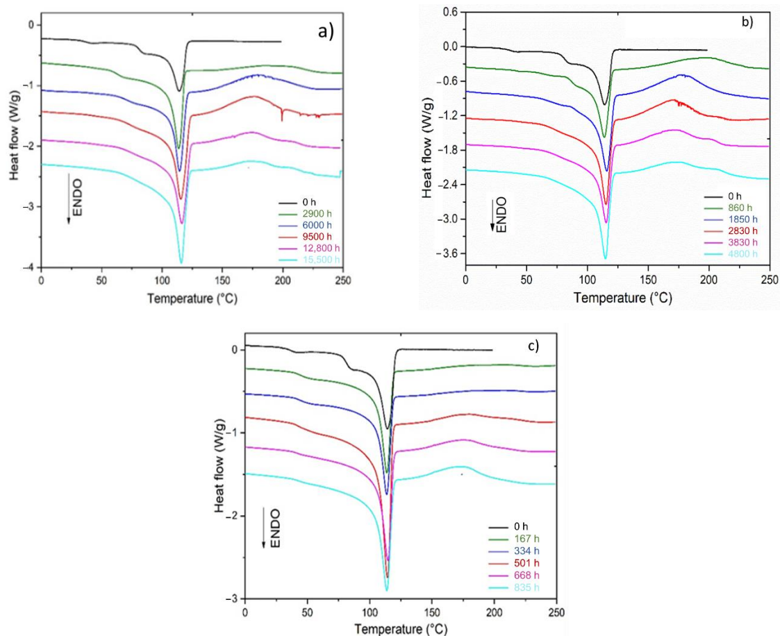
Figure 98. DSC thermograms of Si-XLPE before and after its radio-thermal ageing in air under (a) 8.5 \text{ Gy}\cdot\text{h}^{-1} at 47^\circ\text{C} , (b) 77.8 \text{ Gy}\cdot\text{h}^{-1} at 47^\circ\text{C} , and (c) 400 \text{ Gy}\cdot\text{h}^{-1} at 21^\circ\text{C} .
