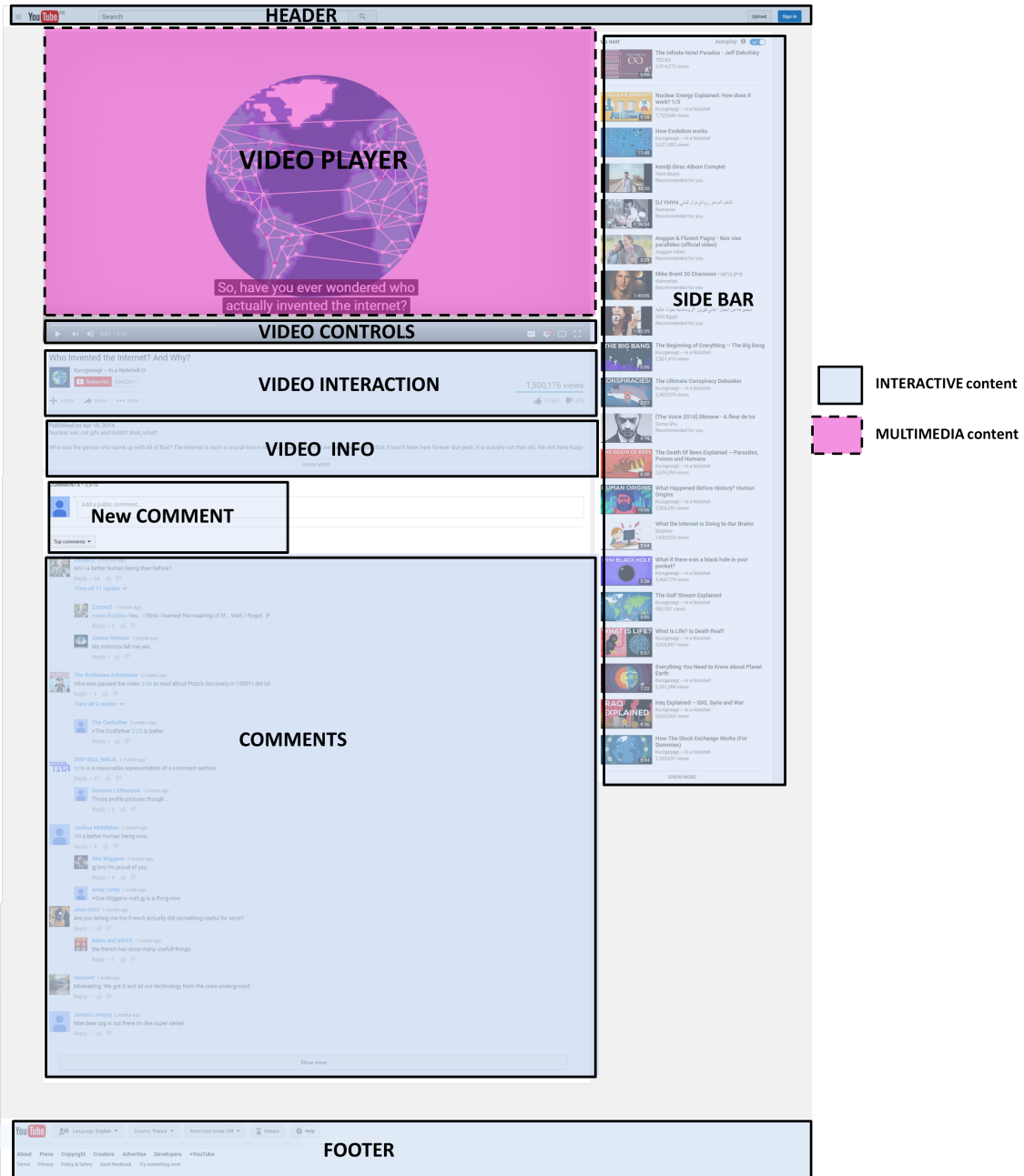
Figure 4-12: Segmentation results on a YouTube page: MSoS with pG = 0.31 and 0.36
