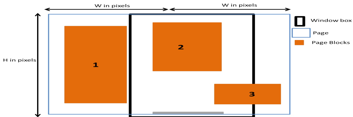
Figure 5-12: Doing horizontal scrolling to see block 2
