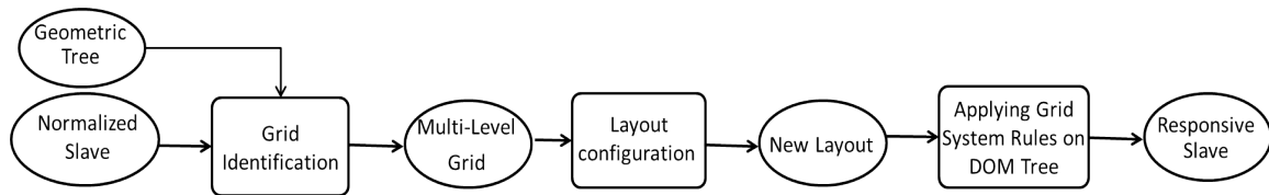
Figure 5-8: Building blocks for making the responsive re-design on the Slave
