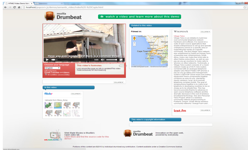
Figure 6-2: Main Application
