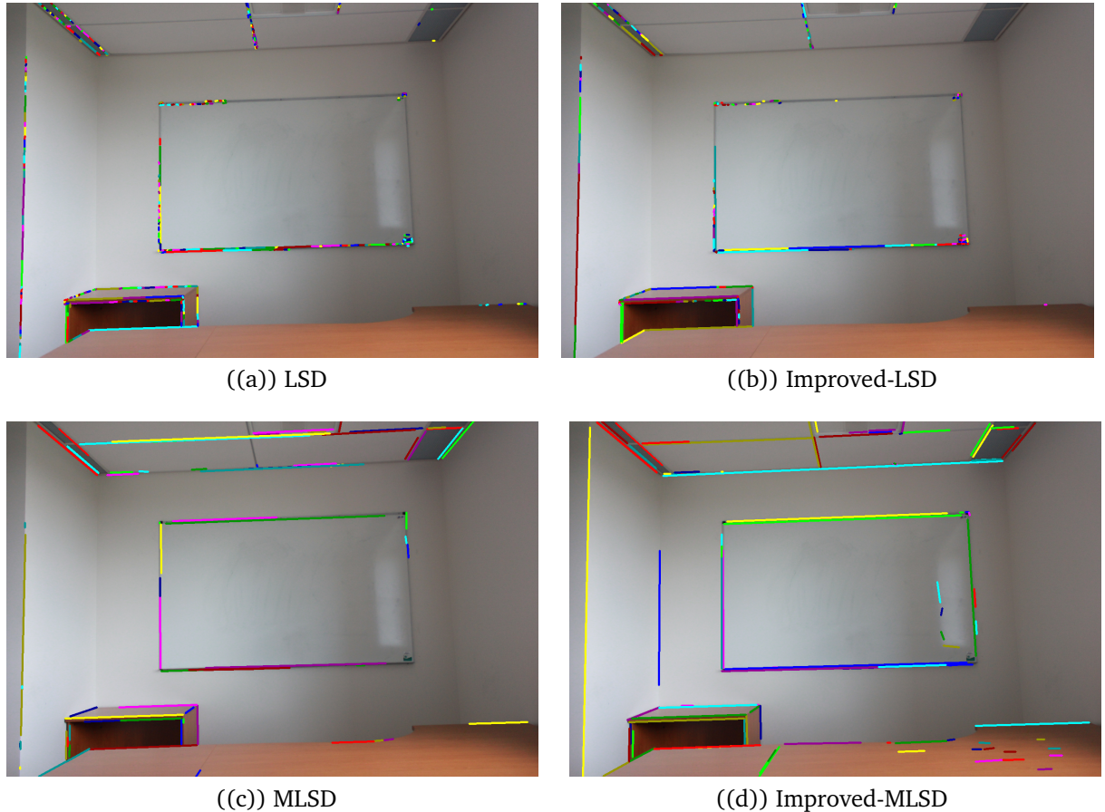
Figure B.5: Comparison between the performance of LSD and MLSD before and after improvement on a big size image
