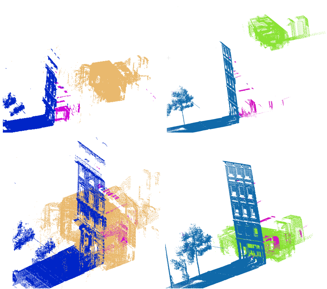
Figure 4.9: Result of the test of our algorithm on two pairs of indoor/outdoor scans, Top: the initial position of each pair, Bottom: The position of each pair after registration, pink points represent the indoor points detected from the outdoor scans.
