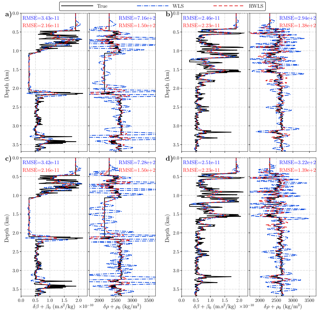
Figure 5.20: The final inverted parameters corresponding to the (a,b) noiseless and (c,d) noisy 2004 BP salt model. Inverted \delta\beta + \beta_0 and \delta\rho + \rho_0 for (a,c) x = 3.8 km and (b,d) x = 7.0 km.
