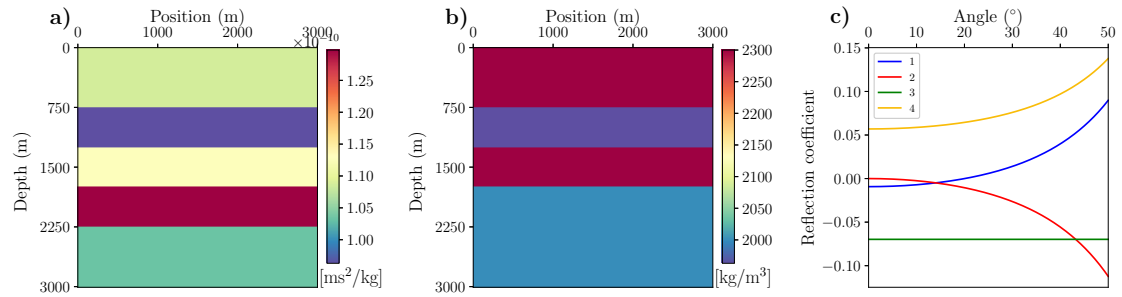
Figure 3.7: Exact a) \beta , b) \rho and c) reflection coefficient as a function of angle for each interface corresponding to model 1.
