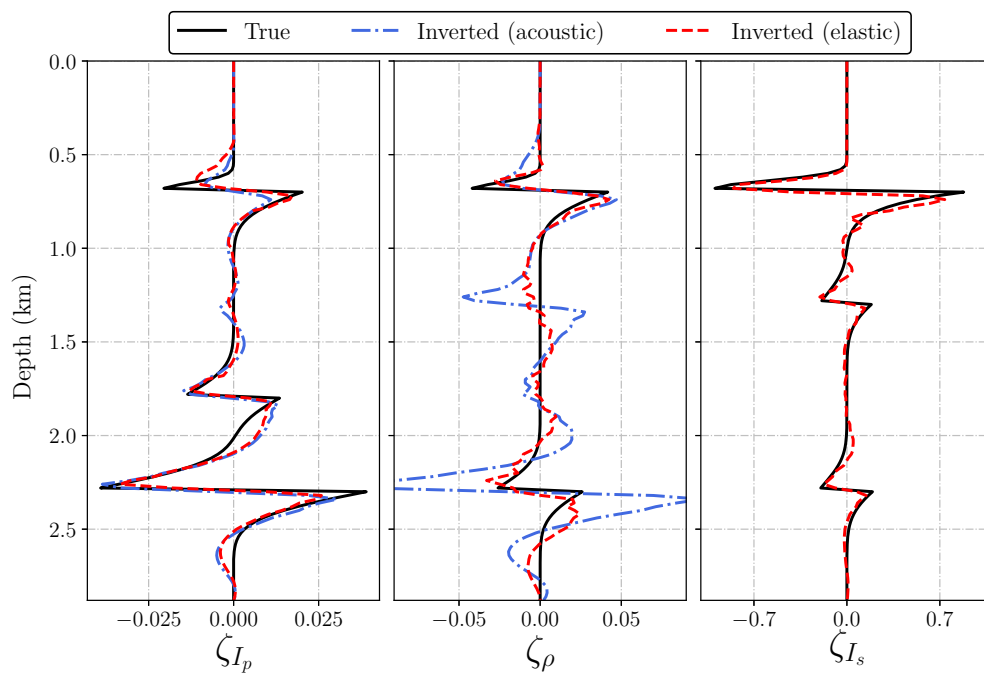
Figure 4.8: Vertical logs extracted at x = 3.4 km (Figure 4.7) comparing the true models (black) and estimated ones using acoustic WLS (blue) and elastic WLS (red). The blue line for \zeta_{I_s} is not displayed as it is not reconstructed.
