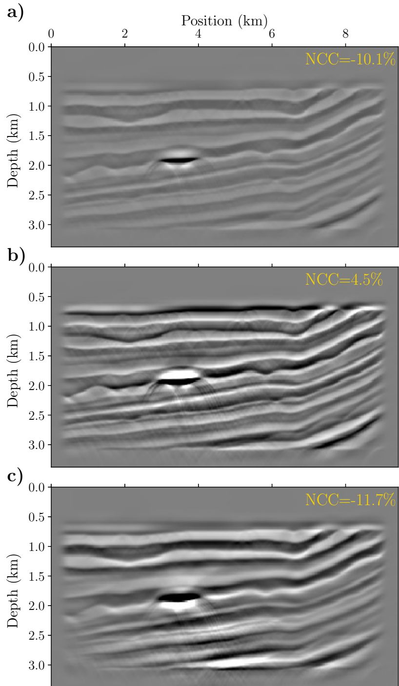
Figure 4.16: Same as Figure 4.12, but for inaccurate P-wave velocity background model (8% error): inverted a) \zeta_{I_p} , b) \zeta_{I_s} and c) \zeta_{\rho} . Inverted model are plotted in the same scale as the exact models.
