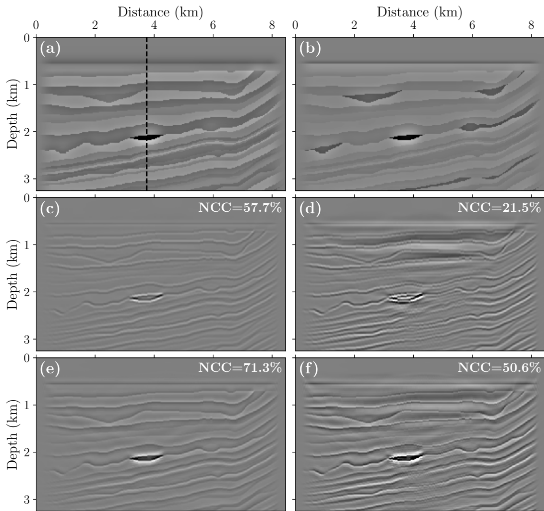
Figure 6.10: The exact model perturbations a) \zeta_{I_p} and b) \zeta_\rho , and inverted c) \zeta_{I_p} and d) \zeta_\rho via 40 iterations of CG-LSRTM, inverted e) \zeta_{I_p} and f) \zeta_\rho via 15 iterations of PCG-LSRTM. Each inverted model is plotted with the same scale as for the exact model. The dashed line in (a) indicates the position of the extracted trace.
