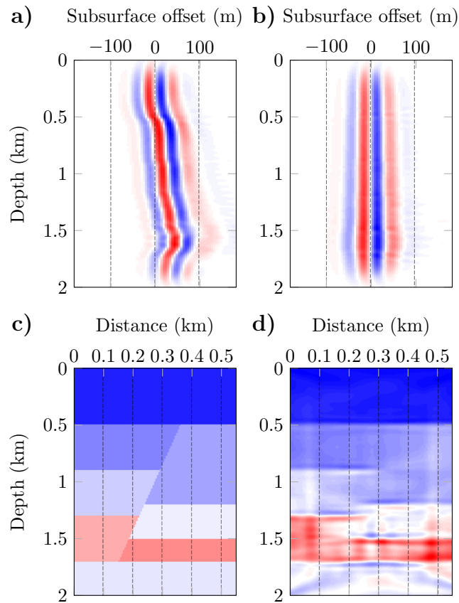
Figure 2.13: MVA cross-well configuration with the full wavefield. a) CIG in the initial homogeneous model, b) CIG in the final model, c) exact velocity model and d) inverted model. In the final model, energy is localized around h = 0 , from Lameloise and Chauris (2016) .
