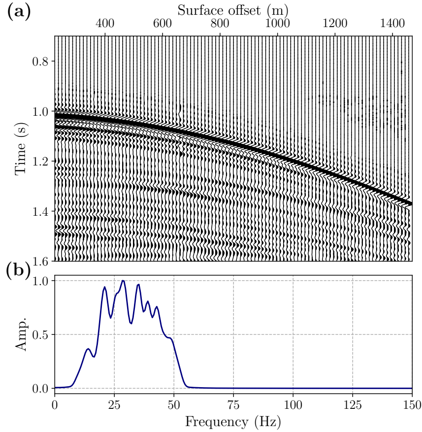
Figure 7.9: The a) shot gather and b) its spectrum after low-pass filtering with cut frequency of 45 Hz.
