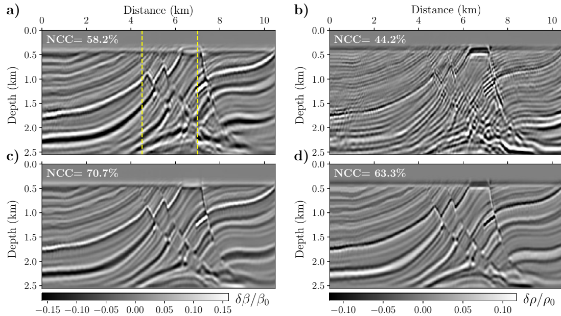
Figure 5.8: Comparison between the inverted parameters corresponding to dense shots (292 shots) for Marmousi2 model. Inverted a) \delta\beta/\beta_0 and b) \delta\rho/\rho_0 vis the WLS method, c) \delta\beta/\beta_0 and d) \delta\rho/\rho_0 via the RWLS method. The dashed lines in (a) correspond to the extracted traces.
