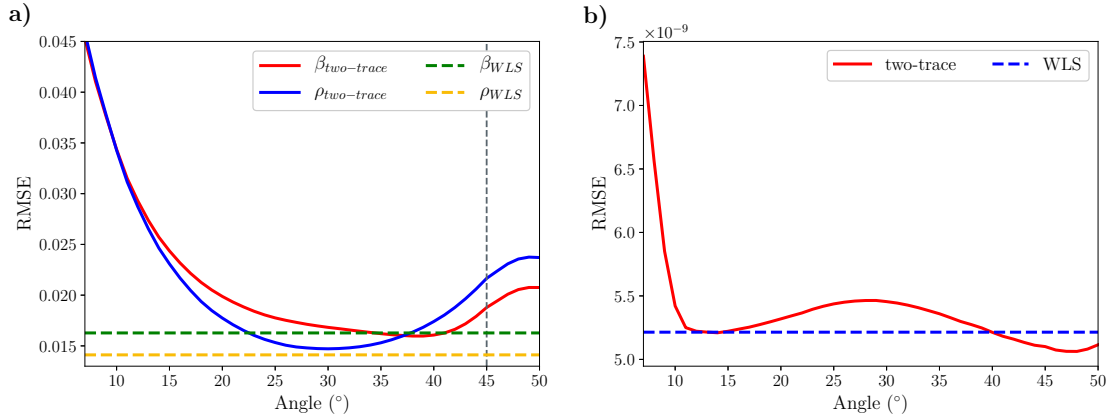
Figure 3.12: RMSE corresponding to a) inverted \beta and \rho and b) shot gathers for different angles via two-trace method comparing to WLS method. The gray dashed line in (a) corresponds to maximum available angle for the 4th event.
