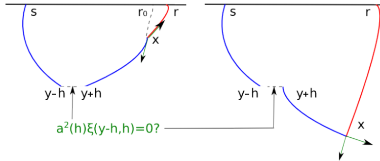
Figure 2.3: Interpretation of the tomographic gradient: a non-zero contribution is obtained when there is a \mathbf{y} position such that A_n^2(\mathbf{h})\xi(\mathbf{y} - \mathbf{h}, \mathbf{y}) \neq 0 and when there is another \mathbf{x} position along the ray joining \mathbf{y} + \mathbf{h} and a receiver position \mathbf{r} , here possibly \mathbf{r}_0 . The same holds for the source side. The second condition implies that in a smooth macro-model, the tomographic update is only above the reflector (left) and not below (right).
