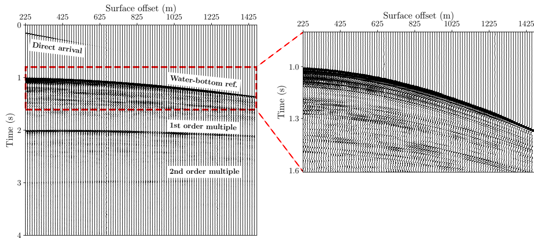
Figure 7.2: An example of observed common-shot gather.
