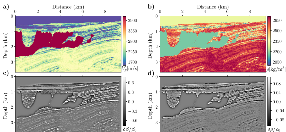
Figure 5.15: The exact a) V_p (m/s), b) \rho ( \text{kg}/\text{m}^3 ), c) \delta\beta/\beta_0 and d) \delta\rho/\rho_0 corresponding to the modified 2004 BP salt model.
