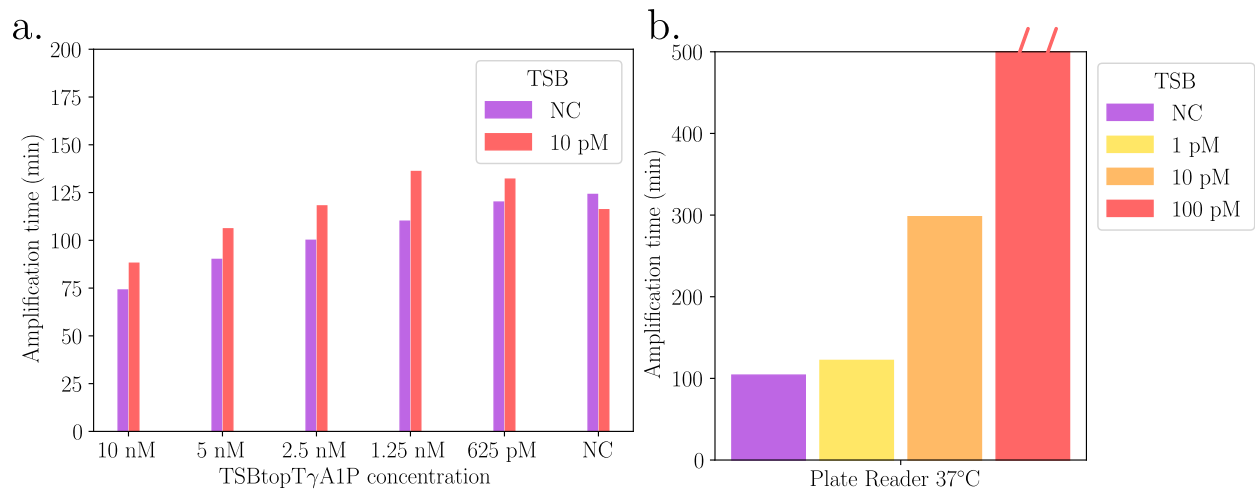
Figure 2.30: TSB-specific kT optimization for \gamma switch. a. TSB topT \gamma A1P range in presence of no and 10 pM of TSB. b. TSB range in presence of 1.25 nM of TSB topT \gamma A1P . The experiment took place in a plate reader at 37°C.
