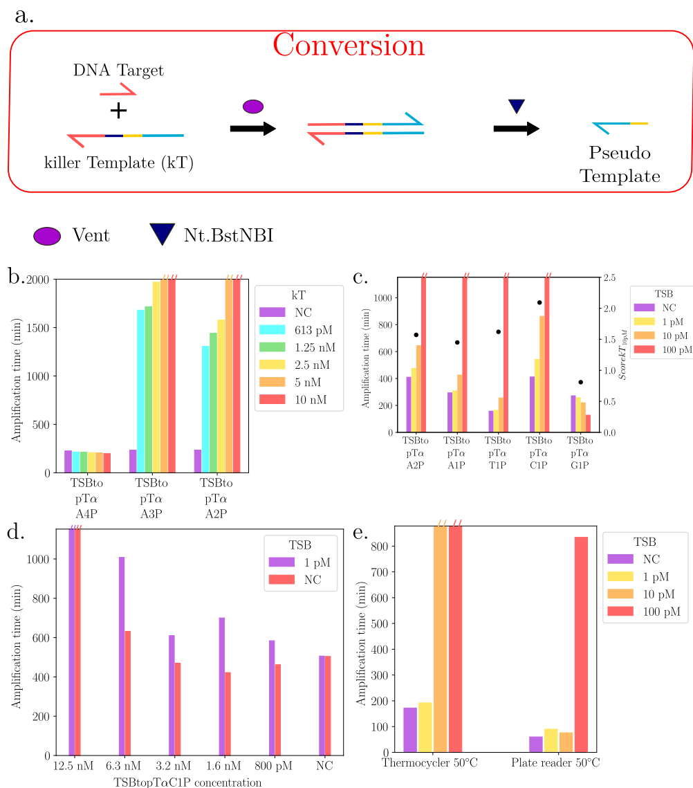
Figure 2.29: TSB-specific kT optimization for \alpha switch. a. Conversion module used for the PUMA: DNA target hybridizes to the kT and undergoes polymerization / nicking cycles, thus producing pT. b. Ranges of various kT differing in the length of the pT output in presence of 100 pM of TSB. 3 kTs have been tested, leading to pT which have respectively 2, 3 or 4 A bases at their 5' extremity. The "P" in the name of the kT indicates the presence of a phosphate at the 3' end of the kT. c. TSB ranges in presence of 2.5 nM of kT. 5 kT have been tested, leading to pT which have respectively 2 bases A, 1 base A, 1 base T, 1 one C or one base G at their 5' extremity. The amplification times for the different TSB concentrations are given by bar charts (left axis) and the scorekT_{10pM} are given by the black dots (right axis). d. TSBtopTaC1P range in presence of 0 and 1 pM of TSB. e. TSB range in presence of 1.6 nM of TSBtopTaC1P. The amplification mixtures have been split between tubes placed either in a thermocycler at 50°C or in a plate reader at 50°C.
