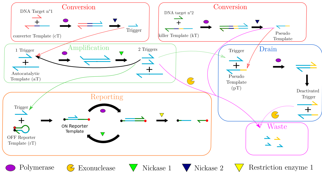
Figure 2.31: PUMA architecture for two-inputs detection: a conversion template (cT) converts the first target molecule into a universal DNA trigger; a killer template (kT) converts the second target molecule into a pseudo template; an amplification template (aT) exponentially amplifies this trigger sequence; the background noise, inherent to all exponential amplification mechanism is reduced thanks to the pseudotemplate (pT) that acts as a drain for unspecifically produced trigger strands stemming from leaky reactions; a reporting template (rT) produces a fluorescence output using trigger strands.
