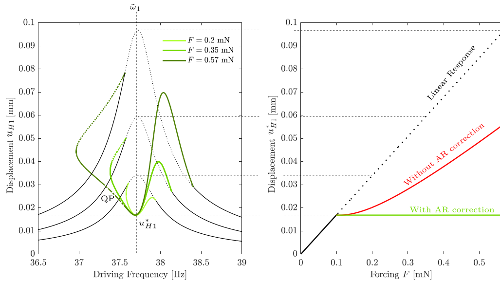
Figure 5. (a) Frequency response of the first harmonic amplitude of the beam tip displacement u_{H1} , estimated by solving system (2a) and (2b) using Manlab, for several excitation levels and with AR correction. (b) First harmonic amplitude of the beam tip displacement at the resonance frequency u_{H1}^* with respect to the excitation level, with and without AR correction. The numerical values are \beta = 0.012 and \xi_1 = 0.005 . The displacement linear response is plotted in black. The solid and dotted/dashed lines denote, respectively, the stable and unstable solutions. QP refers to a quasi-periodic response, obtained after a loss of stability due to Neimark-Sacker bifurcations.
