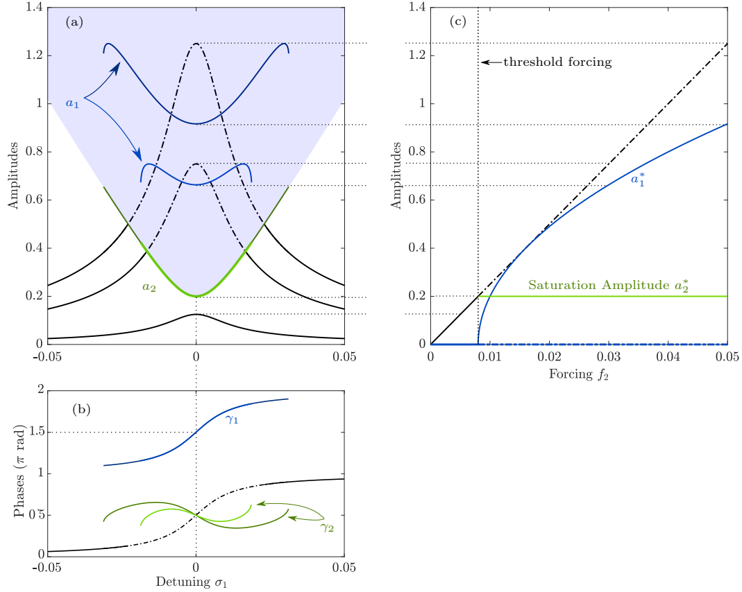
Figure 1.6: Typical response of the amplitudes a_1 and a_2 and the phases \gamma_1 and \gamma_2 by solving (1.2a,b) for \omega_2 = 2\omega_1 . The numerical values are \alpha_1 = \alpha_2 = 0.1 , \mu_1 = 0.005 , \mu_2 = 0.01 . (a) and (b) show respectively the amplitude and phase response with respect to the detuning \sigma_1 = \Omega - \omega_2 for values of the forcing f ( f \in \{0.005; 0.03; 0.05\} ). (c) amplitude response at the resonance frequency ( \sigma_1 = 0 ) with respect to the excitation level f . In the plots, the linear responses of a_2 and \gamma_2 are plotted in black. The solid and the dashed-dotted lines denote respectively the stable and the unstable solutions.
