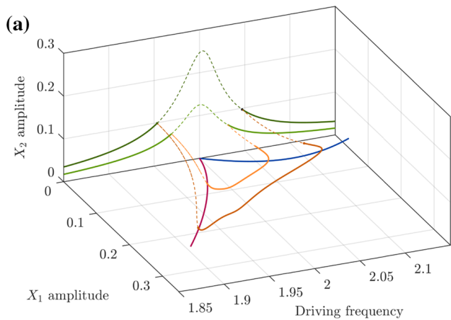
Fig. 6 Three dimensional view, in the space (\Omega, X_{11/2}, X_{21}) , of the forced response and the backbone curves, analogous to Fig. 5 with \sigma = 0 . The uncoupled and coupled forced responses are in green and orange, respectively, whereas the C+ and C- backbone curves are in blue and red, respectively.
