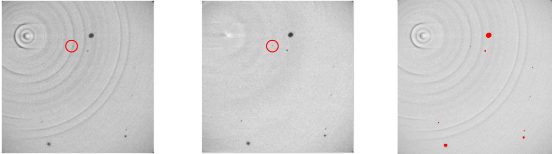
Figure 5.7: Example of image analysis: ring artifacts are removed, and defects are segmented.
