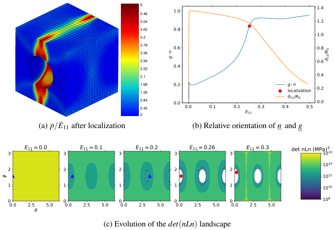
Figure 3.4: Characteristics of the localization band for the unit cell, at (T = 1, L = -1)
