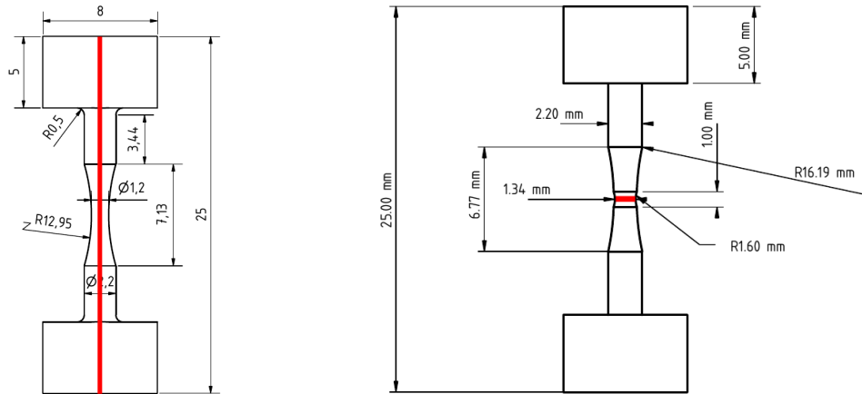
(a) Geometry I with a simple notch, with longitudinal weld joint
