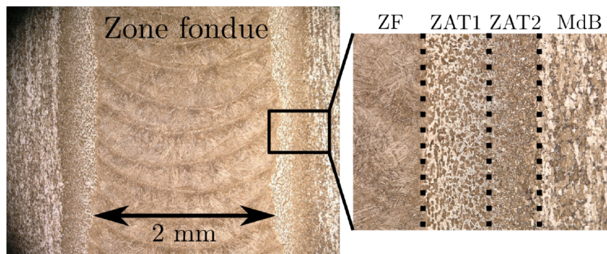
Figure 5.3: Optical micrographies of the microstructure in the weld joint. Taken from Sarre (2018)
