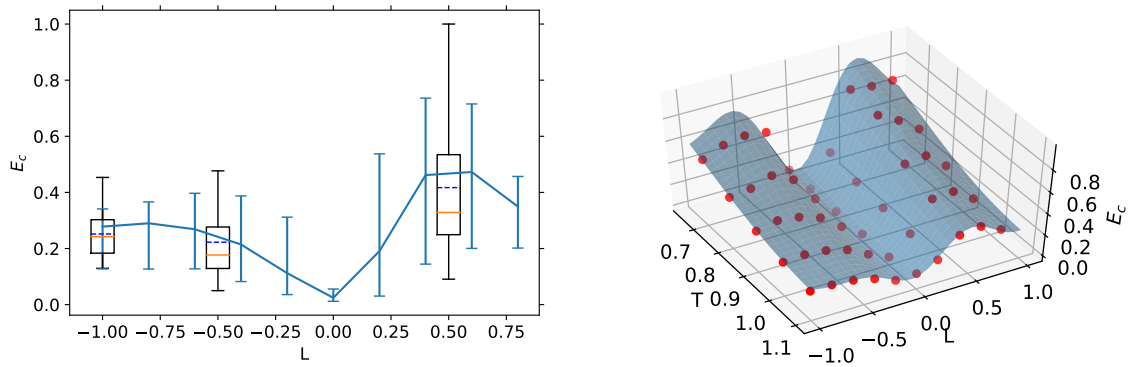
Figure 2.9: Strain at coalescence results for five different microstructures. Left: For T = 1 , evolution of the average, minimum and maximum value of E_c (over the size-5 sample) with respect to L (earlier results from 20 realizations are also plotted). Right: averaged behavior with respect to T-L interpolated using Gaussian Process Regression.
