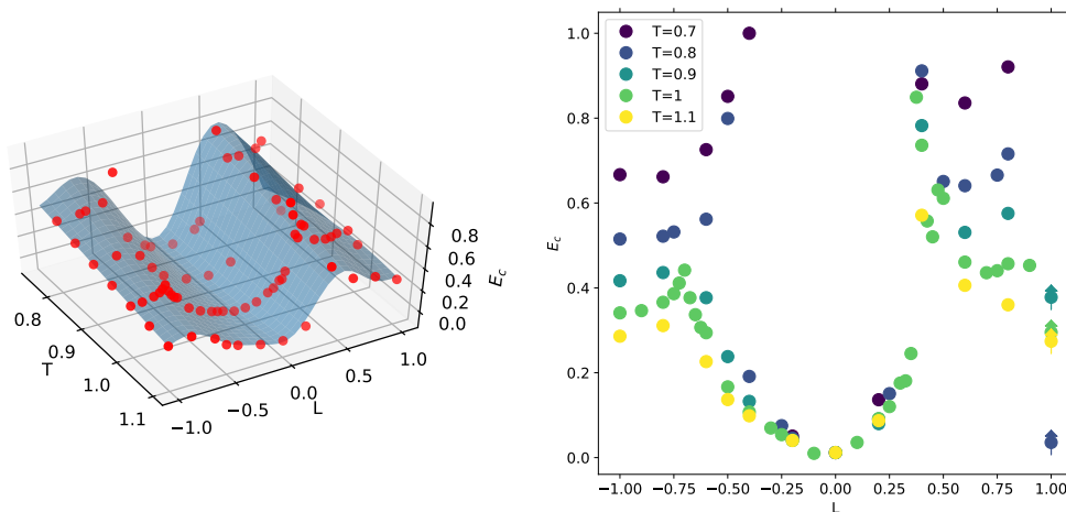
Figure 2.5: Strain at coalescence in the T - L space, for the RI microstructure. Left: Coalescence surface interpolated by Gaussian process regression for multiple loading cases (simulations shown as red points). Right: Projection of the simulation results on the L - E_c plane.
