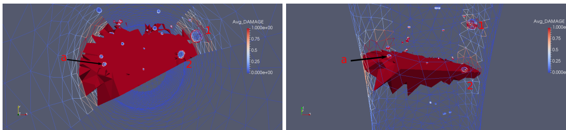
(a) Two different views of the simulated fracture surface. Some elements are cut so as to show more clearly the defects participating in fracture.
