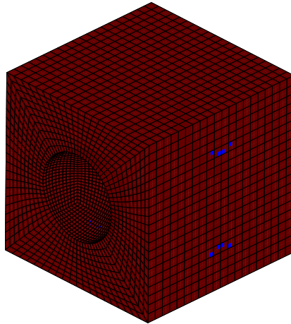
Figure 3.24: Local analysis of the loss of ellipticity for a unit cell with a diagonal loading T = 1 , L = 0 . The sign of \det(\underline{n}\mathcal{L}\underline{n}) is represented (light blue for negative values and dark red for positive values) at the onset of macroscopic localization (Fig. 3.5a)
