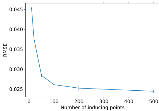
(b) Number of inducing points: test score
