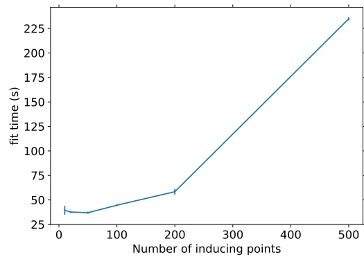
(c) Number of inducing points: fit time
