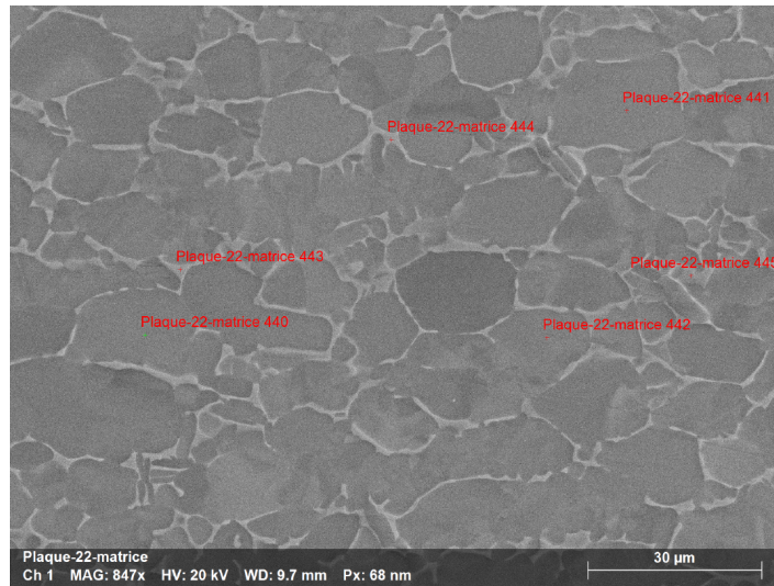
Figure 5.1: SEM micrograph of base metal, taken from Sarre (2018). The microstructure is made of equiaxial \alpha grains surrounded by a fine contour made of \beta phase (in light grey).
