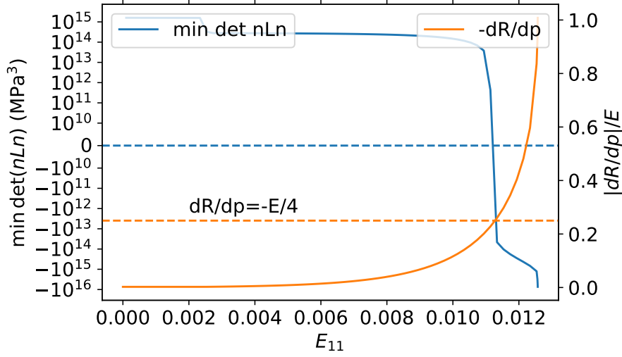
Figure 3.21: Verification of the -\mathcal{E}/4 theoretical localization result on a homogeneous cube: for a von Mises material with softening R(p) , the localization takes place when dR/dp = -\mathcal{E}/4
