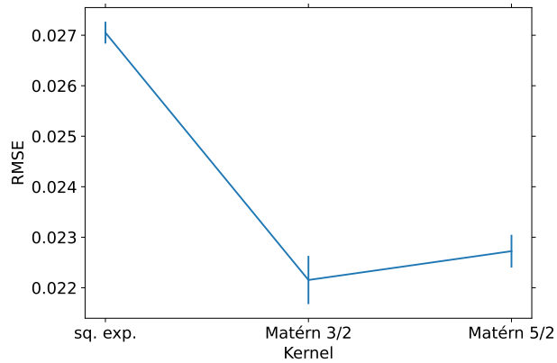
(a) Kernel: test score
