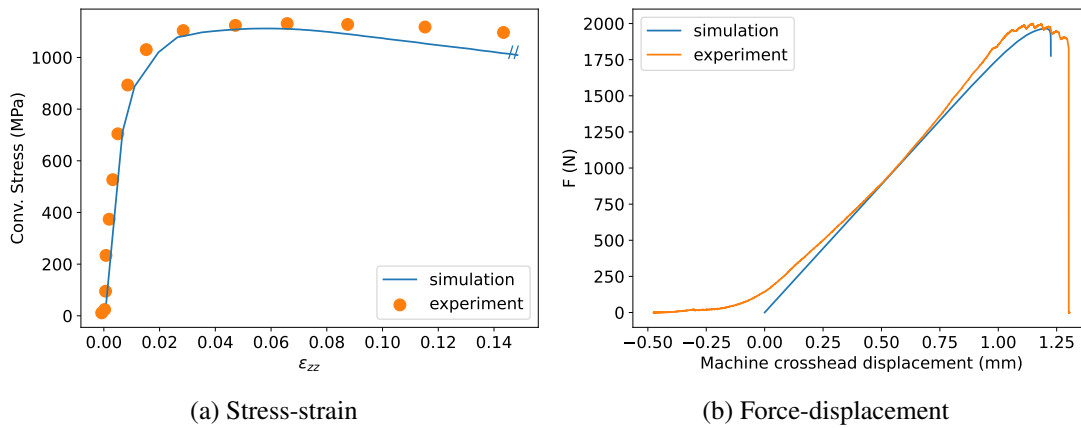
Figure 5.27: Comparison of experimental and simulation results for the EPF4 specimen. The void-free mesh with a spring is used for the simulation.
