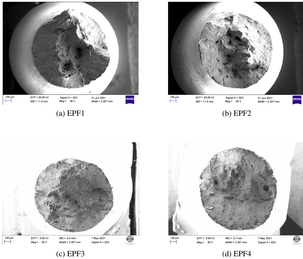
Figure 5.16: Fracture surfaces for specimens with longitudinal weld joints. The fusion zone with weld pores is visible in the center.
