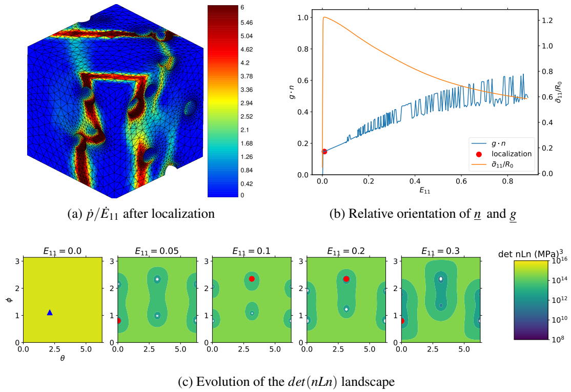
Figure 3.8: Characteristics of the localization band for the random cell R1, at (T = 1, L = 0)
