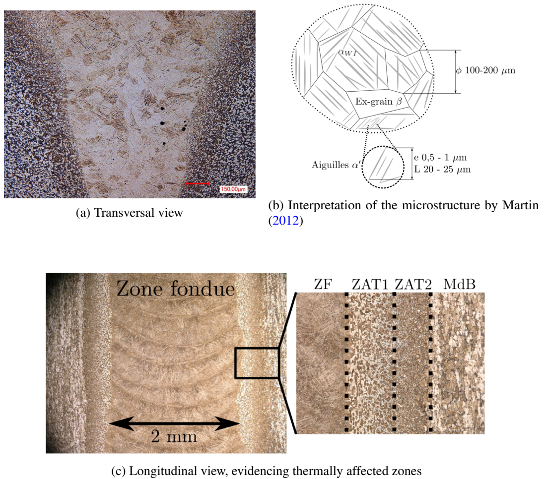
Figure 5.3: Optical micrographies of the microstructure in the weld joint. Taken from Sarre (2018)
