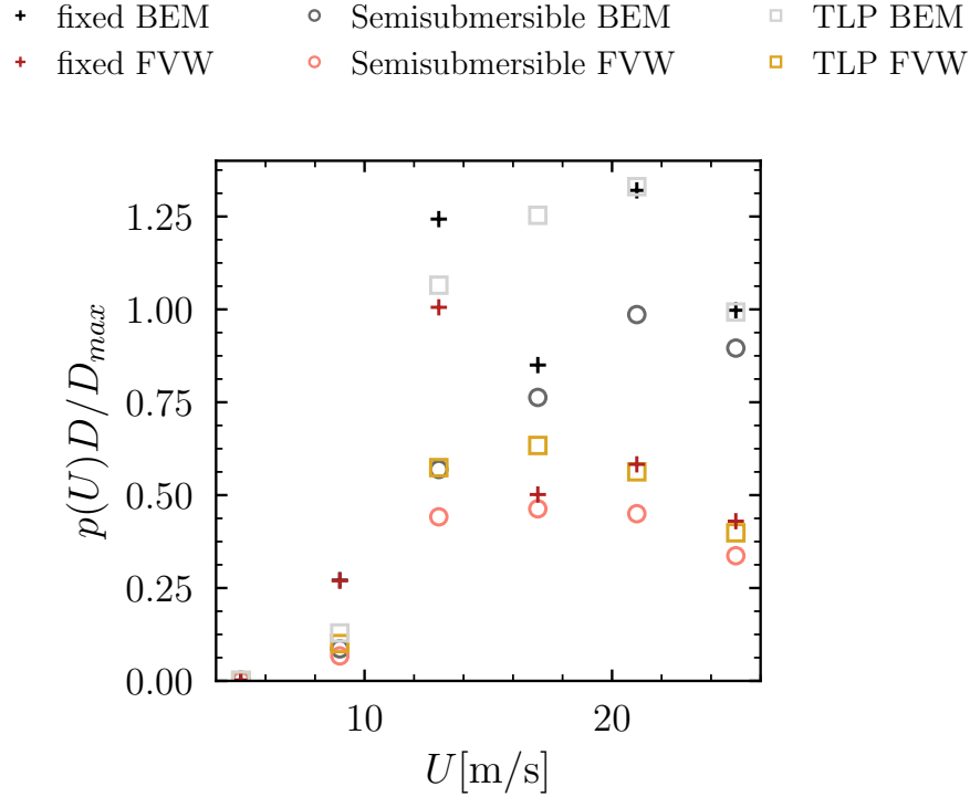
Figure 4.5: Accumulated damage over lifetime taking into account the probability of occurrence of the wind condition. The data is scaled by the maximum damage of one seed obtained with the BEM.
