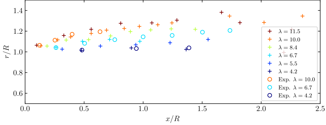
Figure 2.10: Comparison of tip vortex axial and radial positions for different tip speed ratios for the MEXICO wind turbine for experimental results[29] and FVW results of CACTUS.
