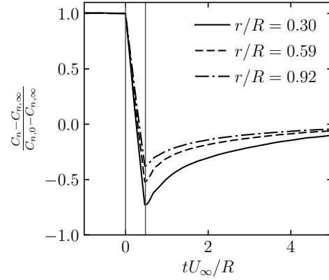
Figure 2.25: Dynamics of the induction factor from FVW for a thrust coefficient decrease due to a ramp of blade pitch. The vertical bars delimit the pitch ramp. Figure 2.26: Normal force coefficient from FVW for a thrust coefficient decrease due to a ramp of blade pitch. The vertical bars delimit the pitch ramp.
