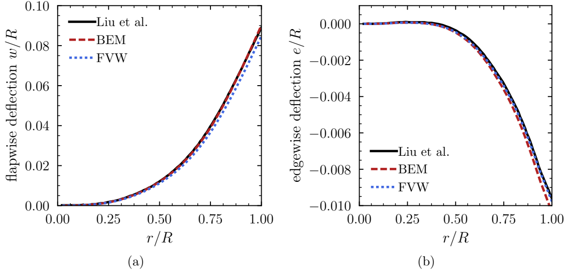
Figure 3.27: Elastic deformations of the blade of the NREL 5MW wind turbine at rated conditions computed with the BEM and FVW of DIEGO compared to numerical blade-resolved CFD data from Liu et al. [111]: (a) flapwise deflection and (b) edgewise deflection.
