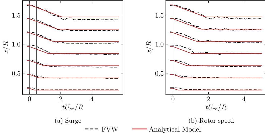
Figure 2.19: Tip vortex positions in the rotating plane defined by the blade and the axial direction from the FVW and analytical models in the thrust coefficient increase case of section 2.3.2.2: (a) surge velocity step; (b) rotor speed step. The vertical lines delimit the applied ramp for the FVW.
