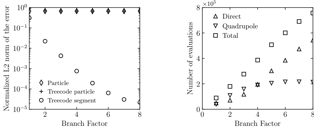
Figure A.5: Normalized L2 norm of the error to the direct calculation for the self-induced velocity. Figure A.6: Number of direct and quadrupole evaluation for the self-induced velocity with the vortex line-based treecode.
