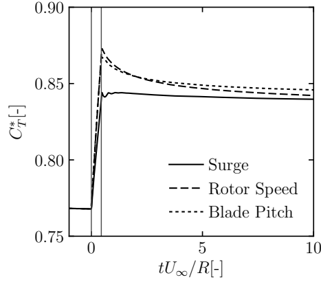
Figure 2.11: Thrust coefficient after a blade pitch, surge, and rotor speed ramp under the conditions listed in Table 2.2 as computed by the FVW model CACTUS for an NREL 5MW reference turbine. The vertical lines delimit the start and end of the applied ramps of duration 0.47R/U_\infty .
