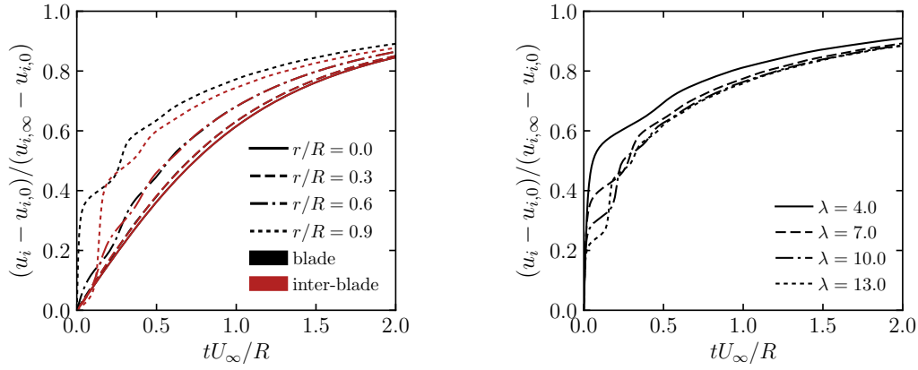
Figure 2.23: Induced velocity at the blade and inter-blade positions for various radial positions. The lines essentially overlap for r/R = 0.0 and 0.3 . u_{i,\infty} is the final converged induced velocity.
