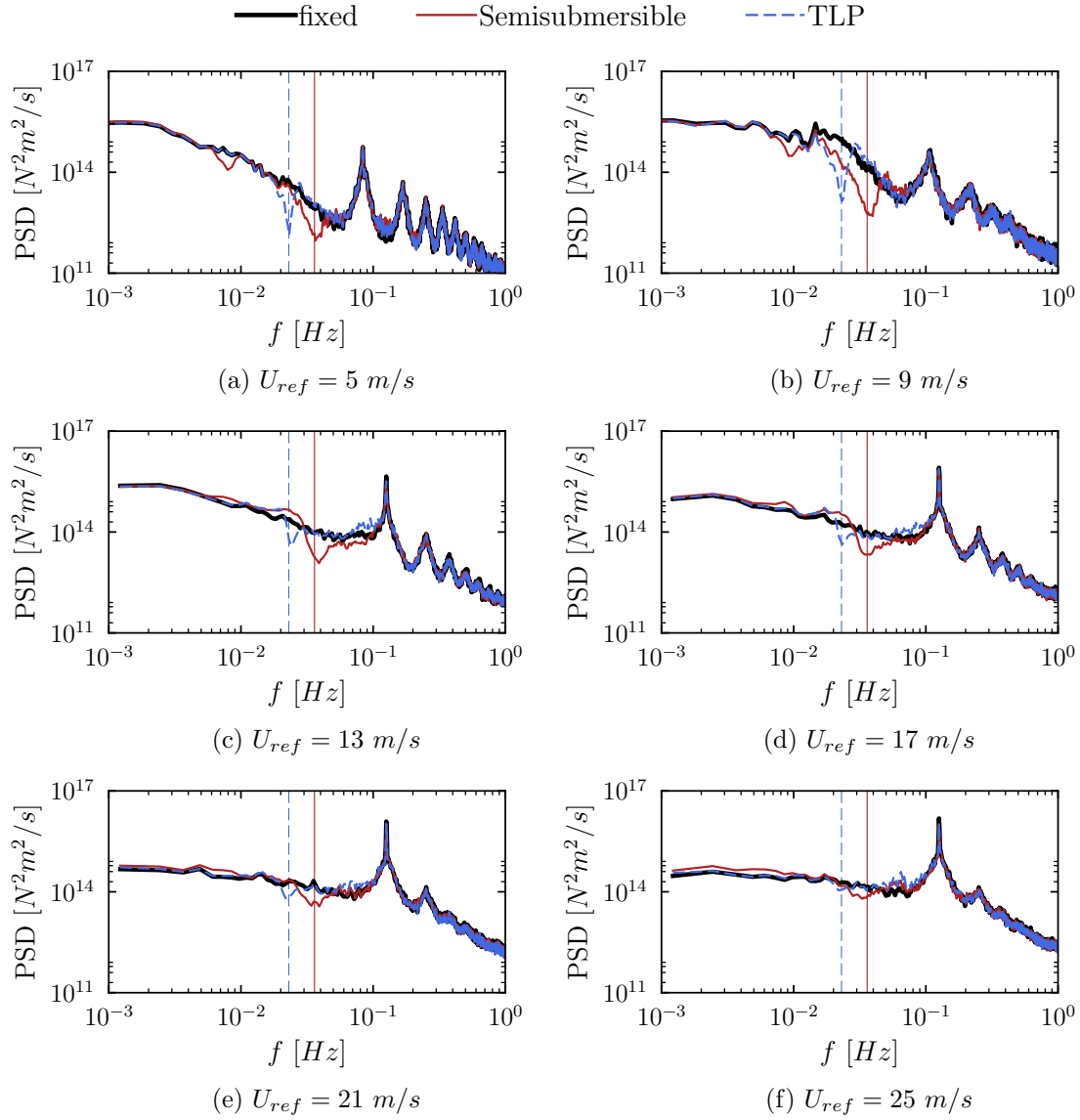
Figure 4.6: Power Spectral Density of the flapwise root bending moment for FVW. The red vertical line shows the natural pitch frequency of the floating wind turbine with the semi-submersible while the blue dashed line shows the natural surge frequency of the floating wind turbine on the TLP.
