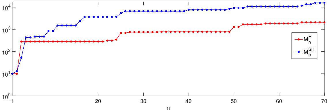
Figure II.7: Evolution of M_n as a function of n for the HMC and SHMC-greedy algorithms.
