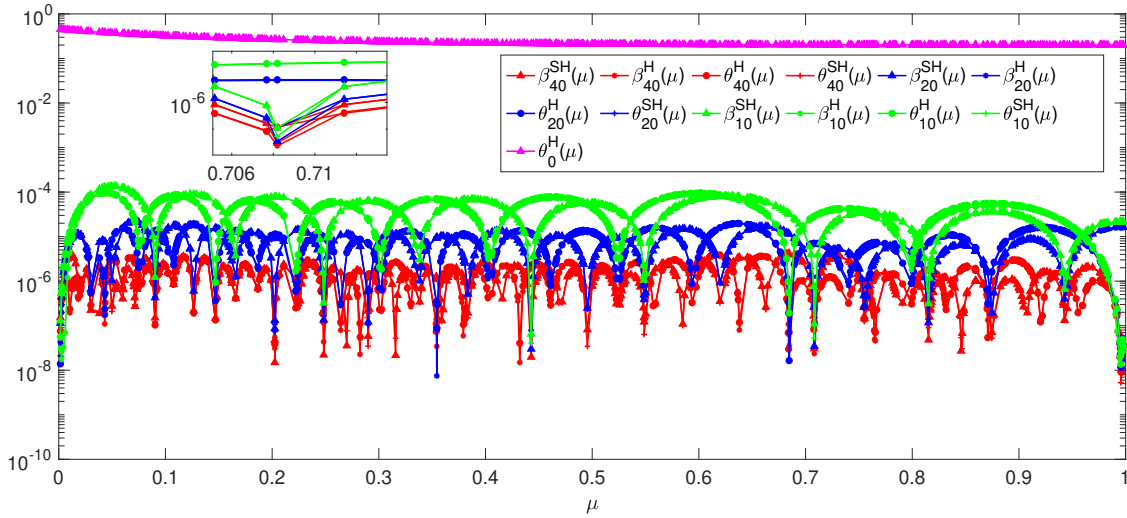
Figure II.10: \theta_n^H(\mu) , \theta_n^{SH}(\mu) , \beta_n^H(\mu) , \beta_n^{SH}(\mu) as a function of \mu for N = 0, 10, 20, 40 on \mathcal{P}_{test} = [0, 1] .
