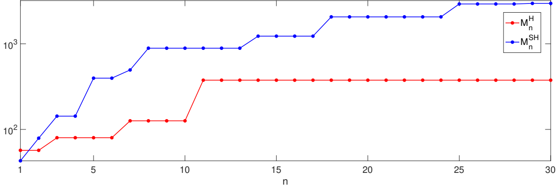
Figure II.1: Evolution of M_n as a function of n for the HMC and SHMC-greedy algorithms in test case 1.
