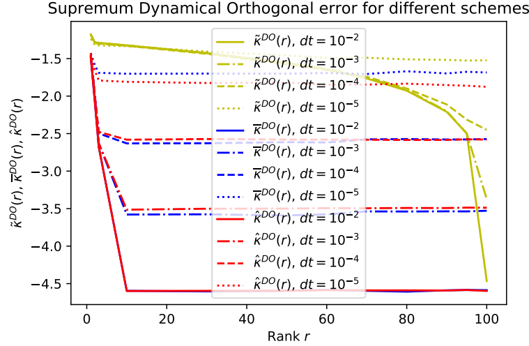
Figure III.10: Convergence of algorithms (9), (10) and (11) for different rank r at different time steps.
