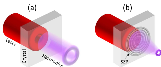
Fig. 1. Sketch of two approaches to create HHG beams carrying an OAM in semiconductor crystals: (a) transfer of the OAM from the driving laser to the harmonics; (b) diffraction of the harmonics by a SZP patterned at the surface of the generation crystal.
