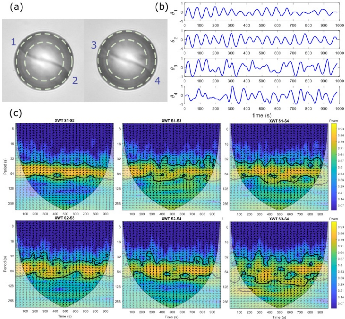
Figure A.1: Dynamics of SRs defects in isolated droplets. (a) Bright-field micrograph of a dimer connected through a disclination line. Dashed circles limit the area analyzed for obtaining the space time plots in (b). Time series in (b) are numbered from 1 to 4 according to the position of the analyzed section. (c) Cross wavelet transform of the time series in (b). The phase lag between the signals is given by the orientation of the black arrows. The dark contour represents a significance level of 5% against noise. The opaque regions correspond to the cone of influence (COI).
