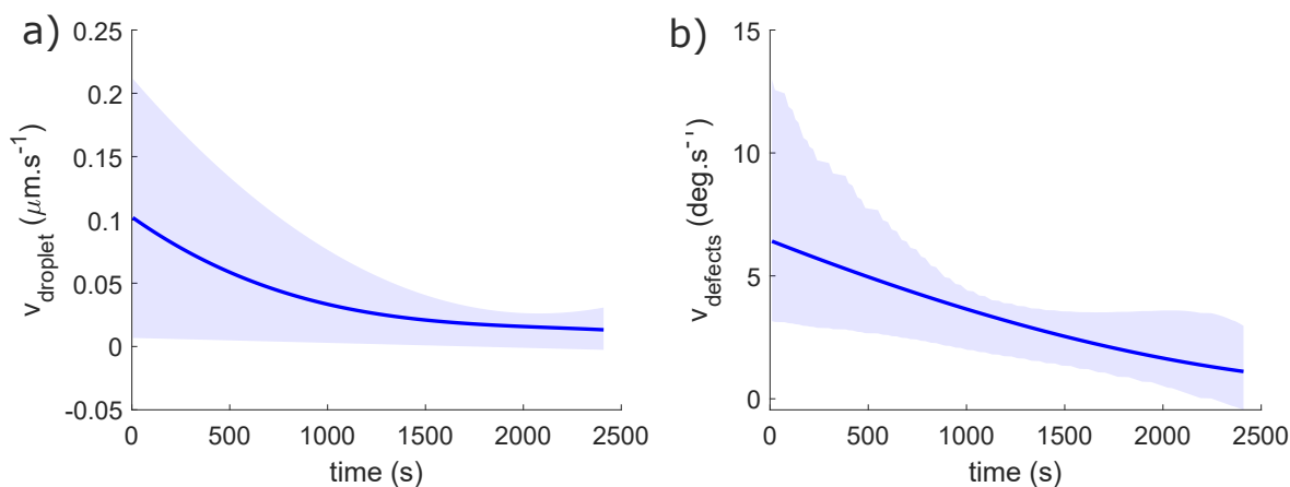
Figure 4.10: Evolution of the (a) droplet speed and (b) defect speed with time. Blue lines corresponds to the polynomial fits of the droplets and defects speeds of a droplet with diameter \sim 50\mu\text{m} . Blue shades represent the data dispersion around the lines.
