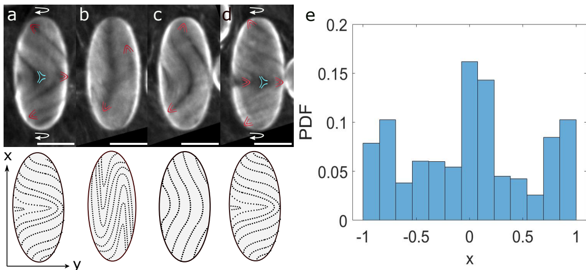
Figure 3.8: Defect dynamics in the transitory, quadrupolar, dynamical state. (a-d) Fluorescence confocal micrographs of active nematics constrained to ellipsoidal surfaces from t = 0 (a) to t = 23 s (d). Parabolic and hyperbolic marks illustrate +1/2 and -1/2 defects, respectively. Sketches in the bottom panel display the director field configuration of the snapshots in the top of the figure. (a), (d) Rotational regime: +1/2 defects spiral by pairs towards the poles while a series of oppositely charged defects circulate around the waist of the ellipsoid. Note that co-rotation at the poles is coupled with counter-rotation at the equator. b) Translational regime: The aligned material destabilizes under extensile stresses, leading to bend distortions which evolve into cracks. Defects propagate longitudinally along the cracks exchanging from one pole to the other. The two regimes repeat periodically for over two hours. (e) Normalized probability distribution of defects along the main axis of the ellipsoid in the transient dynamical state.
