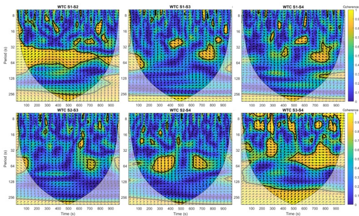
Figure A.2: Wavelet coherence spectra of signals Fig. A.1 (b) The phase lag between the signals is given by the orientation of the black arrows. The dark contour represents a significance level of 5% against noise. The opaque regions correspond to the cone of influence (COI)
