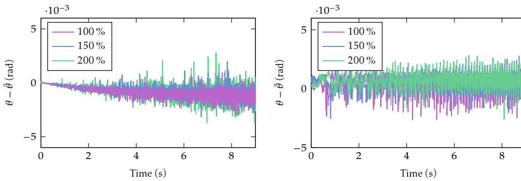
(c) Error \theta - \hat{\theta} (rad) at 100% (purple), 150% (blue) and 200% (green) of rated torque.
