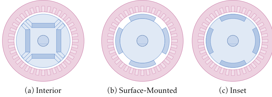
Figure 1.1: Different PMSM rotor structures along with distributed stator windings
