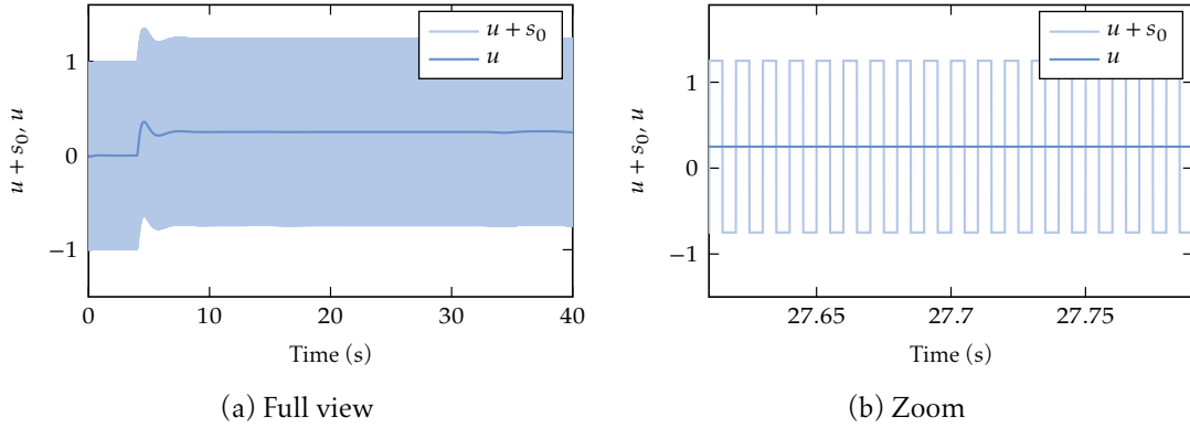
Figure 2.1: Control inputs u and u + s_0 . Full view (left), zoom (right).
