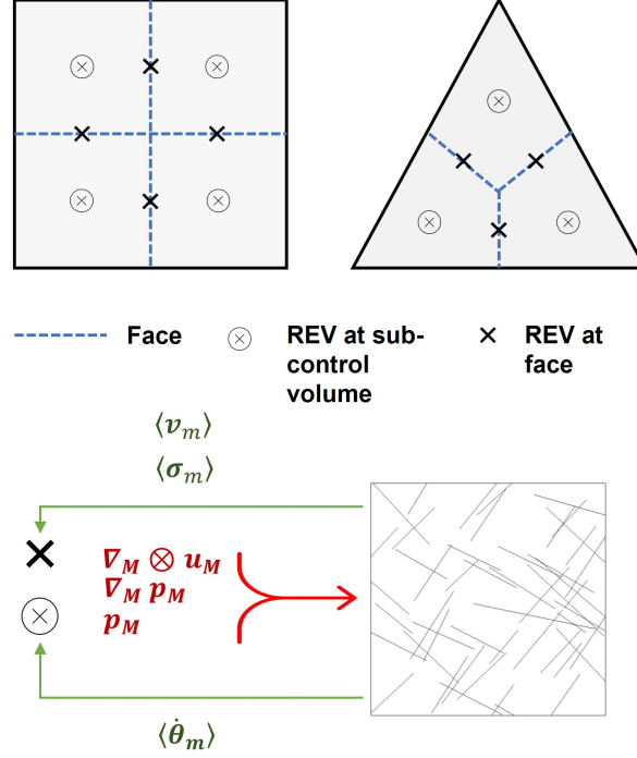
Figure 6.1: Location of the REV in the multi-level Box method: each center of a face and of a SCV contains a REV. The REV receives the interpolated pressures and gradients at these locations, and sends homogenized fluxes and stresses to the faces and the homogenized storage term to the SCV.
