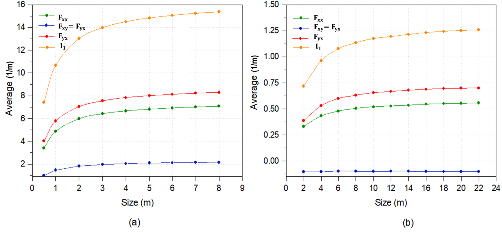
Figure 5.5: Average values of the fracture tensor components for (a) Network 1 and (b) Network 2.
