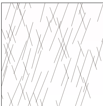
Figure 7.1: Example of one of the generated DFNs that replicate the pattern of the tectonic fractures in the Ekofisk reservoir. There is a main sub-vertical set of larger fractures, which are sometimes associated to conjugate smaller fractures.
