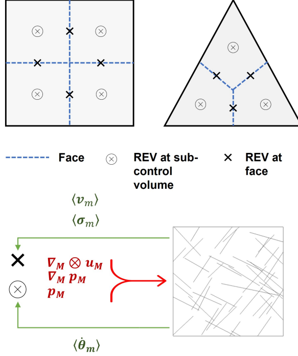
Figure 6.1: Location of the REV in the multi-level Box method: each center of a face and of a SCV contains a REV. The REV receives the interpolated pressures and gradients at these locations, and sends homogenized fluxes and stresses to the faces and the homogenized storage term to the SCV.
