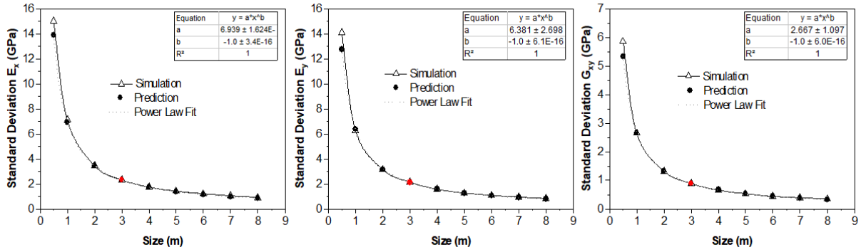
Figure 5.15: Predicted and calculated curves of the standard deviation of the elastic moduli of Network 2 vs REV size. The red dot signalizes the reference volume.
